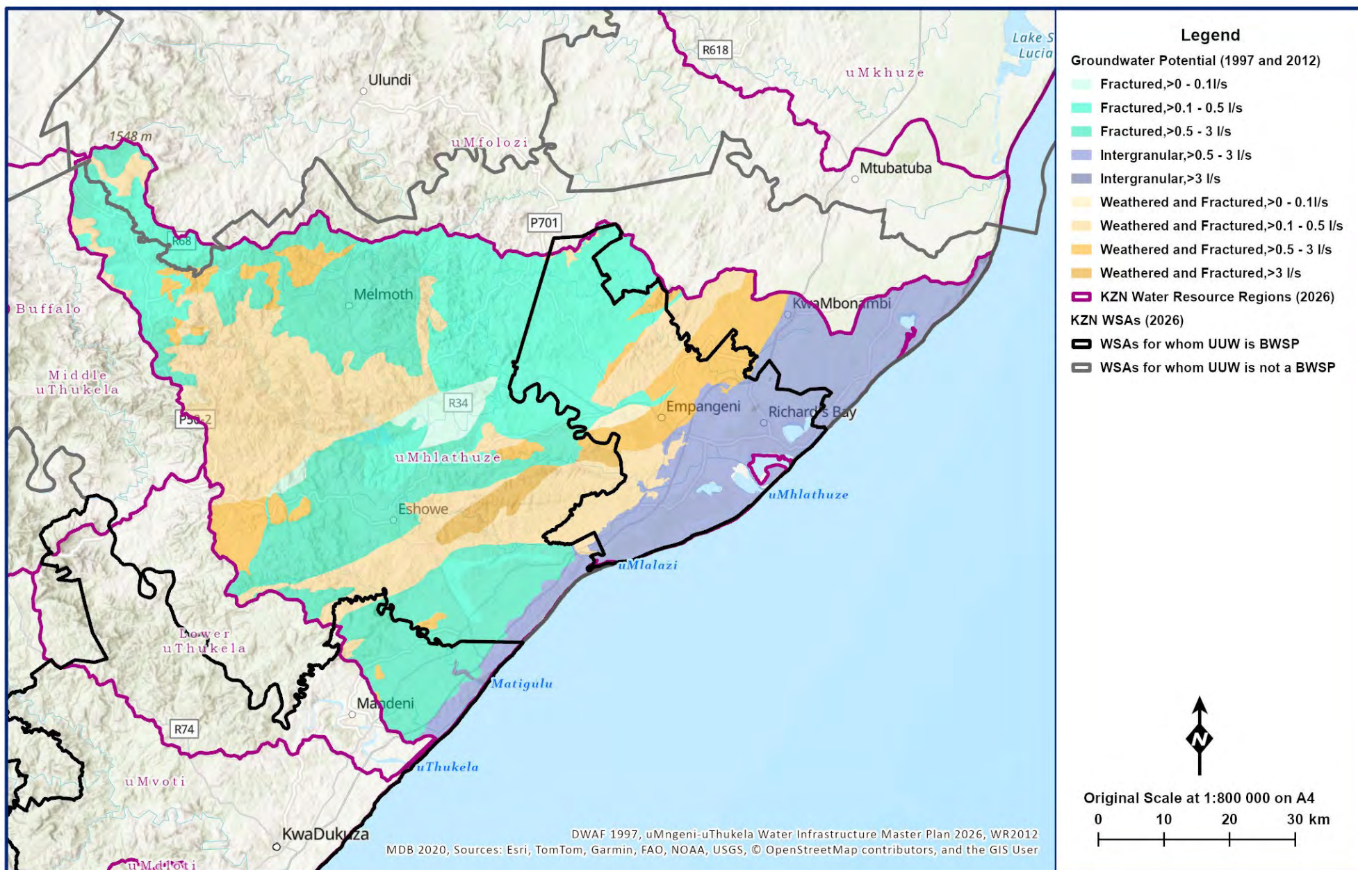
Figure 16.3 Groundwater potential in the uMhlathuze Region.
