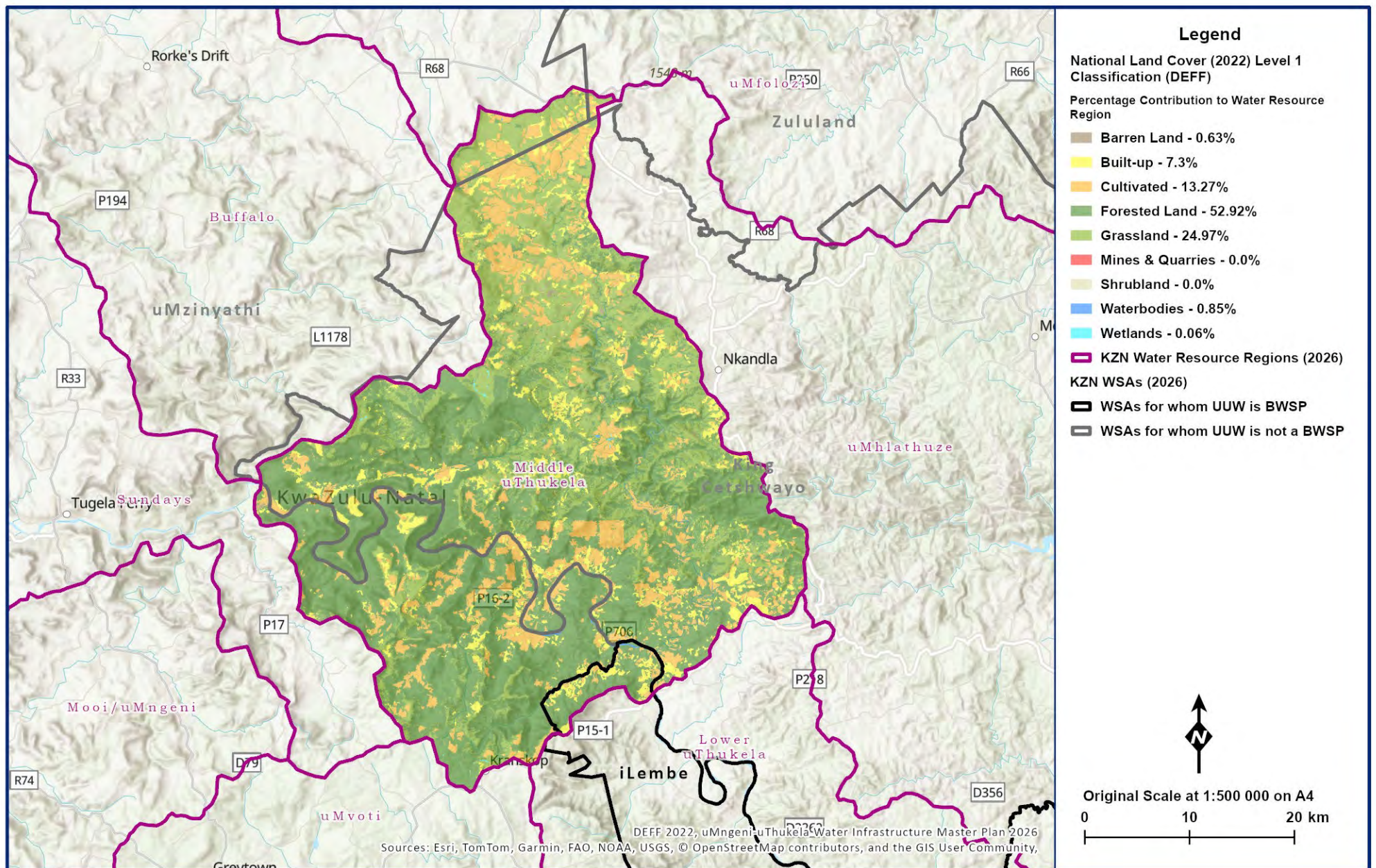
Figure 15.2 Middle uThukela land cover.
