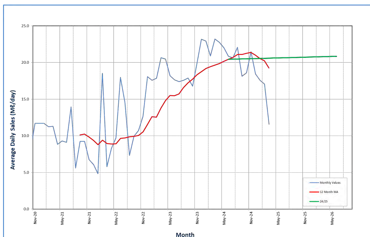
Figure 16.34 Water demand for Greater Mthonjaneni WTP
