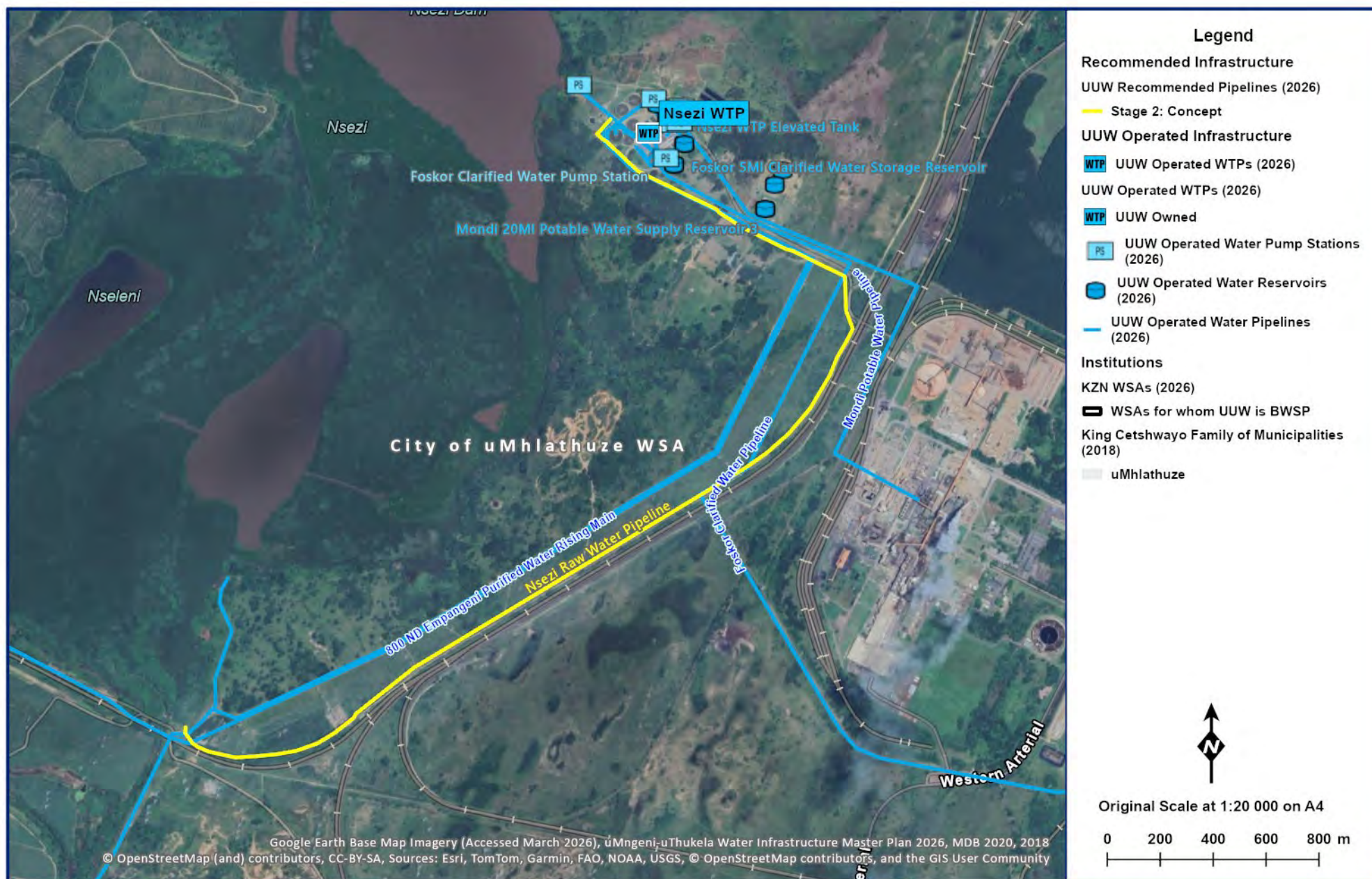
Figure 16.44 Nsezi Raw Water Pipeline.
