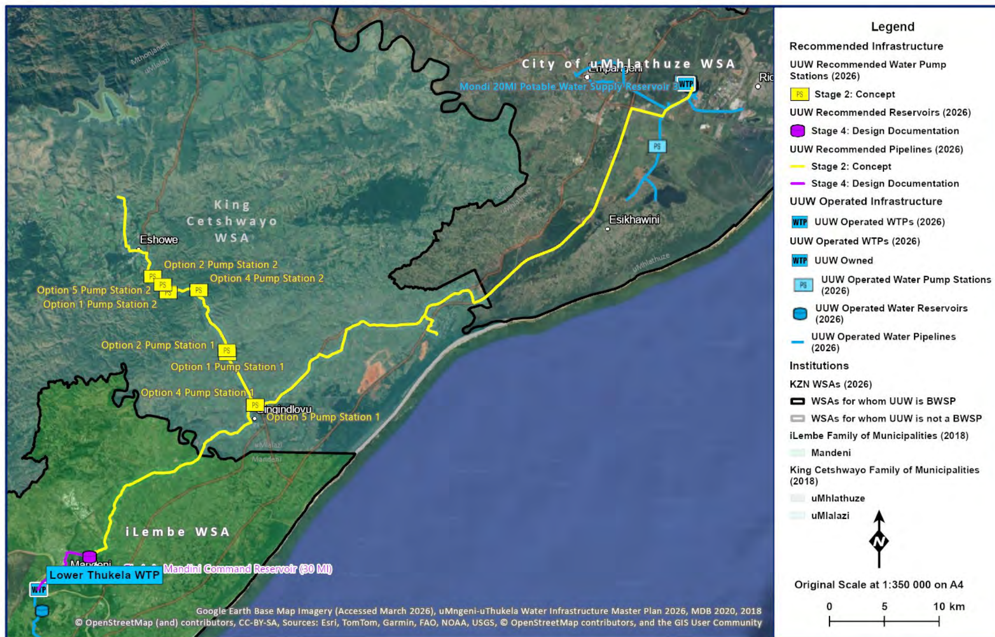
Figure 16.41 General layout of Lower Thukela Bulk Water Supply Scheme Phase 3.
