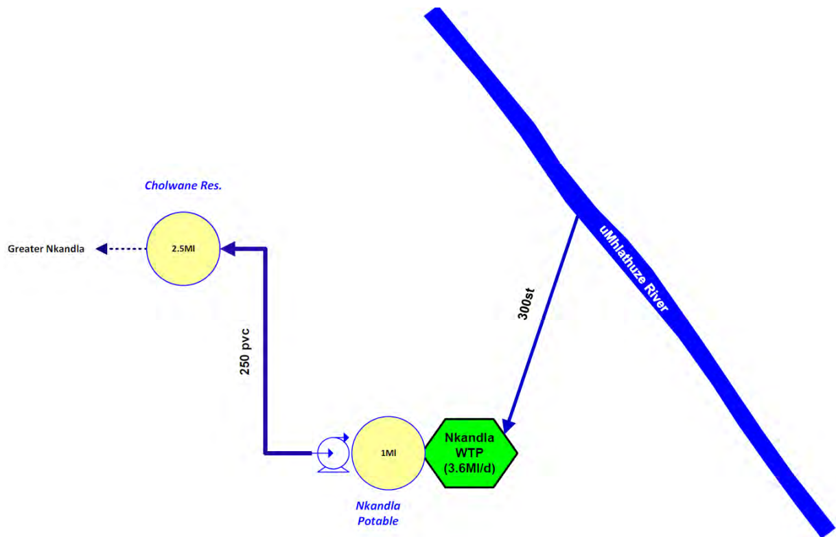
Figure 16.12 Schematic of Nkandla WTP Supply System
