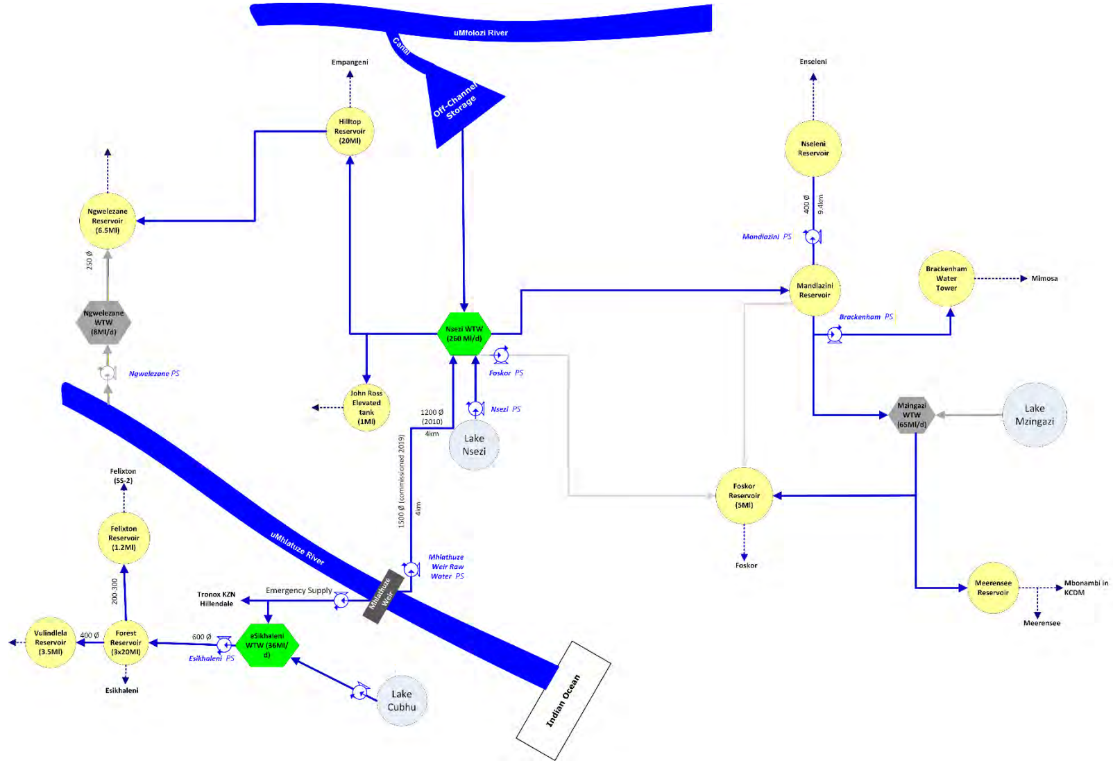
Figure 16.40 Future Bulk Scenario for CoU
