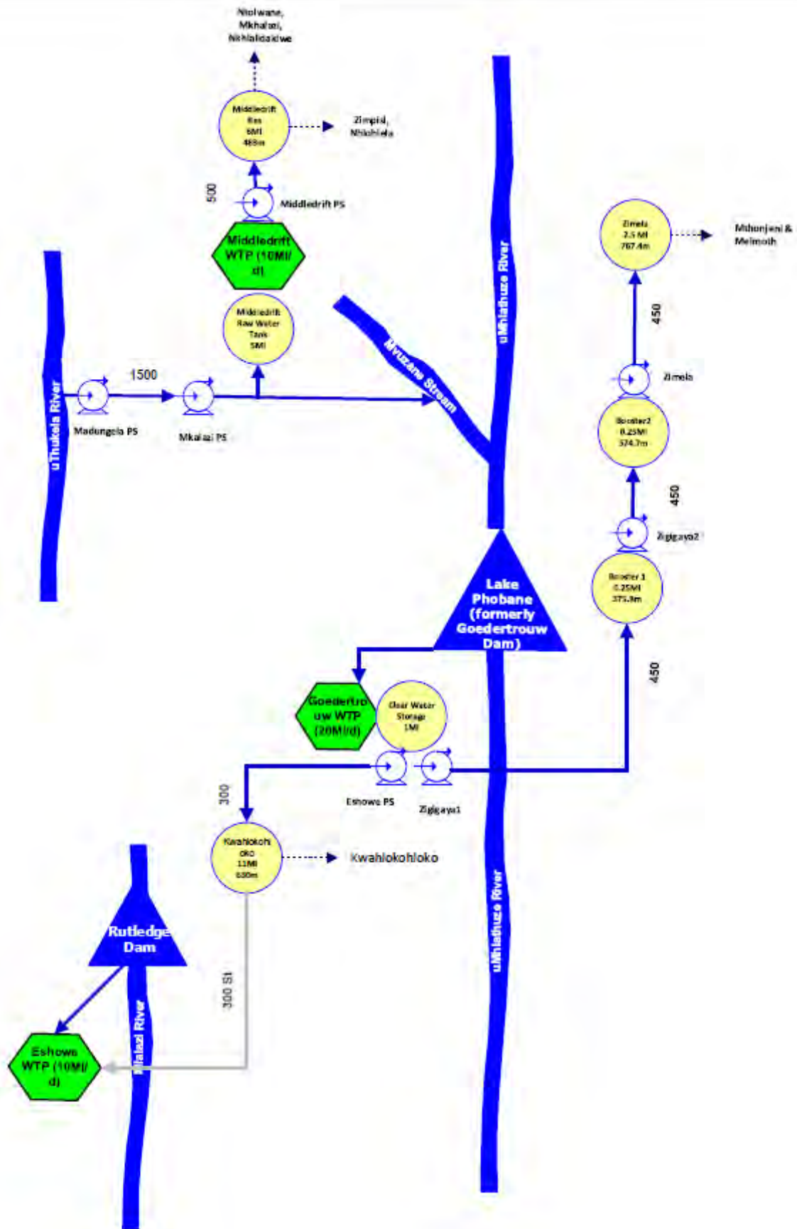
Figure 16.18 A schematic of Central uMhlathuze System.
