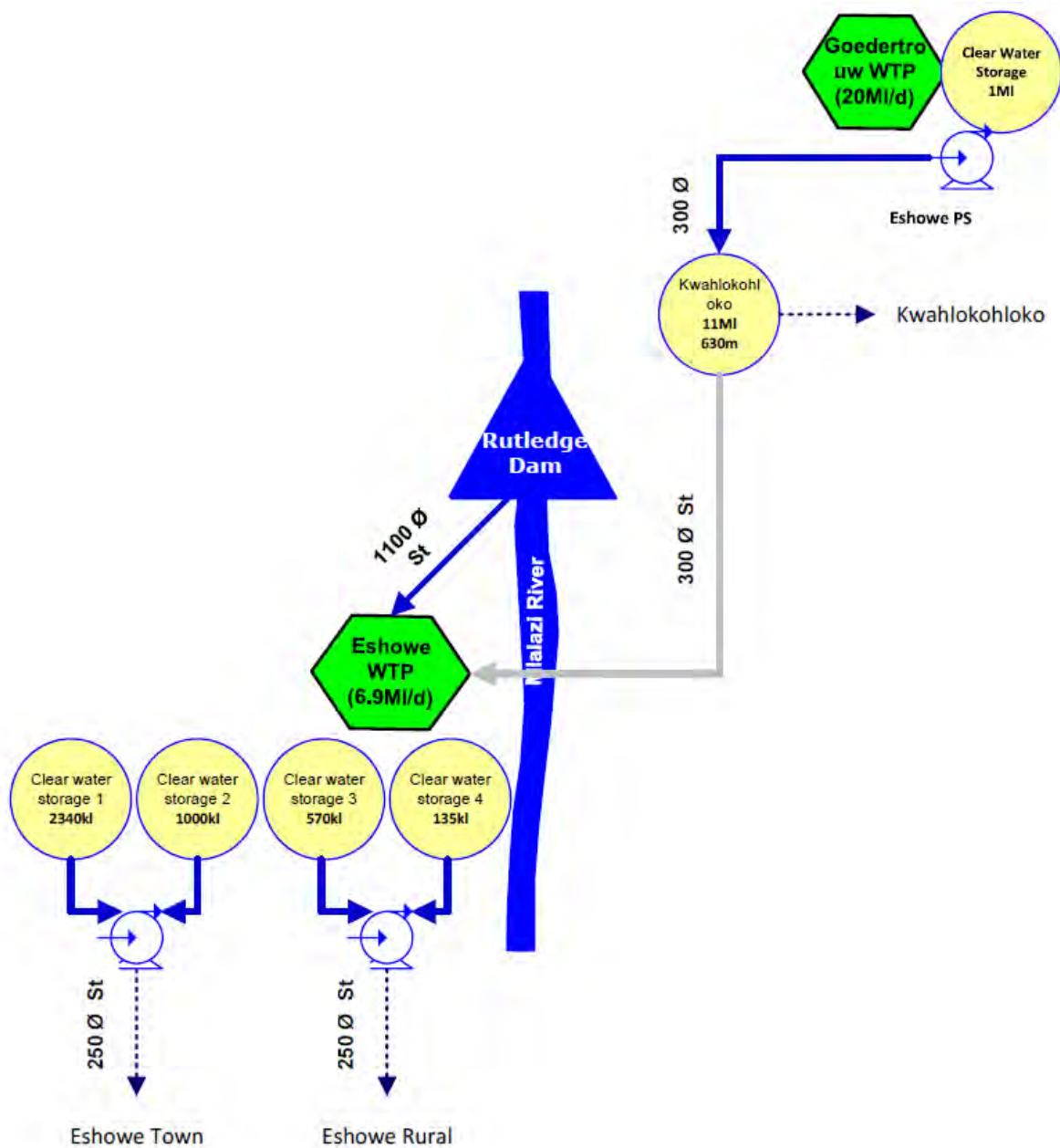
Figure 16.22 Schematic of Eshowe System.
