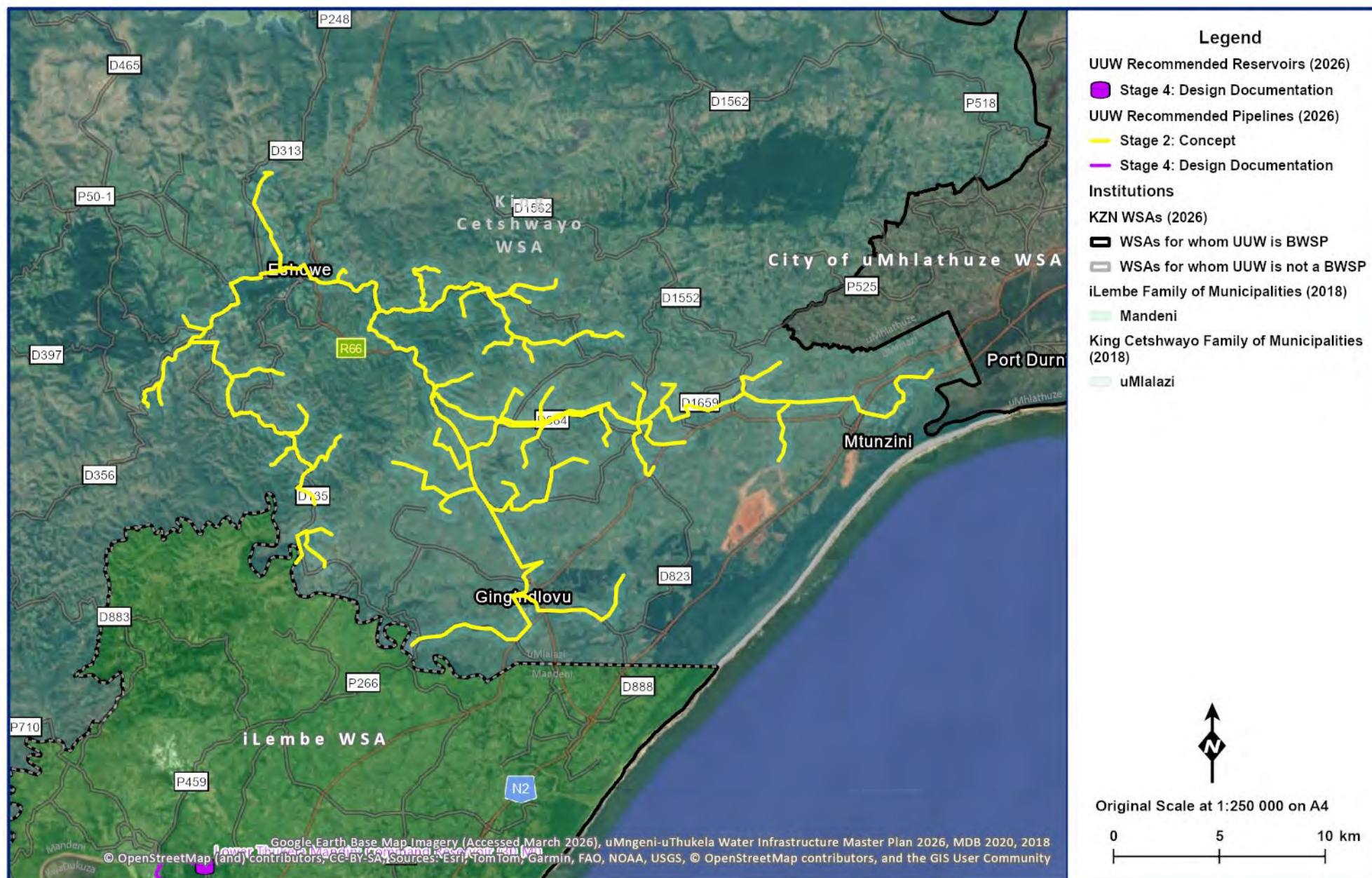
Figure 16.42 General layout of the Eshowe Bulk Water Supply Scheme.
