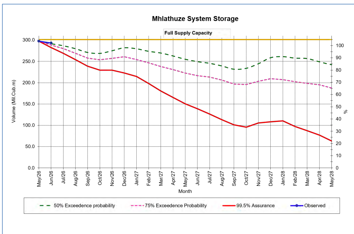
Figure 16.8 Storage trajectories for the uMhlathuze system based on a May 2026 decision date.
