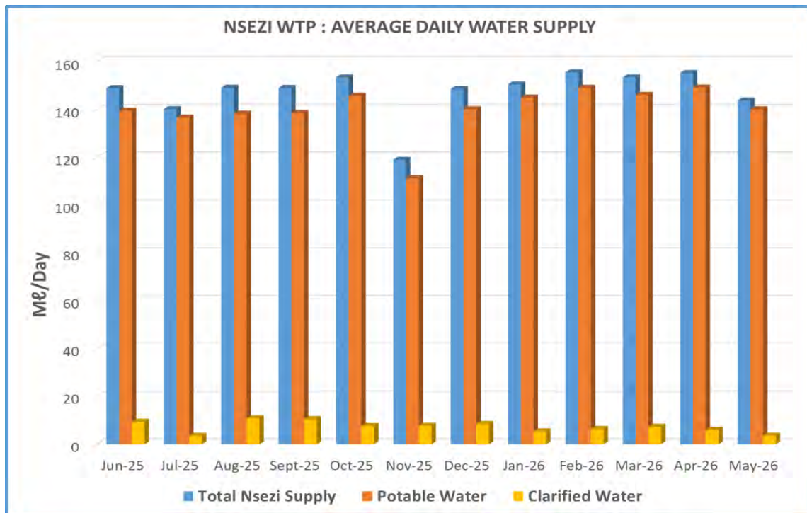
Figure 16.37 Average Water Supply from Nsezi WTP (till end May 2026)
