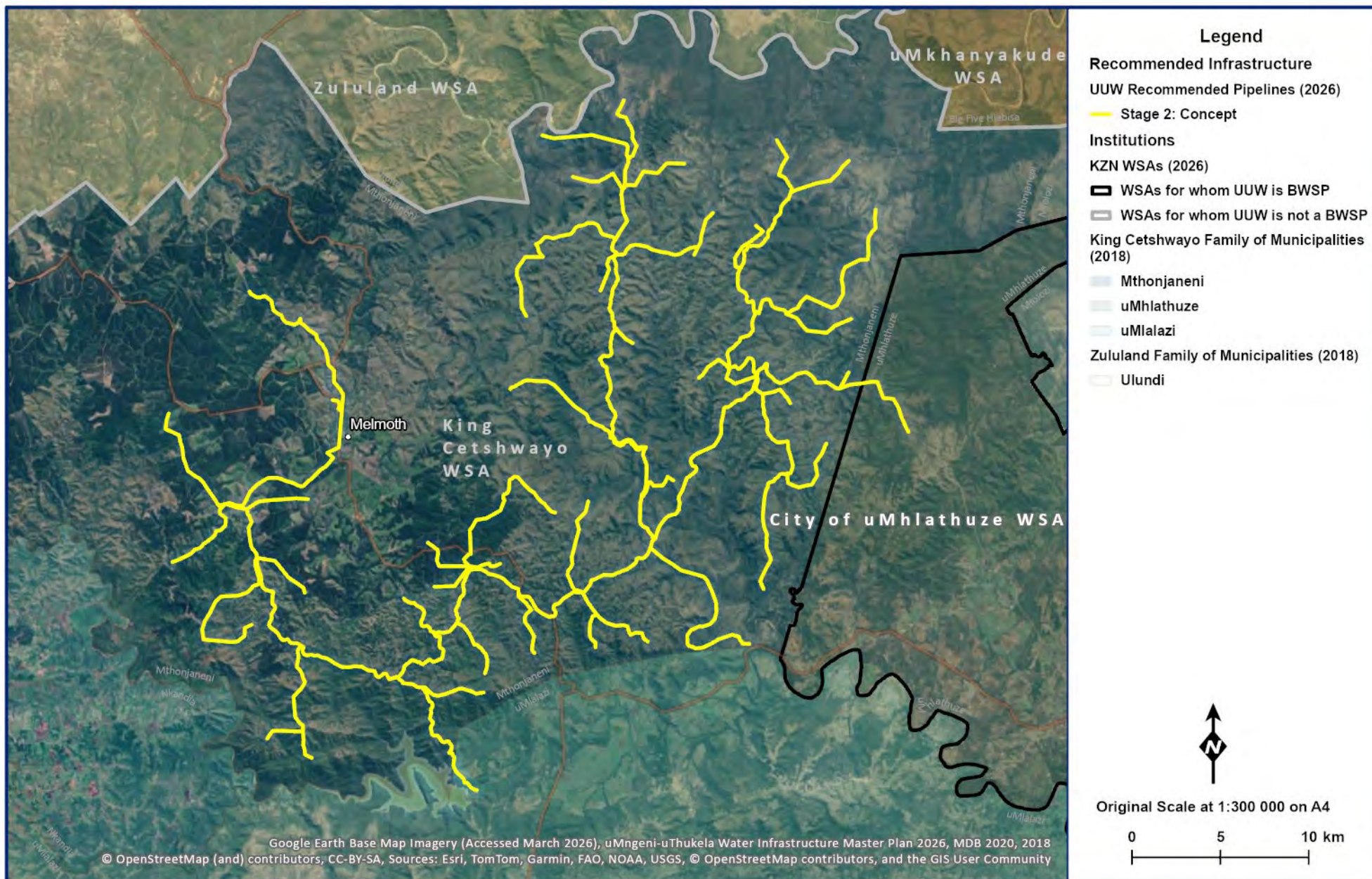
Figure 16.43 General layout of the Mthonjaneni Bulk Water Supply Scheme.
