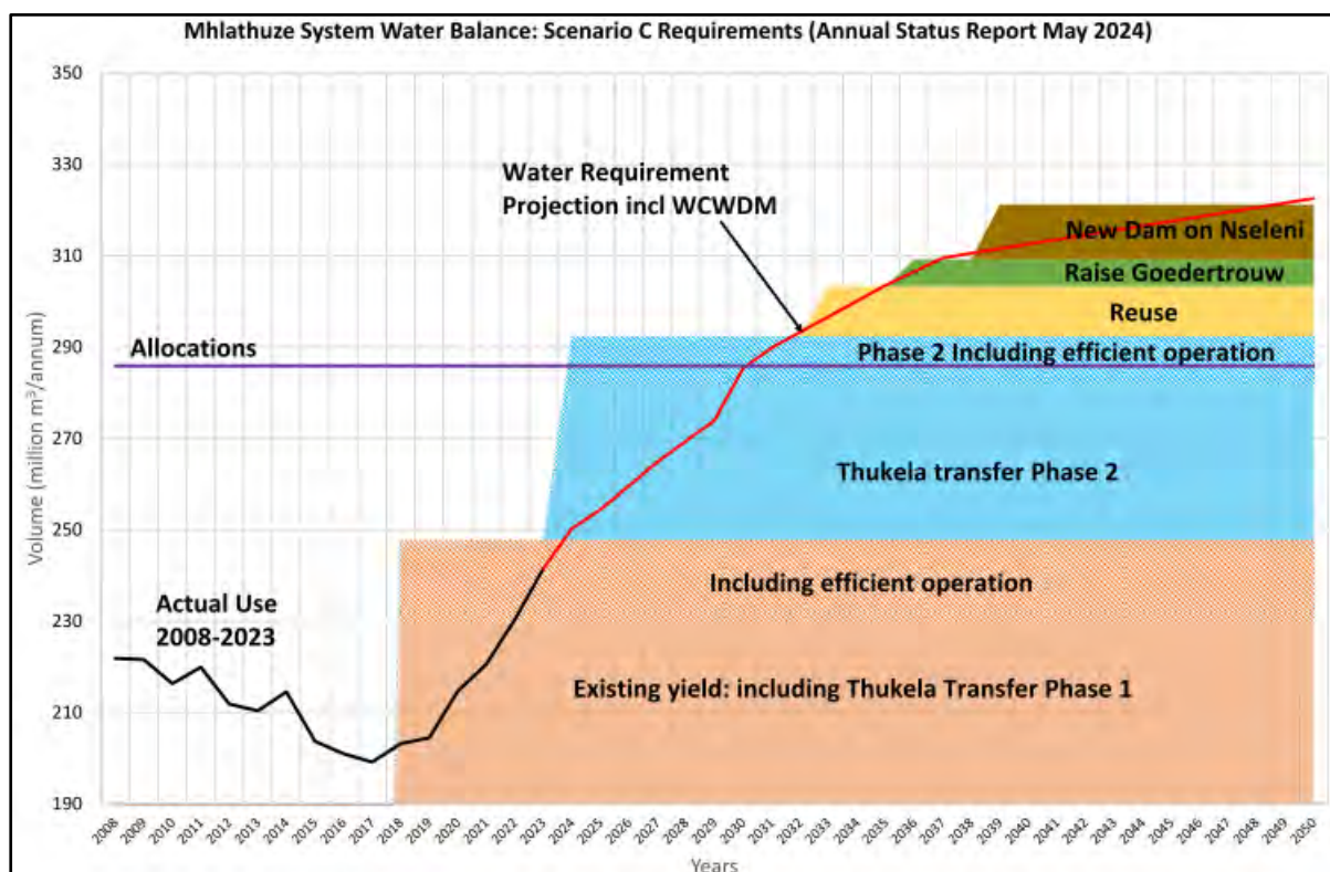
Figure 16.39 uMhlathuze System Balance for a moderate growth scenario.
