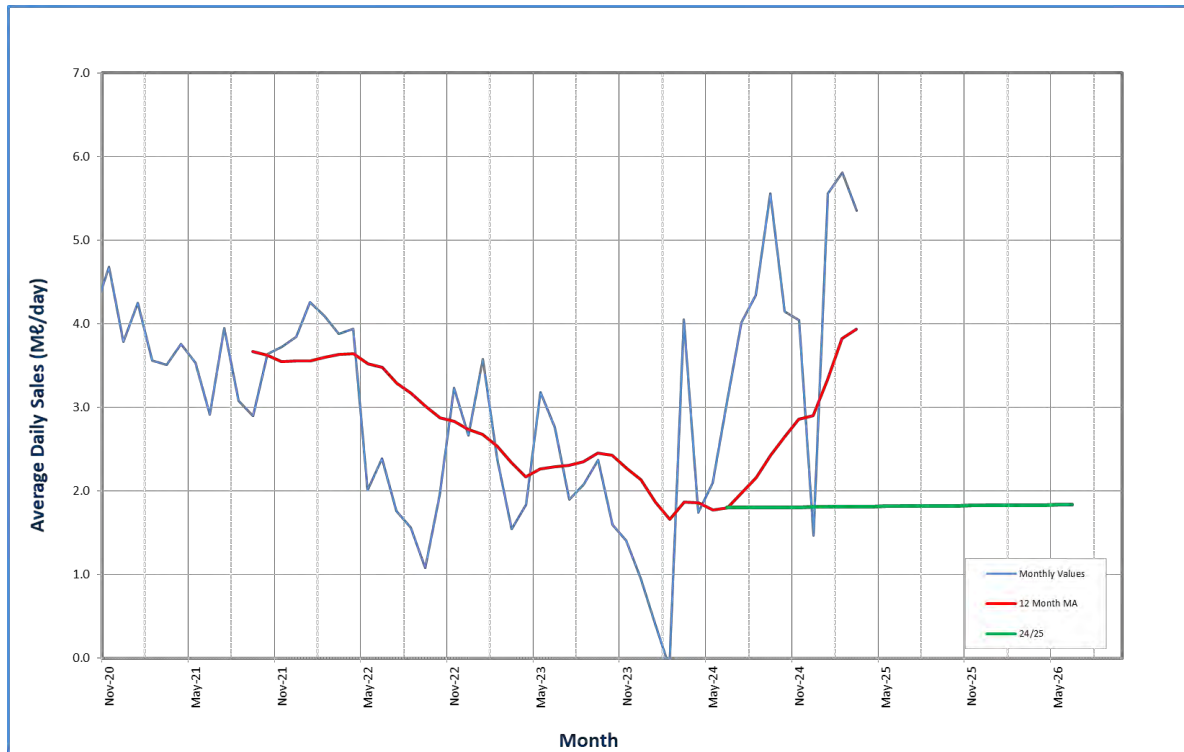
Figure 16.35 Water demand for Eshowe WTP
