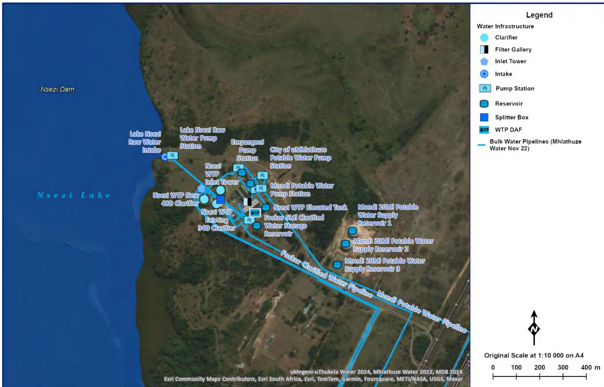
Figure 16.29 Nsezi WTP
