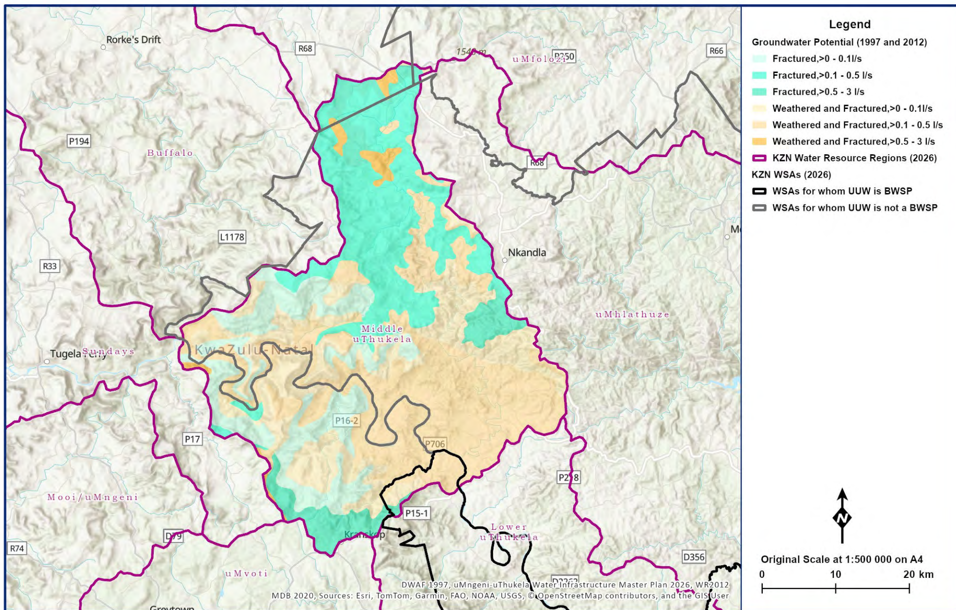
Figure 15.3 Groundwater potential in the Middle Thukela Region.
