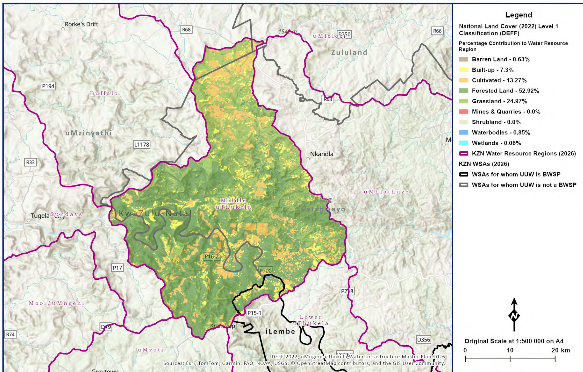
Figure 15.2 Middle uThukela land cover.
