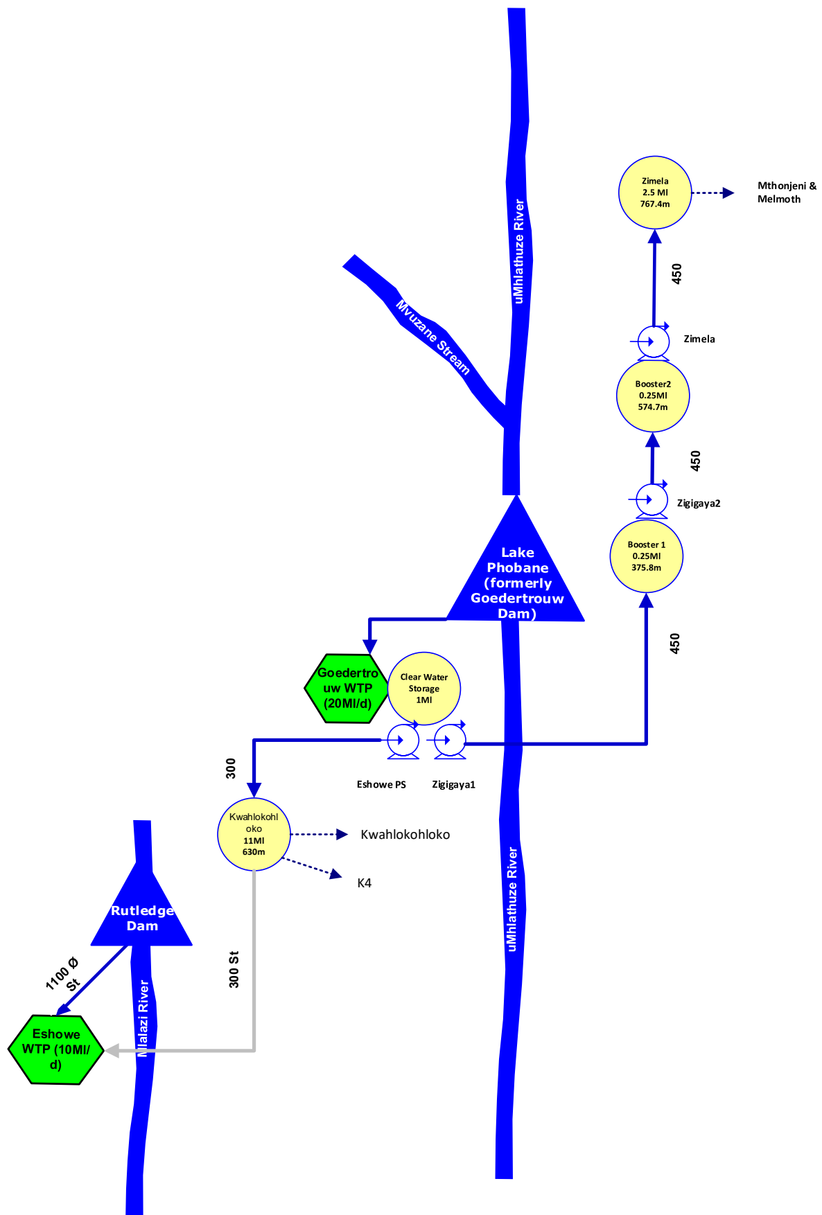
Figure 16.20 Schematic of Goedertrouw Supply System.
