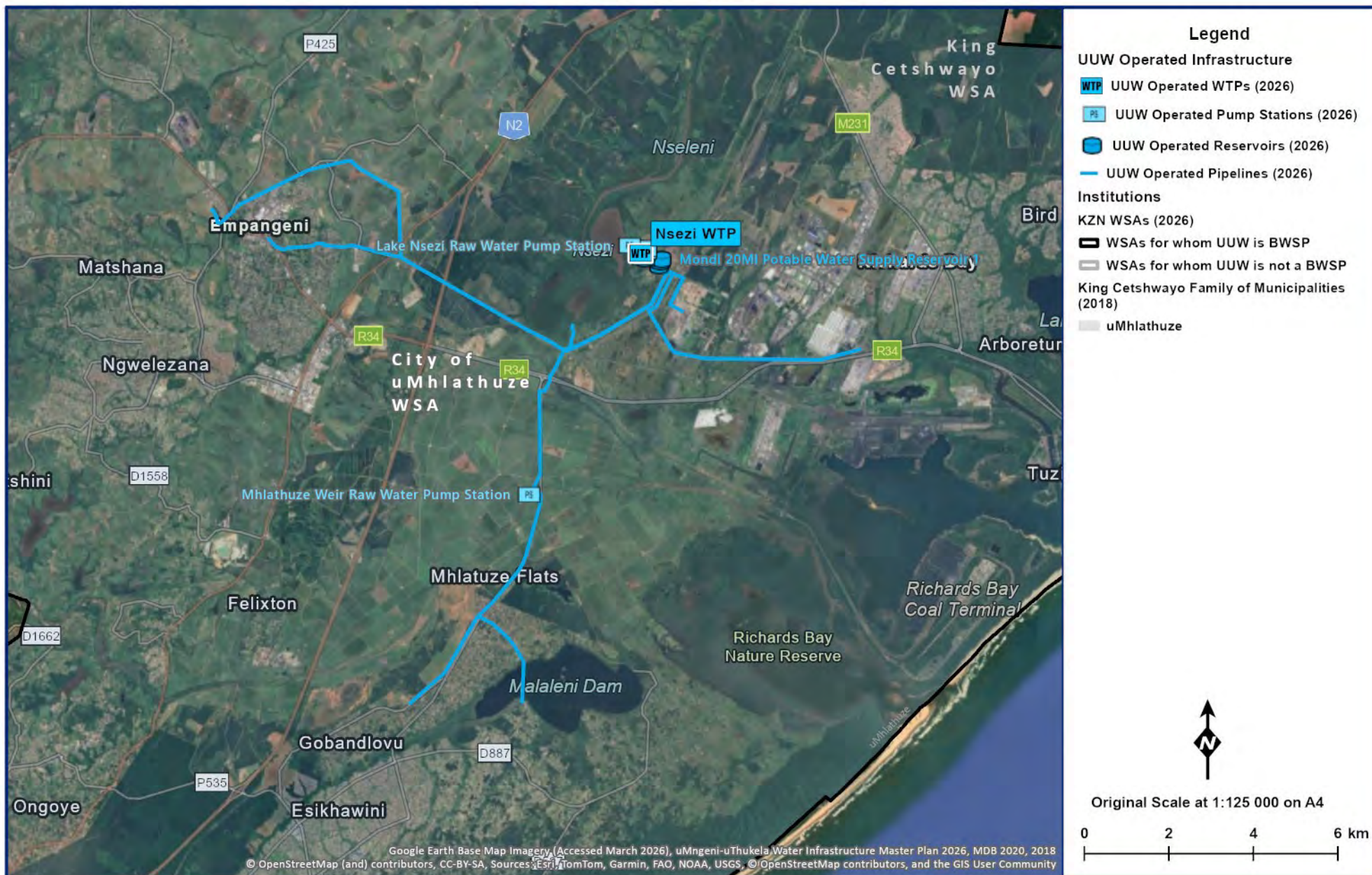
Figure 16.28 Mhlathuze Weir to Nsezi WTP.
