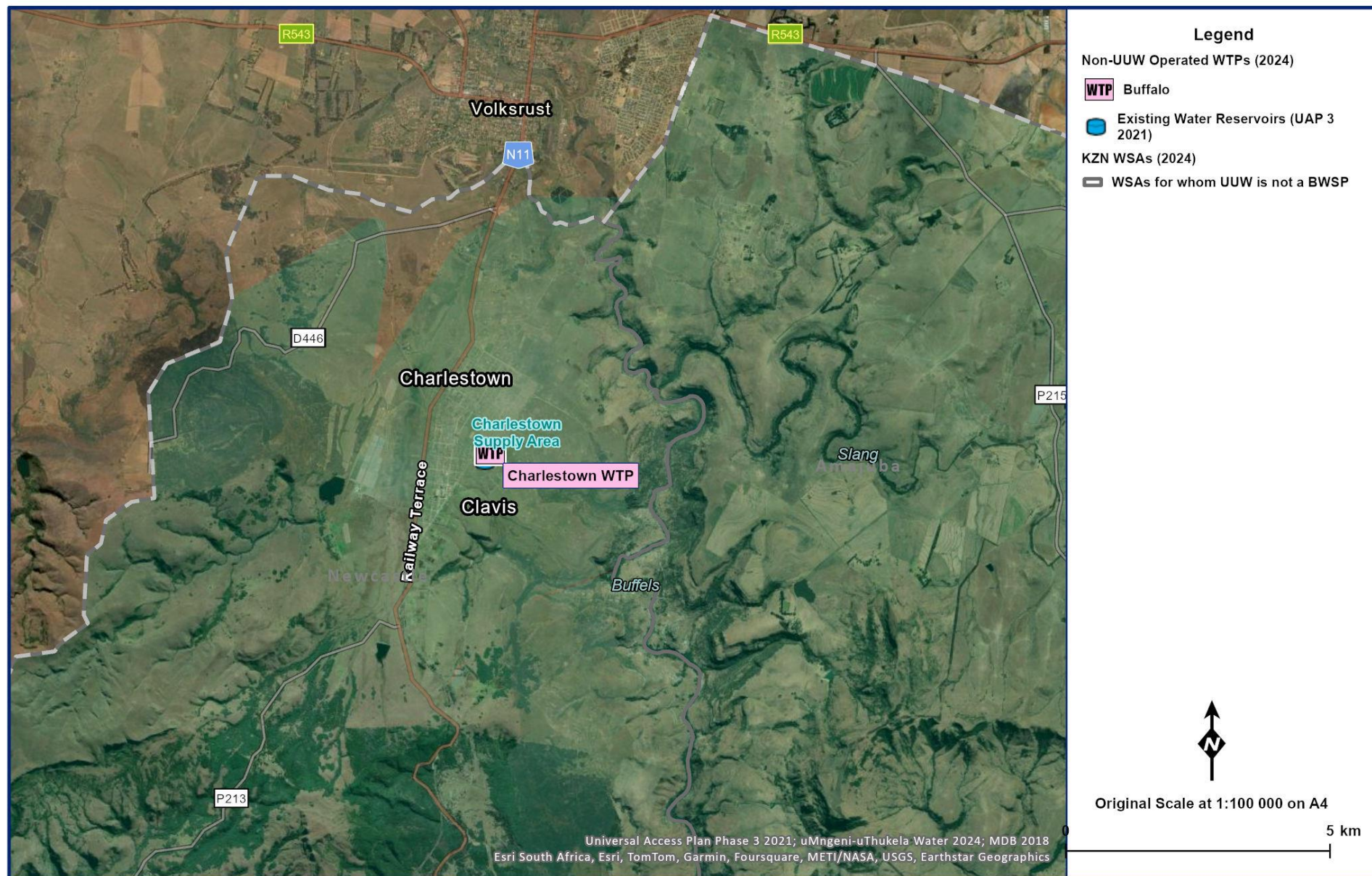
Figure 14.45 Charlestown Supply System Layout (Charlestown WTP System) (NGI 2014; Umgeni Water 2020)
