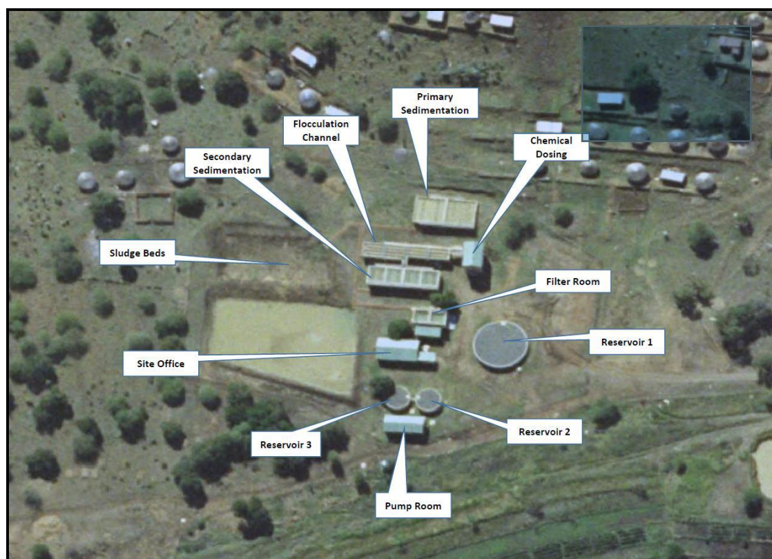
Figure 13.70 Overview of Tugela Ferry WTP, uMzinyathi DM O&M Manual (December 2016)
