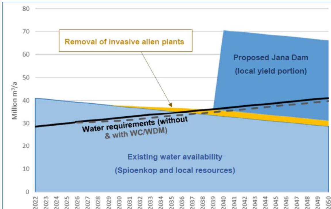
Figure 13.73 Water balance for the Upper Thukela Supply system (DWS 2024).
