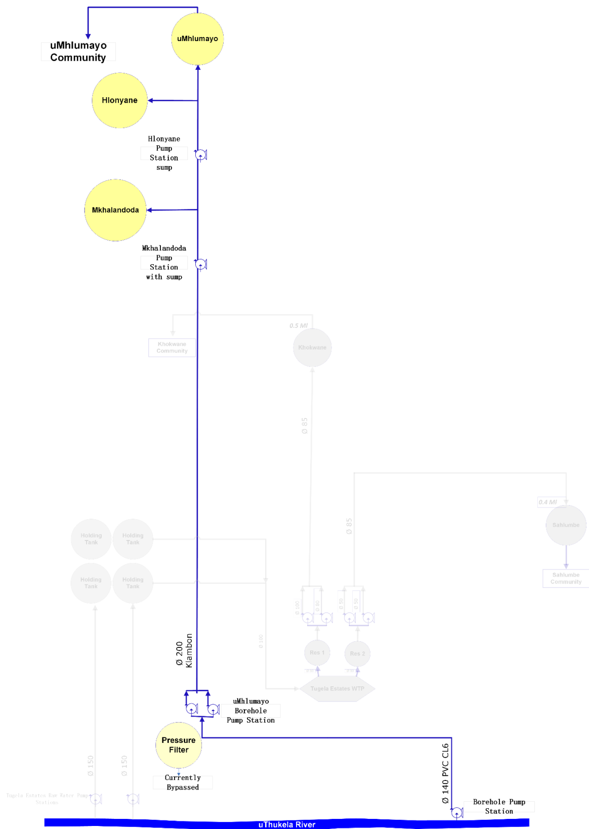
Figure 13.37 uMhlumayo Borehole Supply System schematic.
