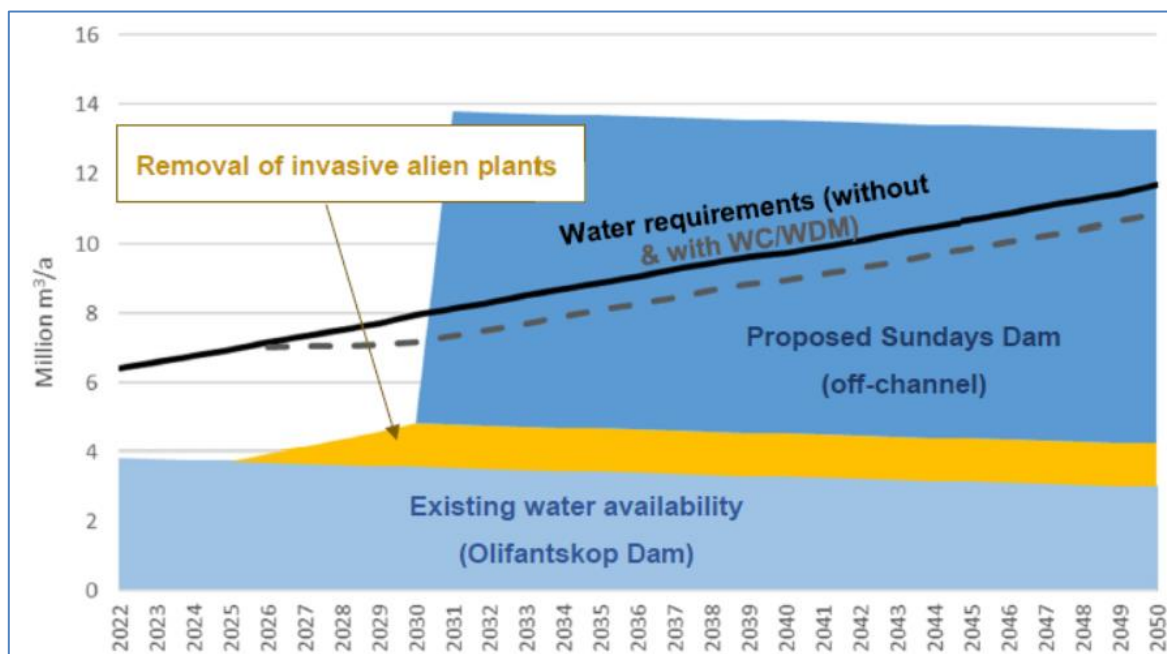
Figure 13.74 Water balance for the Sundays System (DWS 2024).
