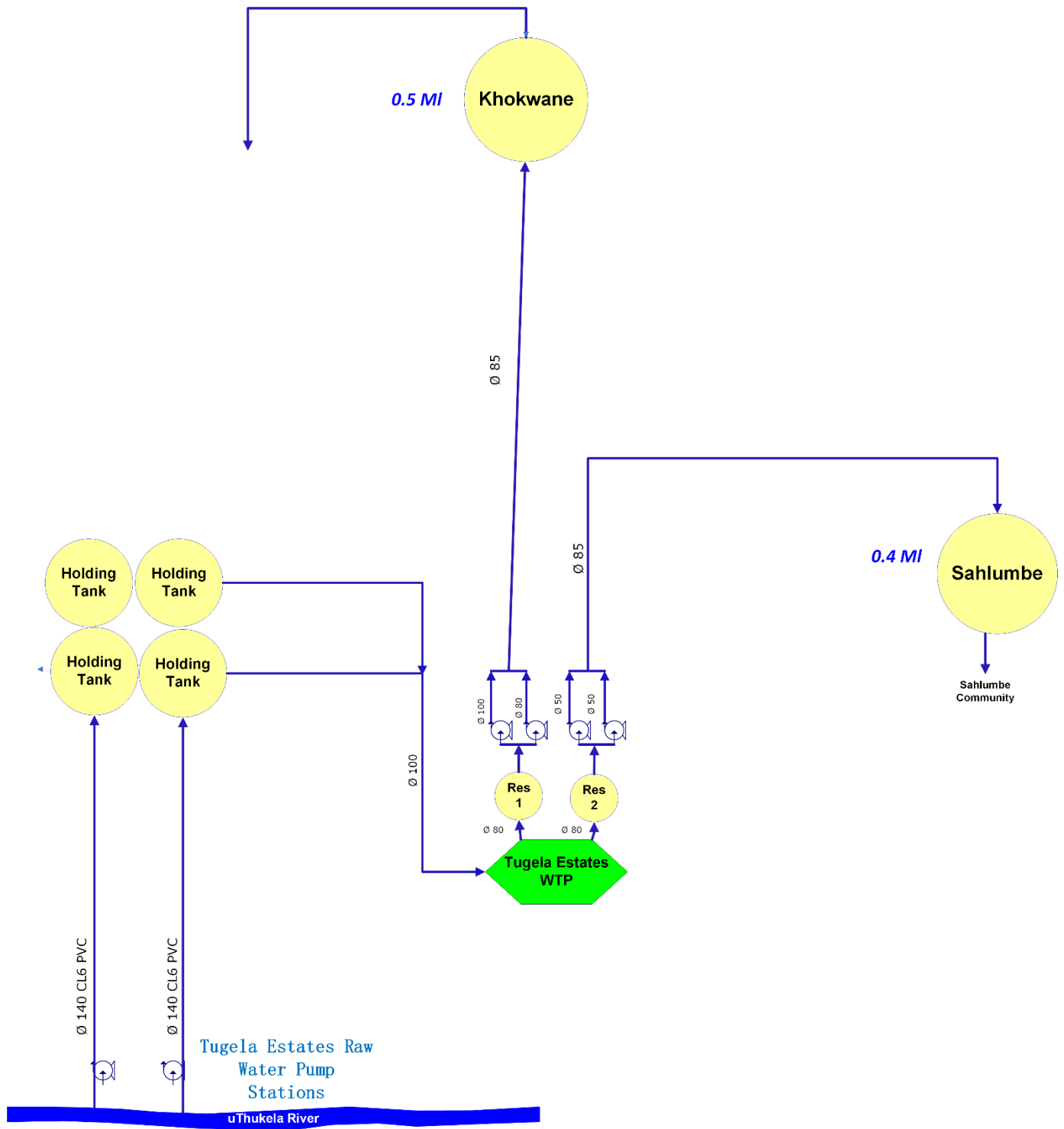
Figure 13.36 Tugela Estates WTP Supply System schematic.
