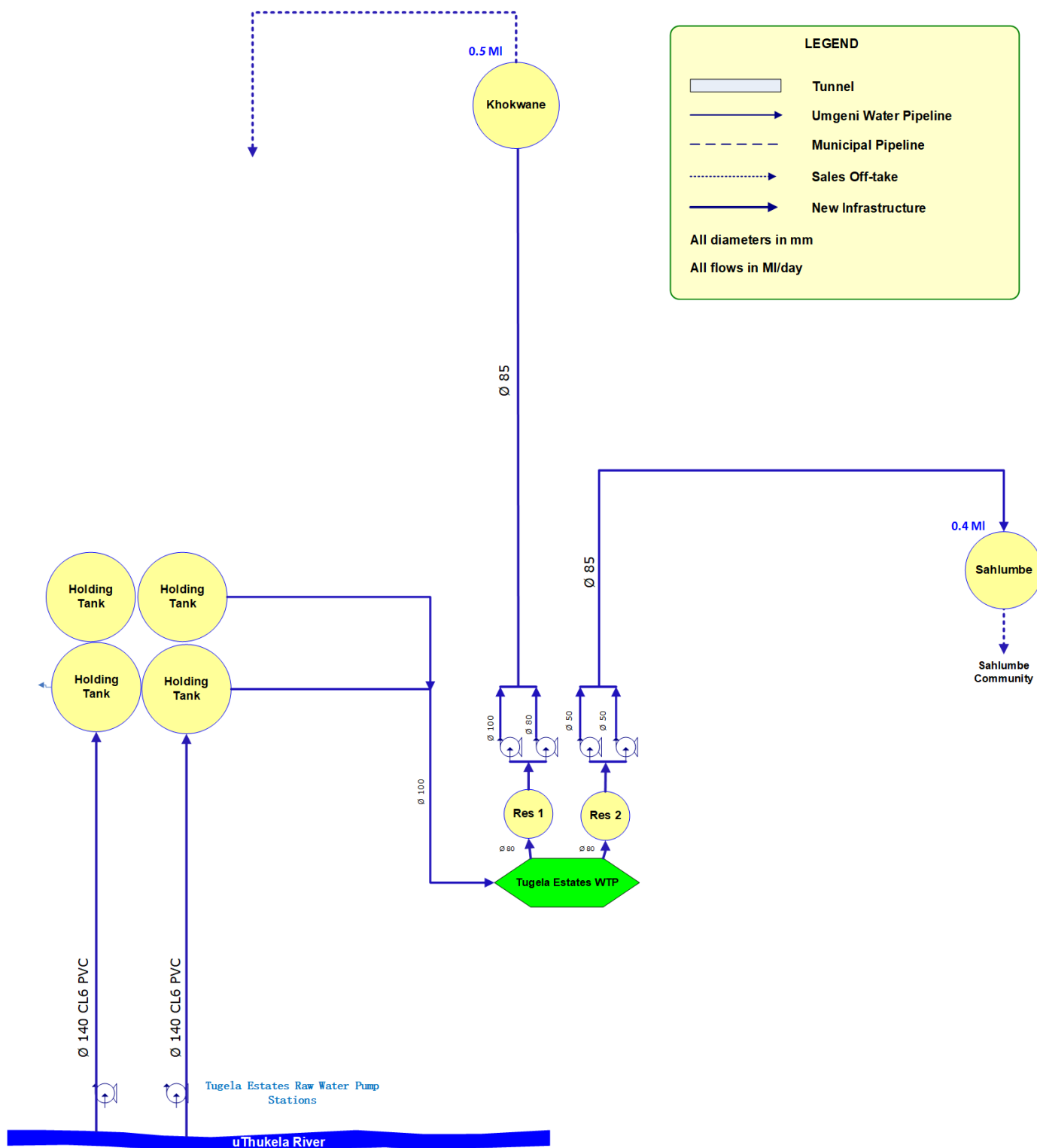
Figure 13.36 Tugela Estates WTP Supply System schematic.
