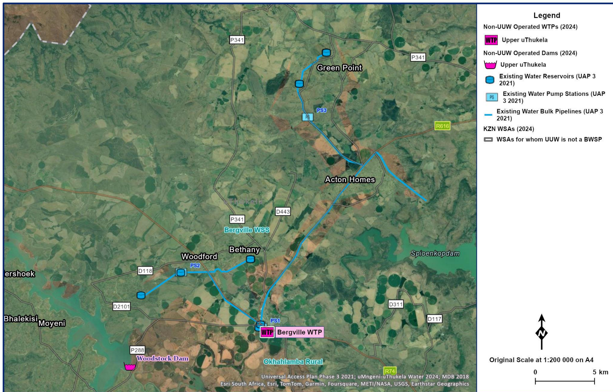
Figure 13.53 Bergville WTP Supply System Layout (NGI 2014; Umgeni Water 2020)
