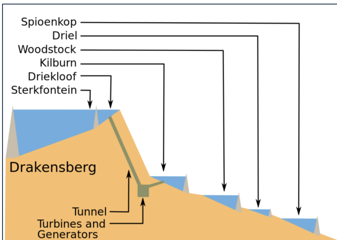
Figure 13.23 Longitudinal profile of the Thukela-Vaal Scheme and the Drakensberg Pumped Storage Scheme (Ladysmith Gazette 2017: website 15 ).
