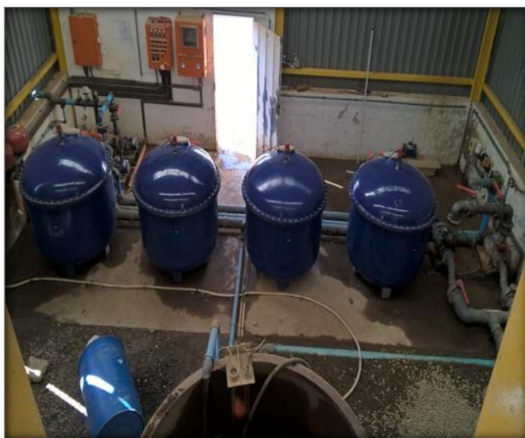
Figure 13.67 Weenen WTP (uMngeni-uThukela Water 2017)
