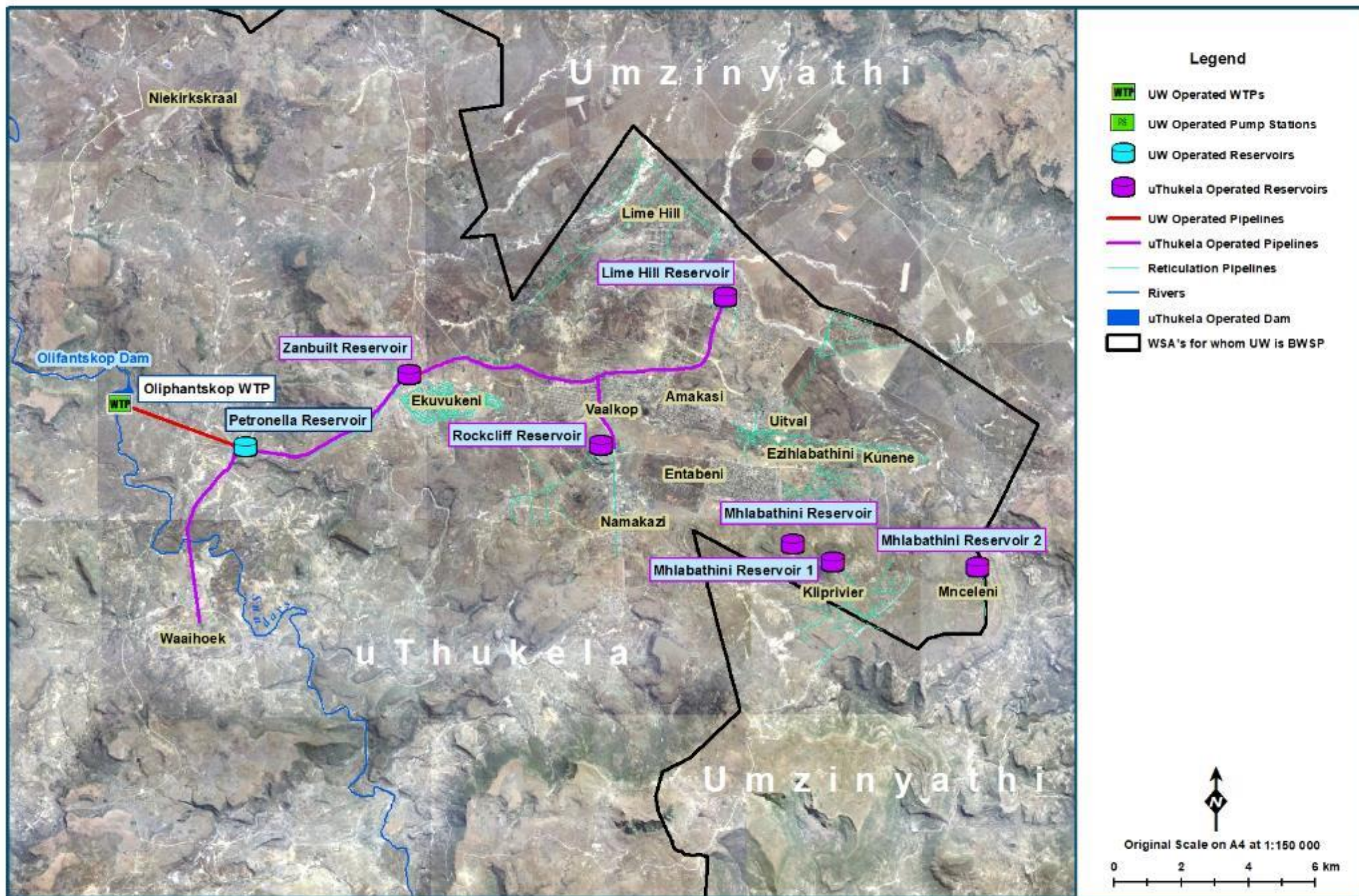
Figure 13.39 Olifantskop WTP Supply System layout (NGI 2014; Umgeni Water 2019).
