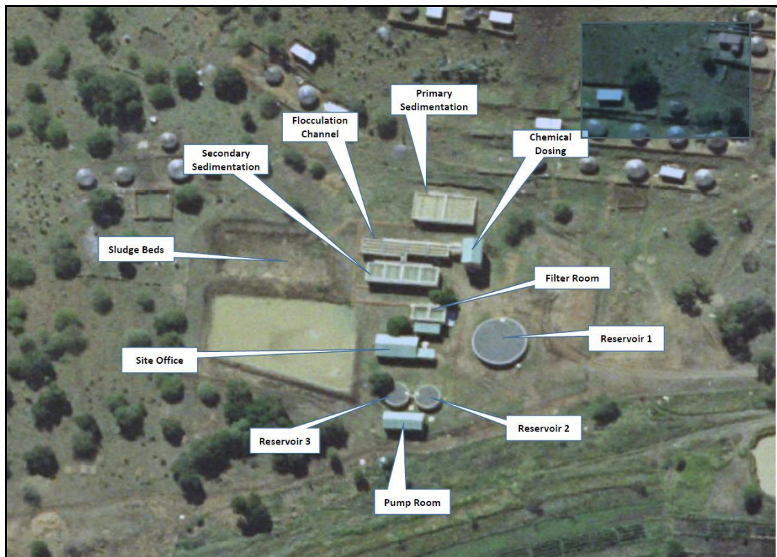
Figure 13.70 Overview of Tugela Ferry WTP, uMzinyathi DM O&M Manual (Dec2016)
