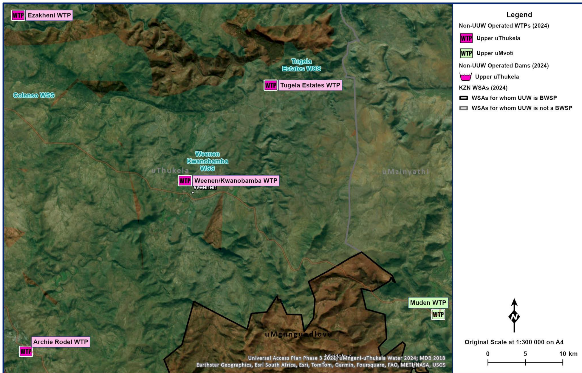
Figure 13.68 Weenen WTP Supply System Layout (NGI 2014; Umgeni Water 2020)
