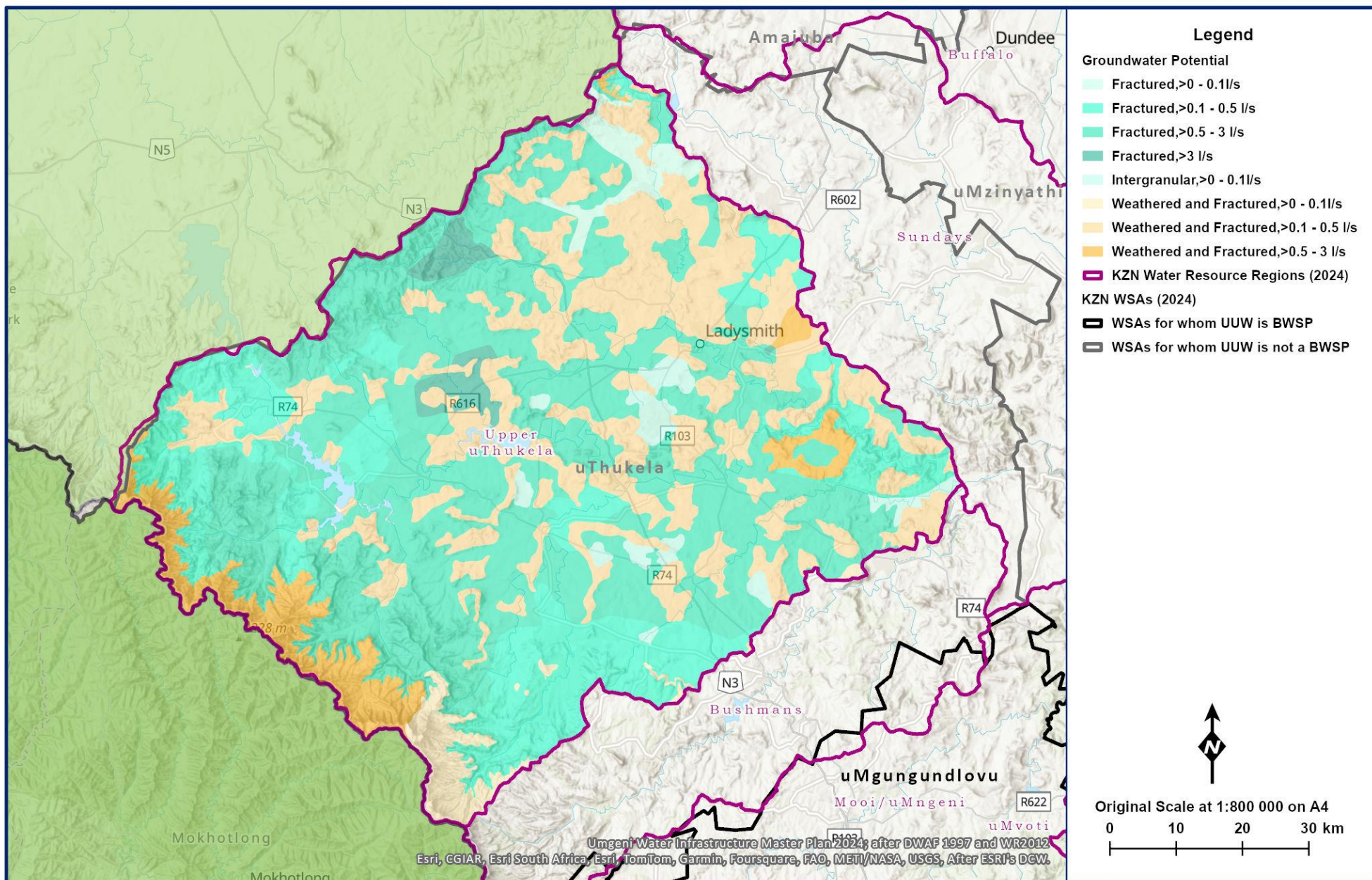
Figure 13.6 Groundwater potential in the Upper uThukela Region (MDB 2020, Umgeni Water 2022, after DWA 1997 and WR2012).
