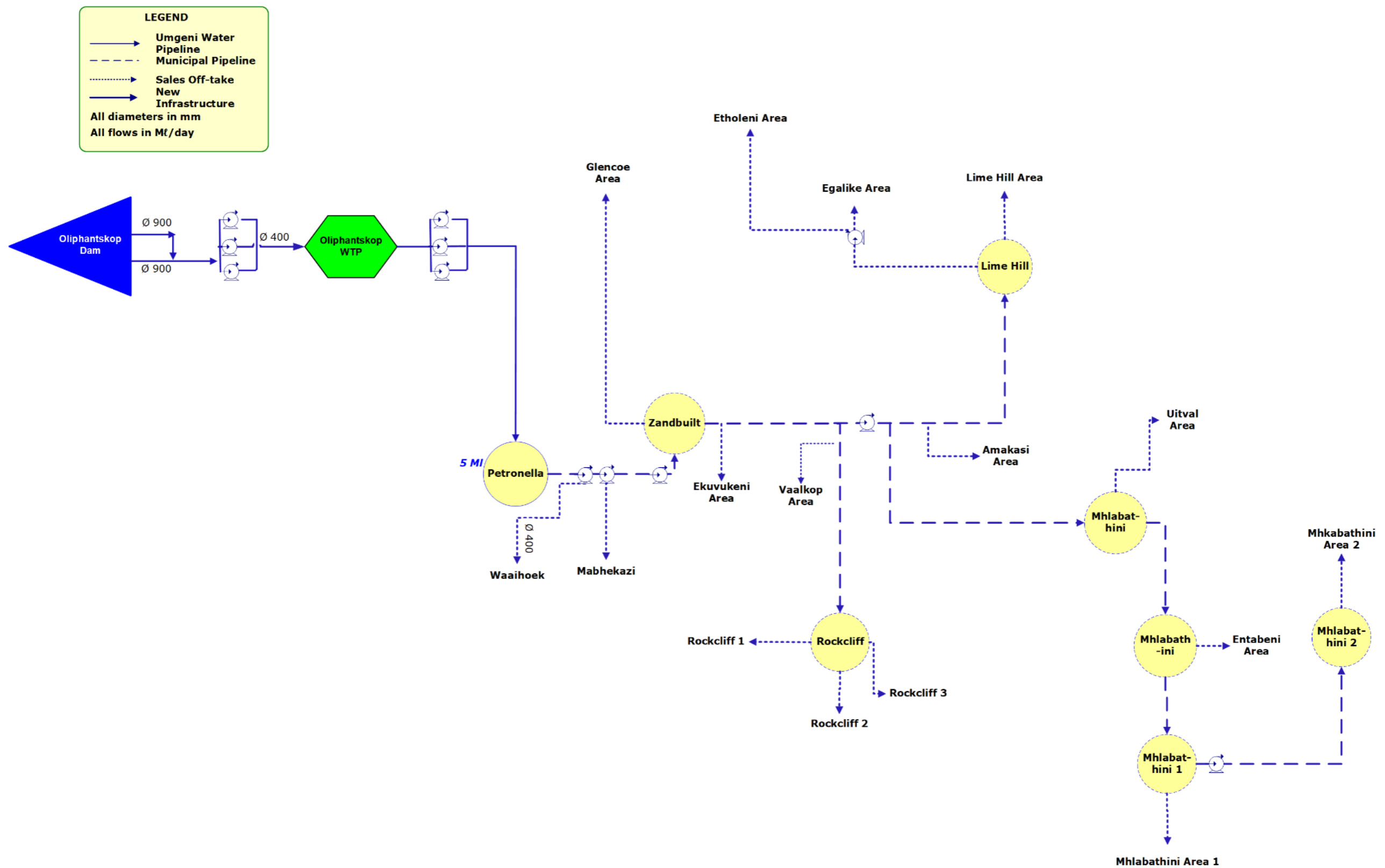
Figure 13.40 Oliphantskop WTP Supply System schematic.
