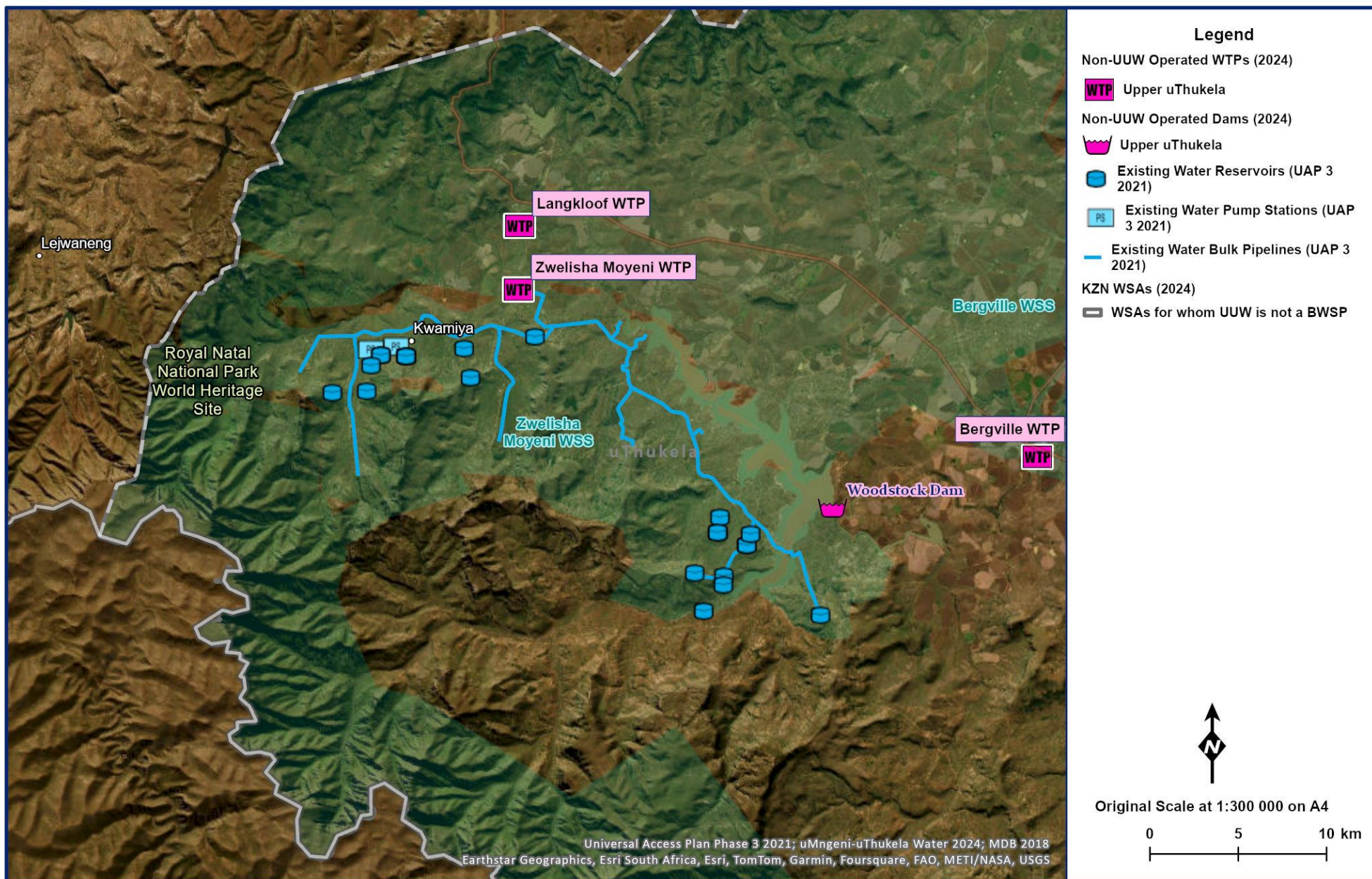
Figure 13.50 Zwelisha Moyeni WTP Supply System Layout NGI 2014; Umgeni Water 2020)
