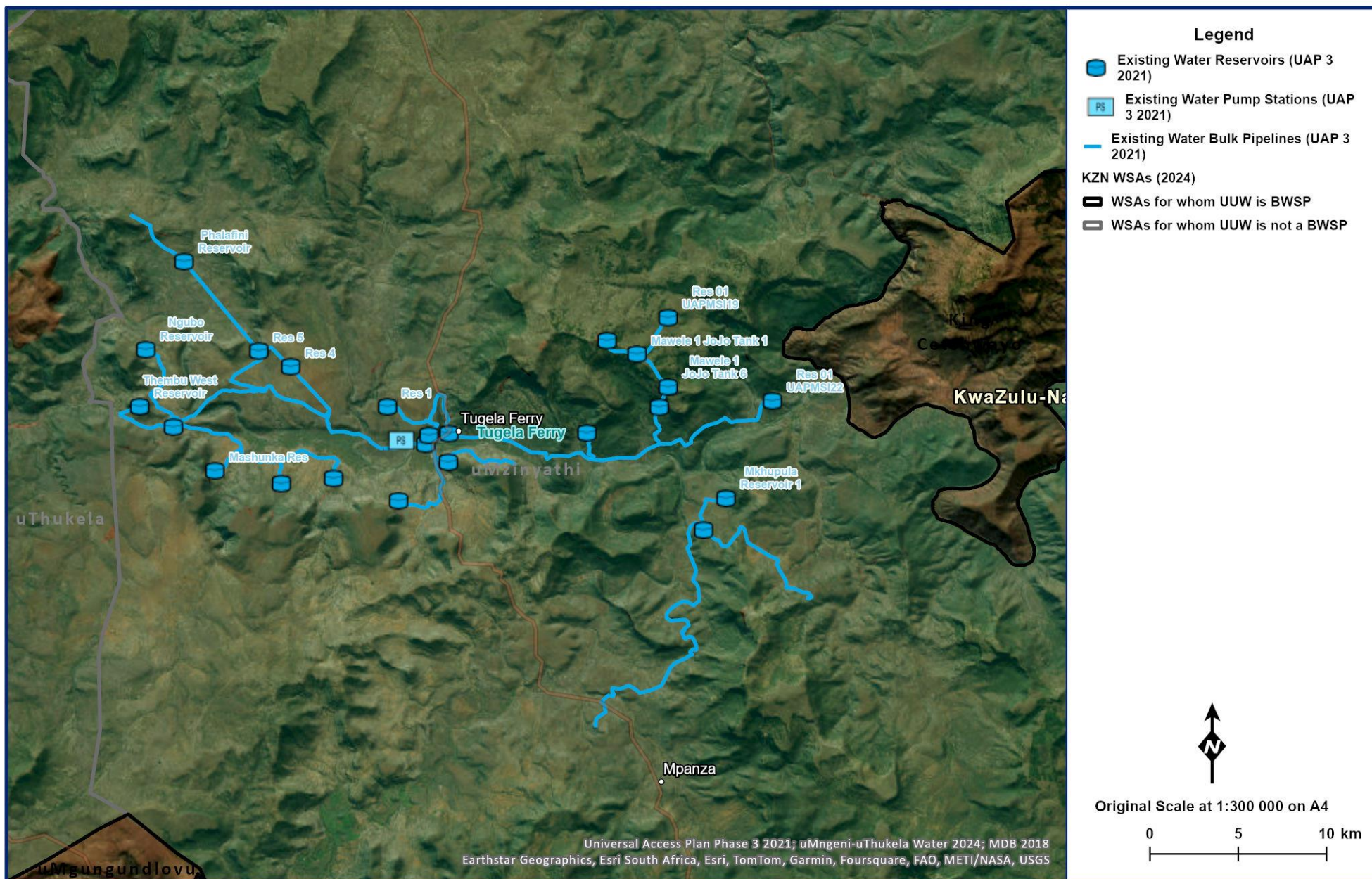
Figure 13.71 Tugela Ferry WTP Supply System Layout (NGI 2014; Umgeni Water 2020)
