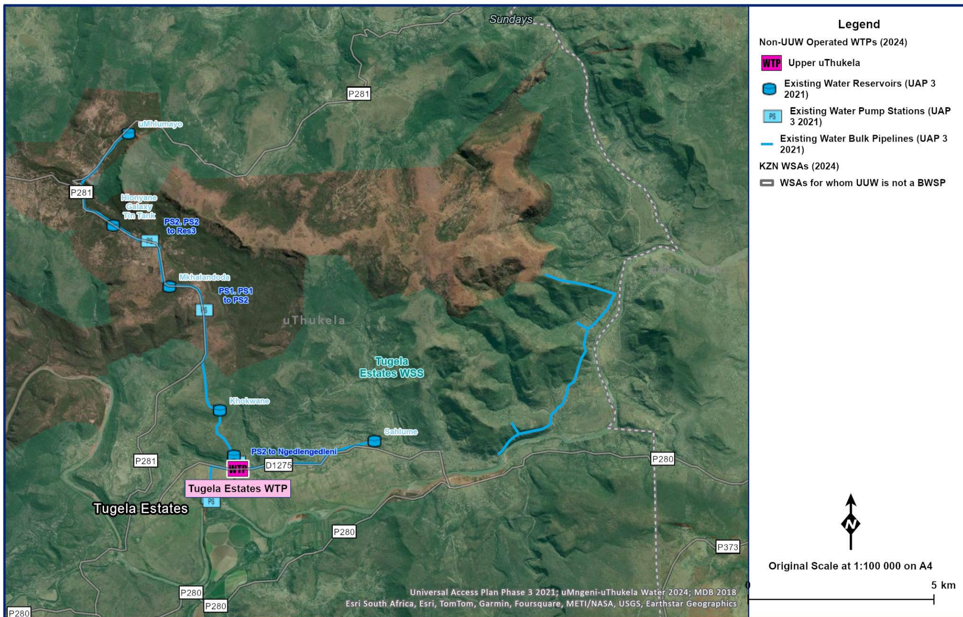
Figure 13.29 Tugela Estates WTP and uMhlamayo Borehole Supply System layout (NGI 2014; Umgeni Water 2019).
