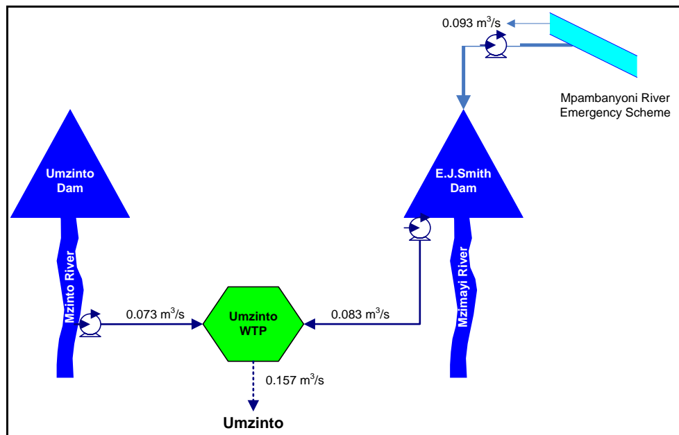
Figure 11.20 Schematic of the Middle South Coast system.
