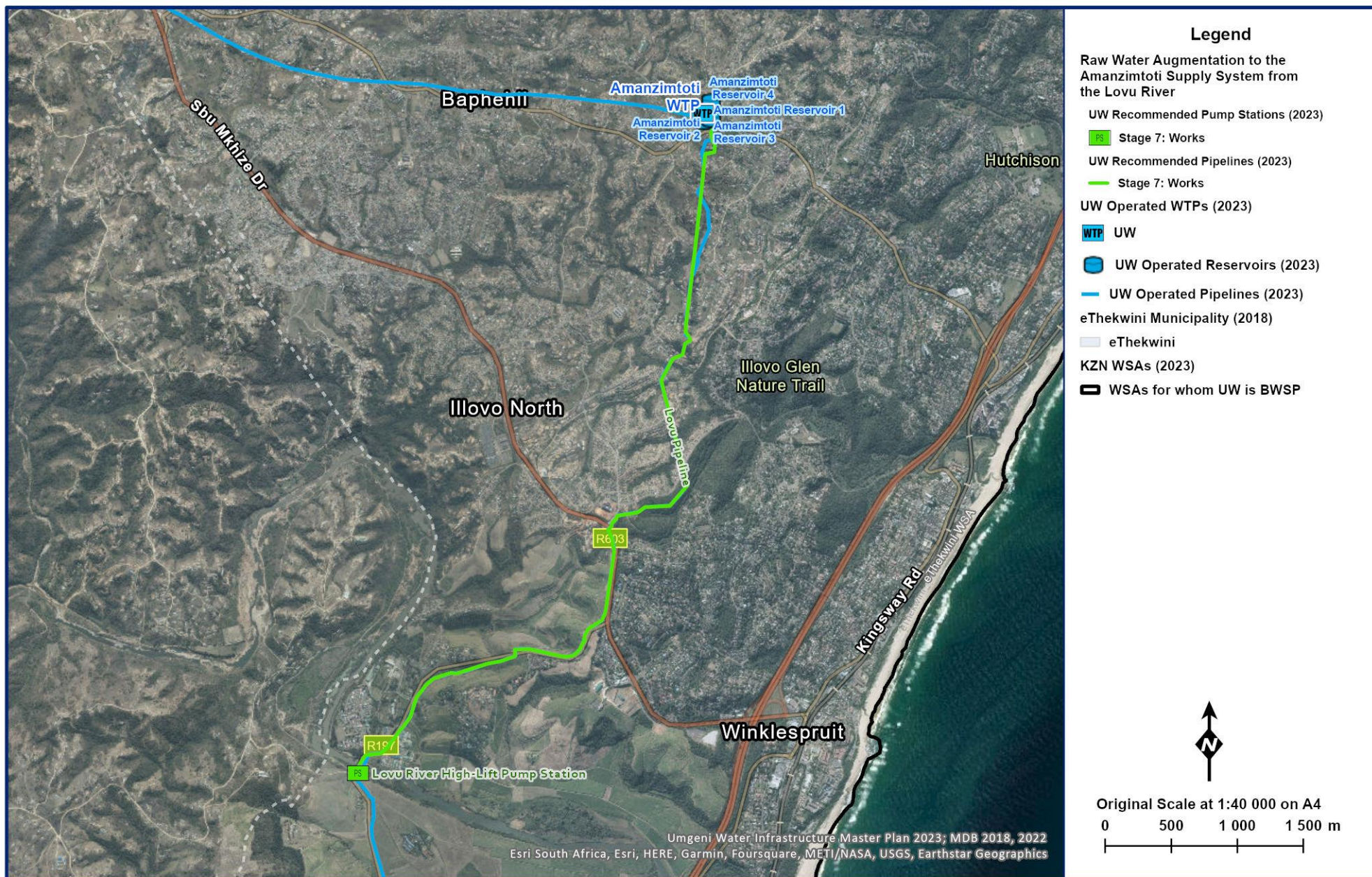
Figure 11.75 Layout of proposed raw water augmentation to the Amanzimtoti Supply System from the Lovu River.
