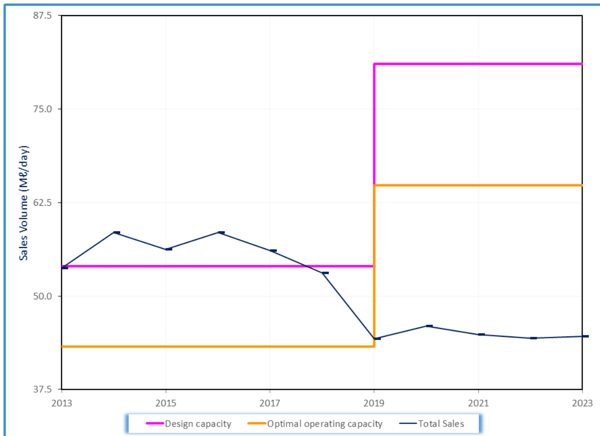
Figure 11.37 Analysis of historical production at Bhubhoyi WTP (January 2013 to June 2023).
