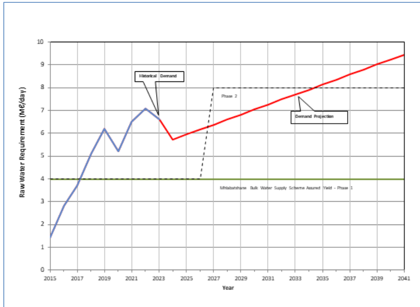
Figure 11.71 Water Balance Mhlabatshane BWSS.
