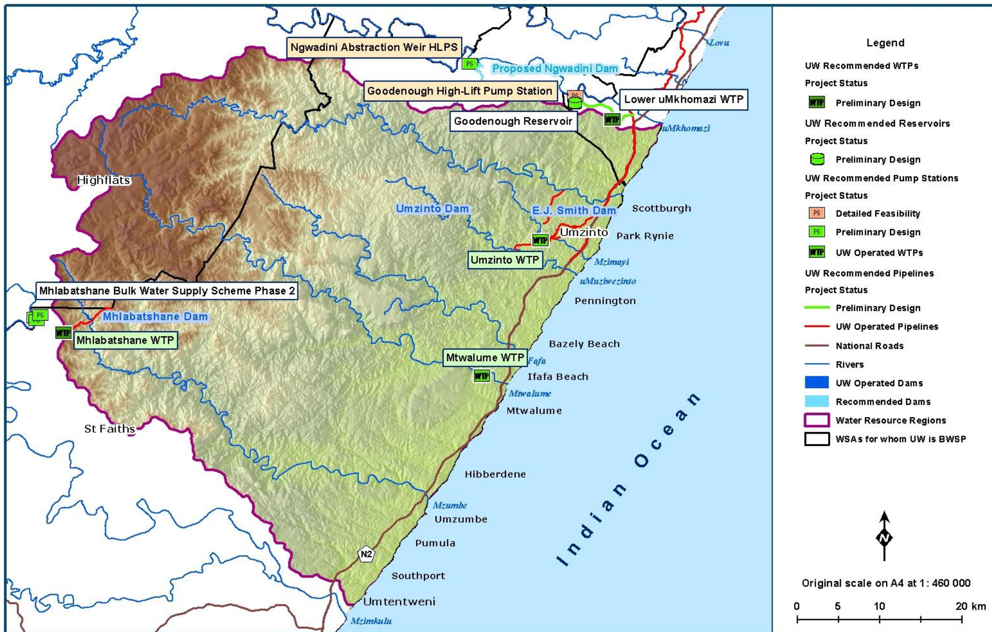
Figure 11.67 Proposed water resource infrastructure in the Middle South Coast Region (KZN DoT 2011; MDB 2016; Umgeni Water 2017; WR2012).
