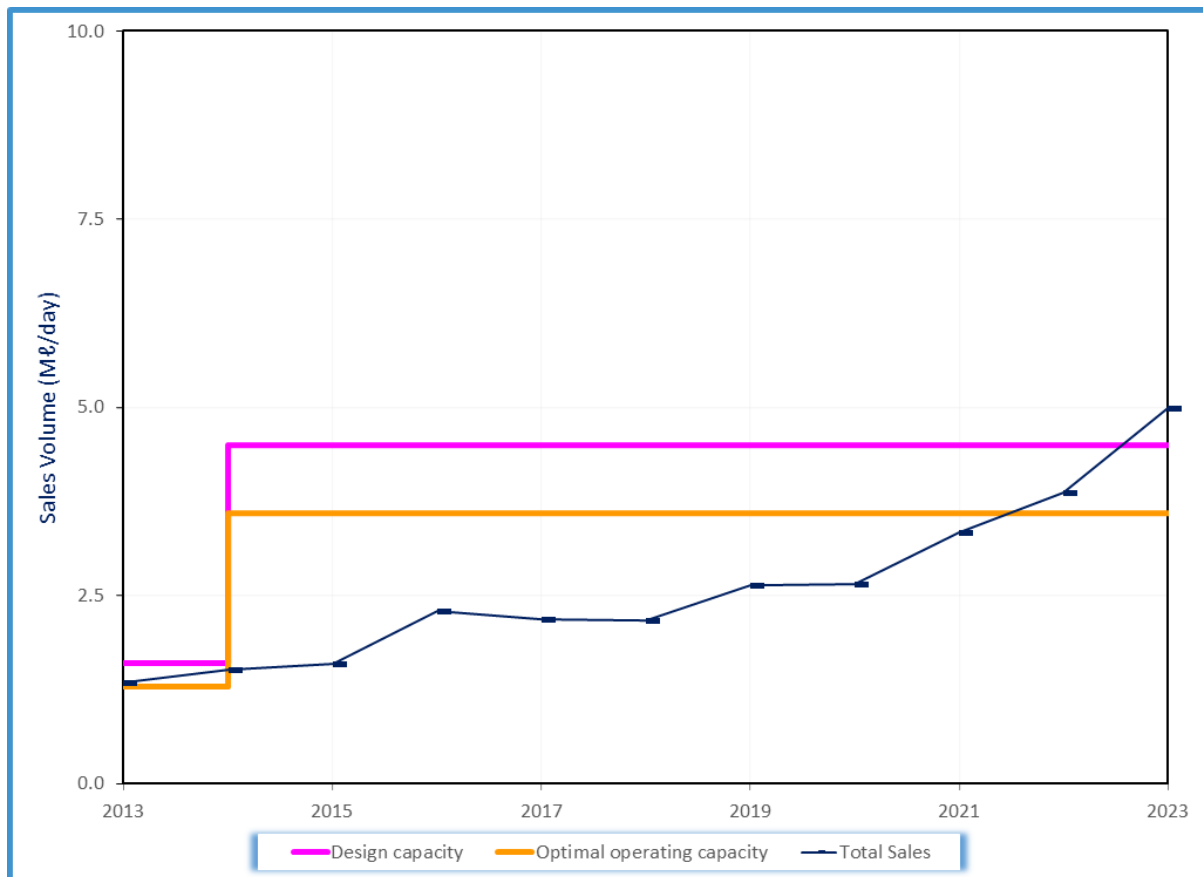
Figure 11.41 Analysis of historical production at Vulamehlo WTP (January 2013 to June 2023).
