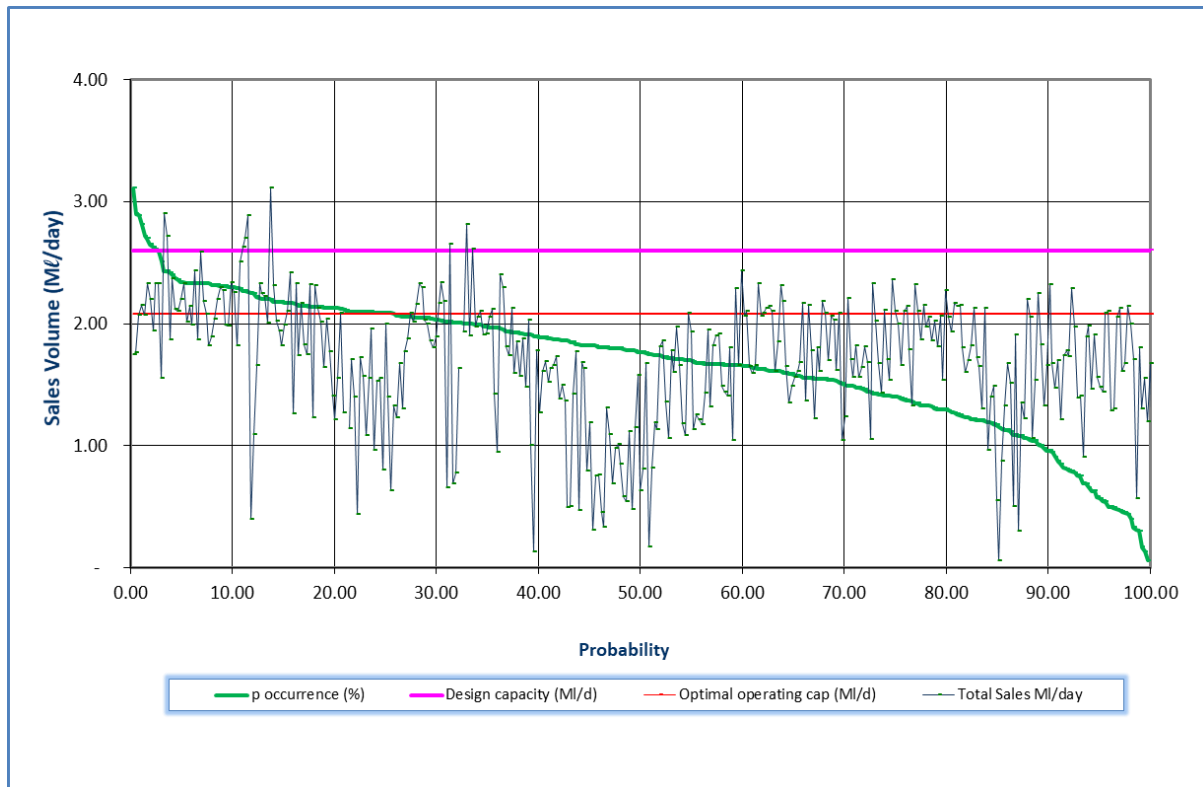
Figure 11.39 Analysis of historical production at Harding WTP (November 2022 to October 2023).
