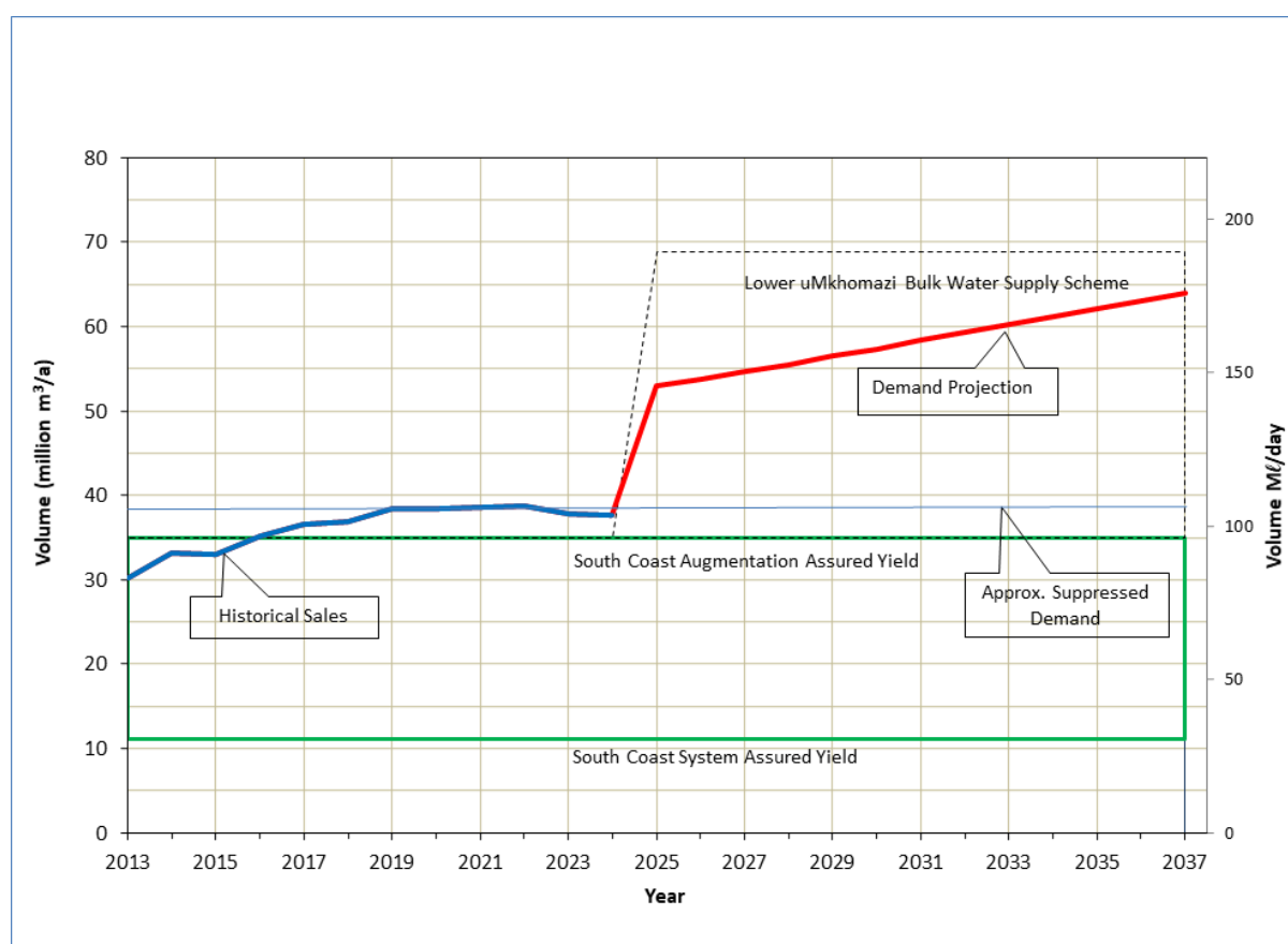
Figure 11.72 Water Balance Upper and Middle South Coast.
