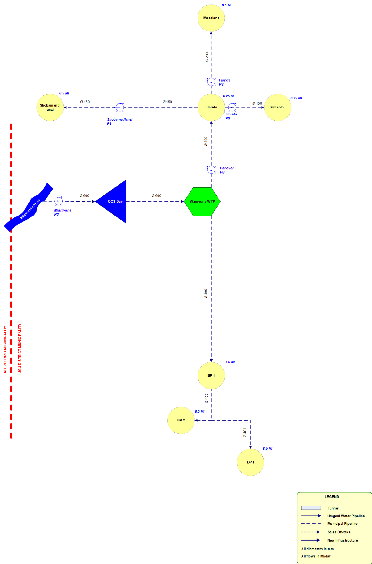
Figure 11.49 Schematic of the uMtamvuna System Bulk Supply Infrastructure.
