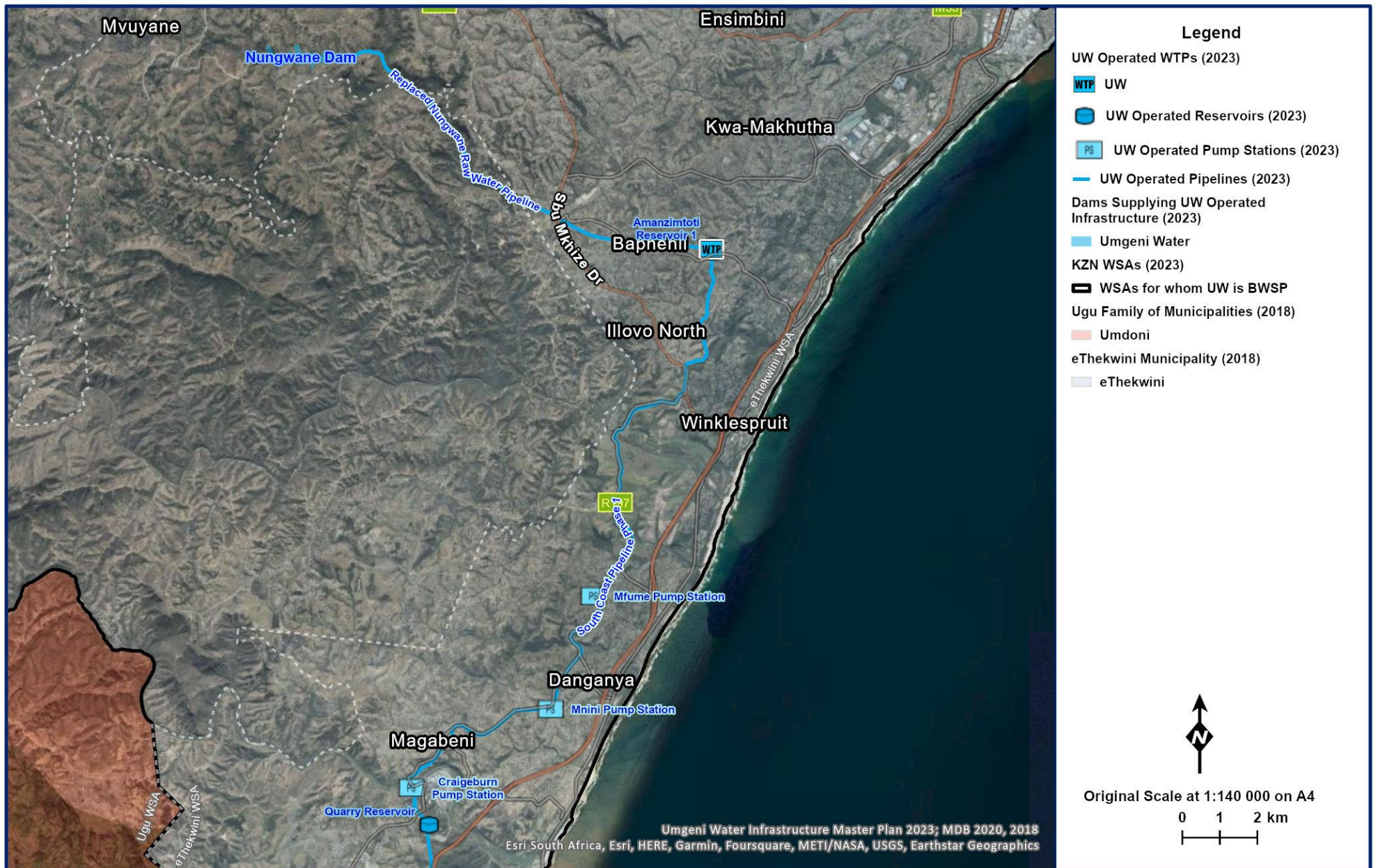
Figure 11.22 Amanzimtoti WTP to Quarry Reservoir.
