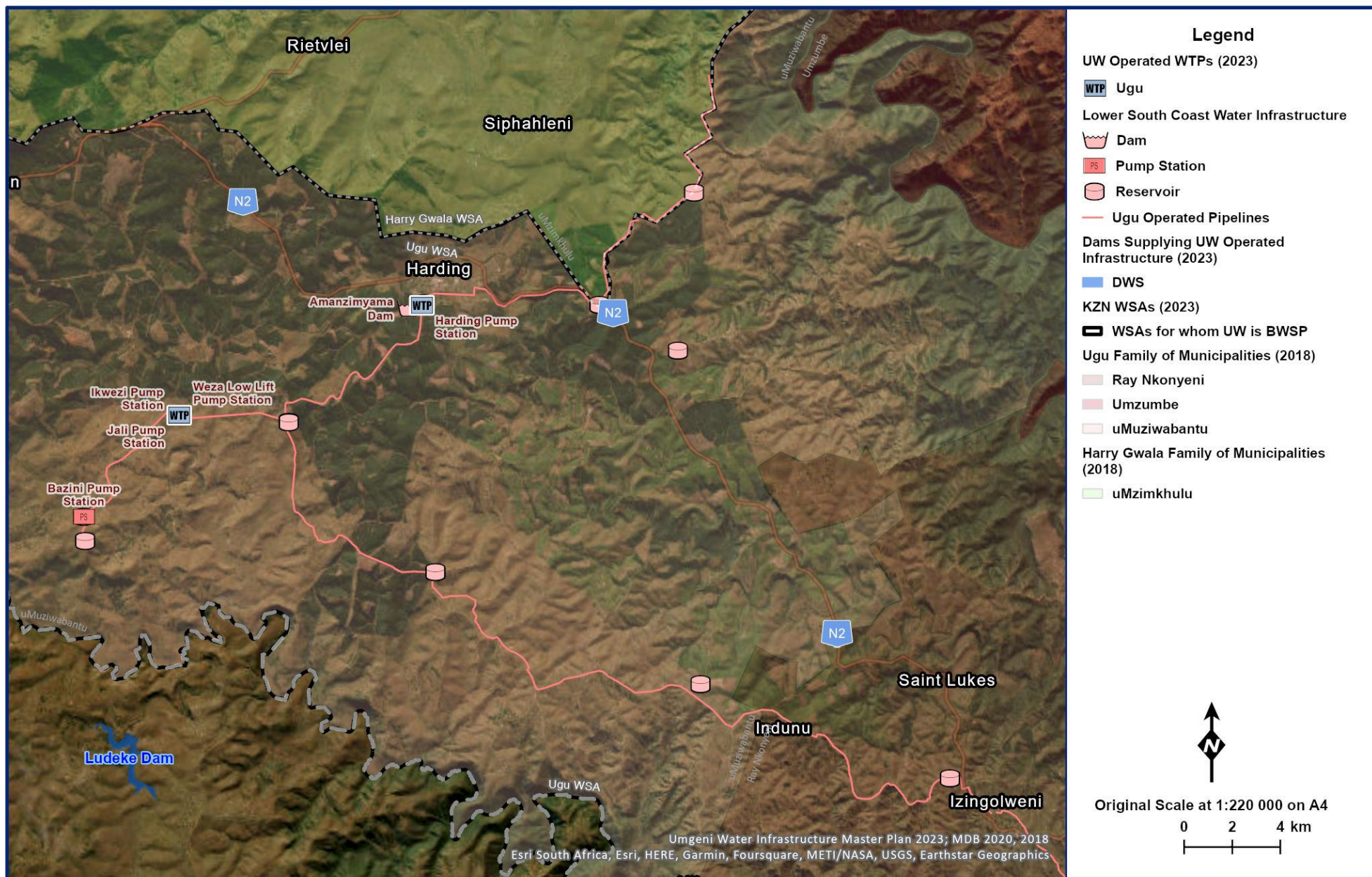
Figure 11.31 Harding-Weza Supply System.
