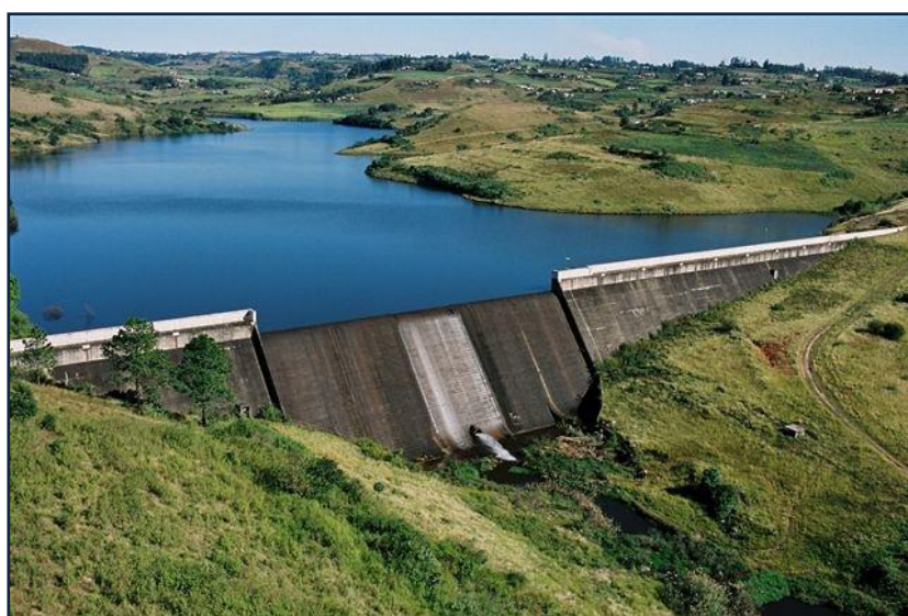
Figure 11.14 Nungwane Dam.
