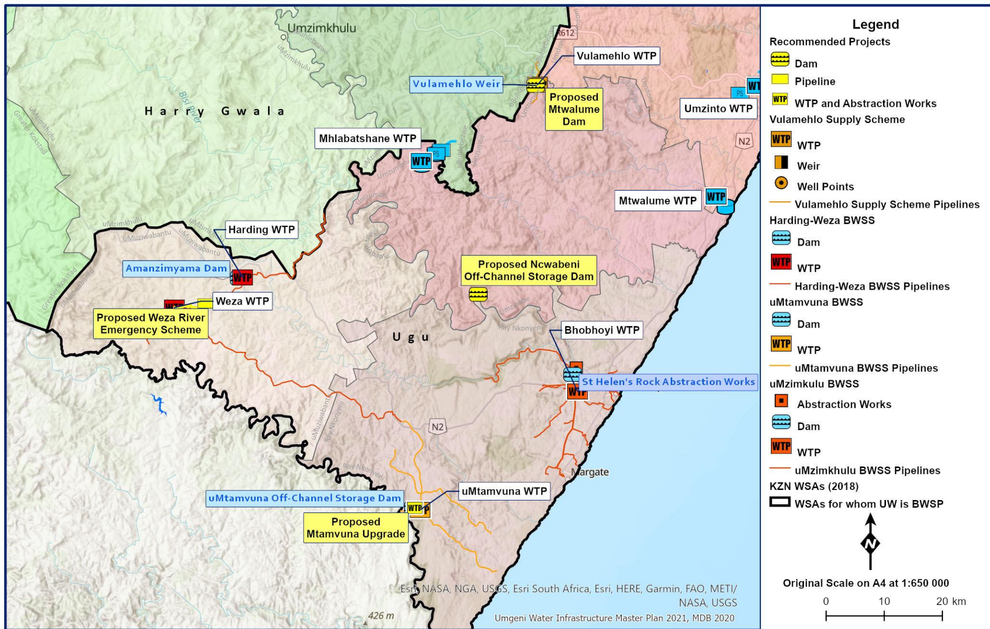
Figure 11.68 Proposed water resource infrastructure in the Lower South Coast Region (KZN DoT 2017; MDB 2016; Umgeni Water 2020; WR2012).
