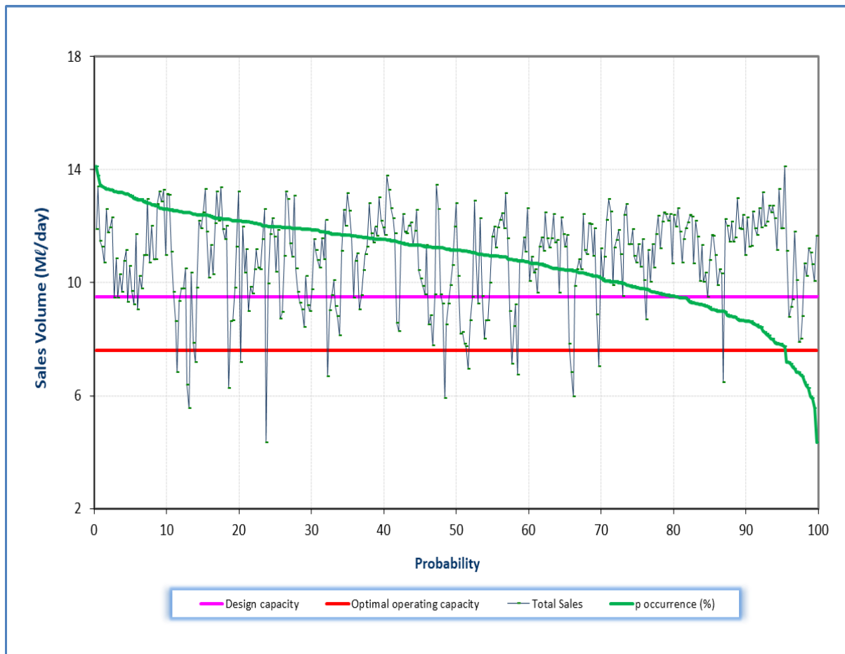
Figure 11.35 Analysis of historical production at Mtwalume WTP (November 2022 to October 2023).
