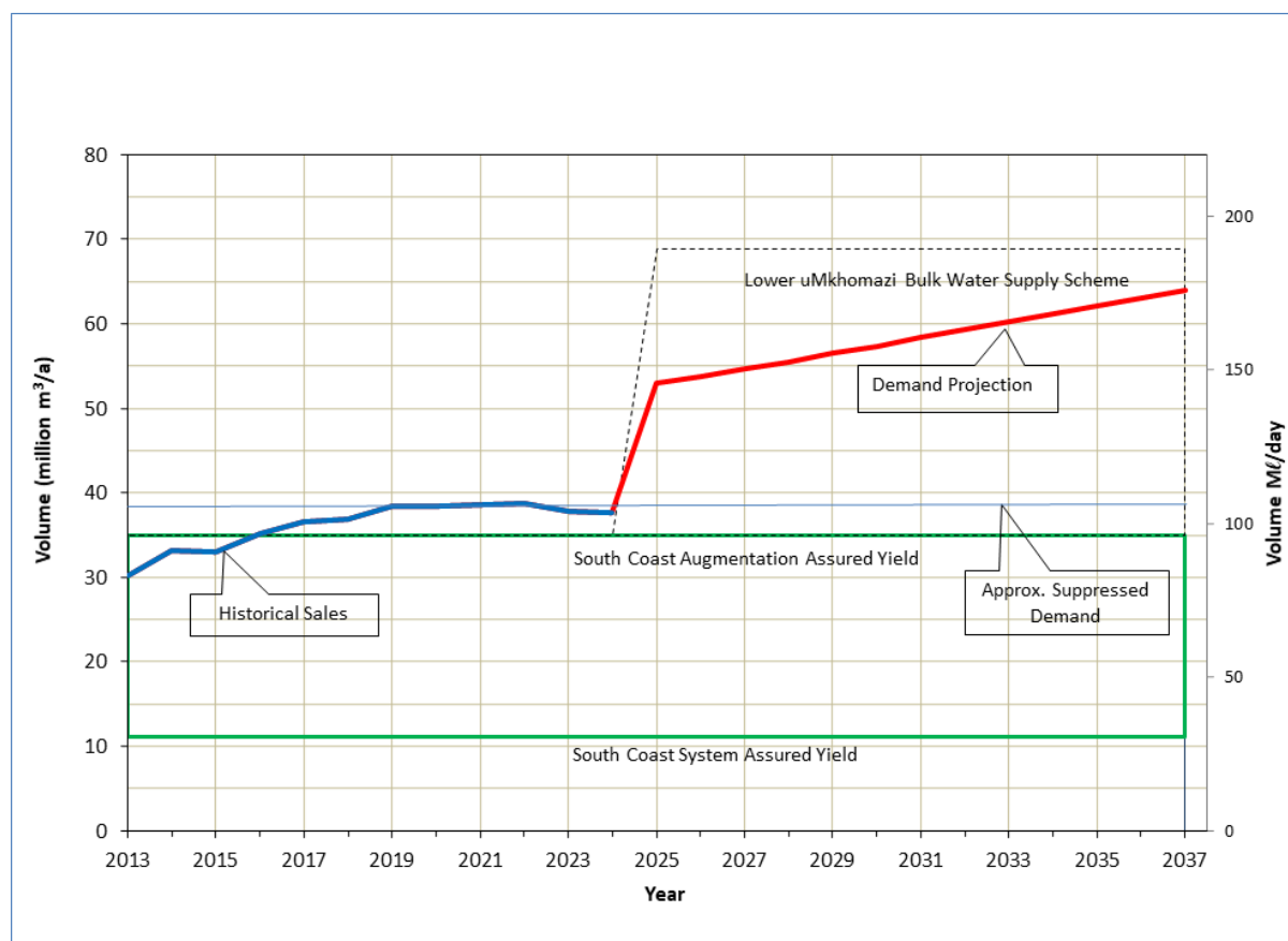
Figure 11.61 Upper and Middle South Coast water requirement projection scenarios.
