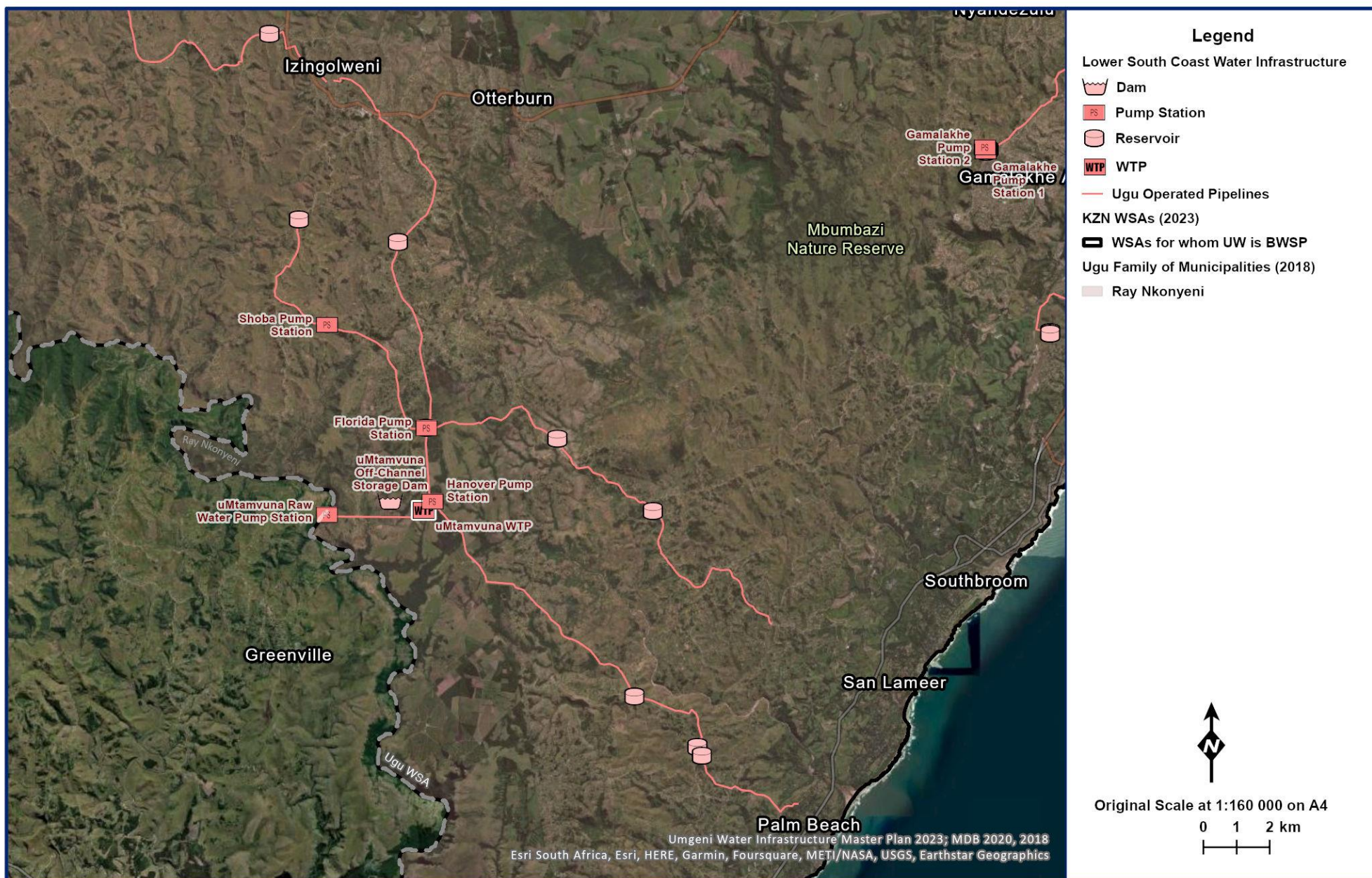
Figure 11.30 uMtamvuna Supply System.
