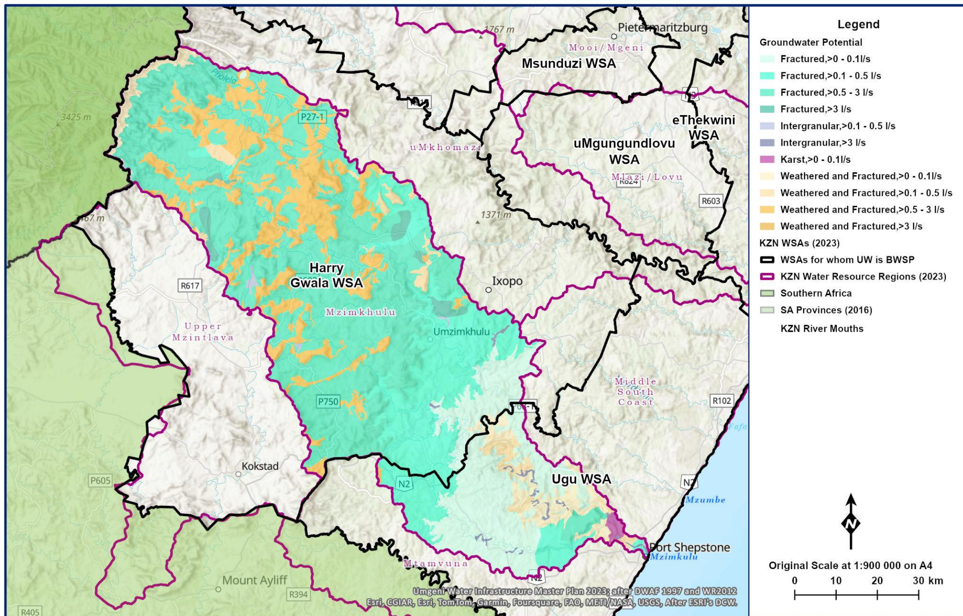
Figure 11.11 Groundwater potential in the Mzimkulu Region (MDB 2020; Umgeni Water 2022; after DWAF 1997 and WR2012).
