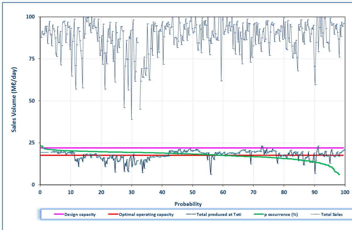
Figure 11.33 Analysis of historical production at Amanzimtoti WTP (November 2022 to October 2023).
