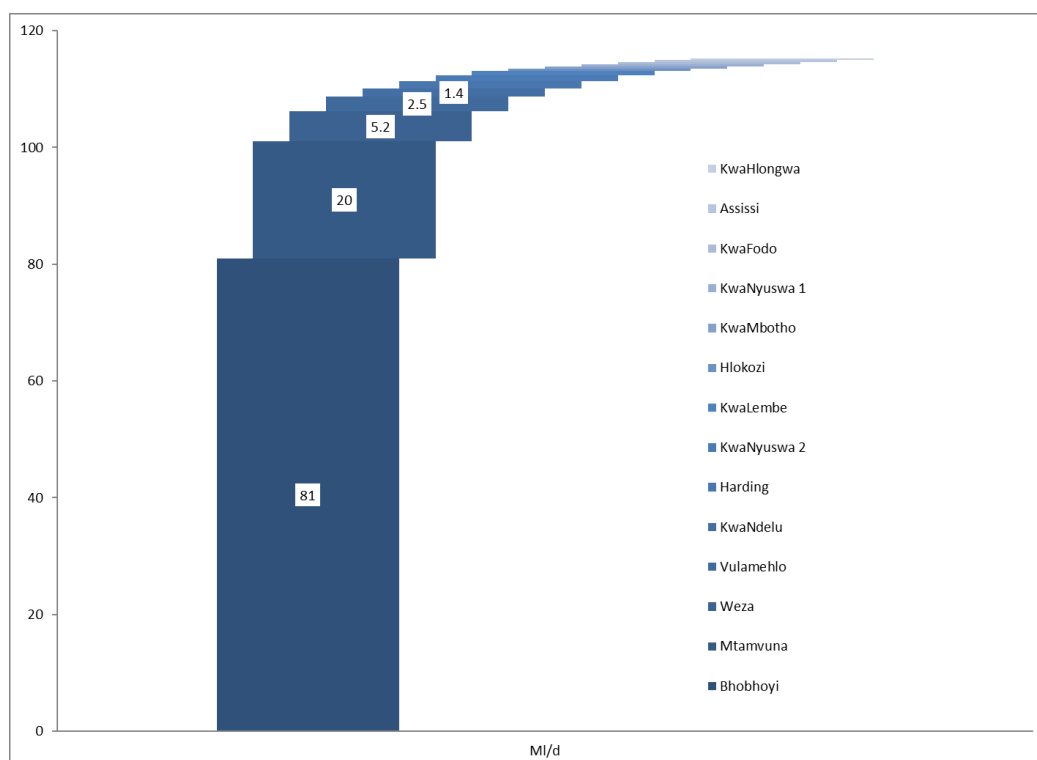
Figure 11.27 Water Treatment Plants Capacity.
