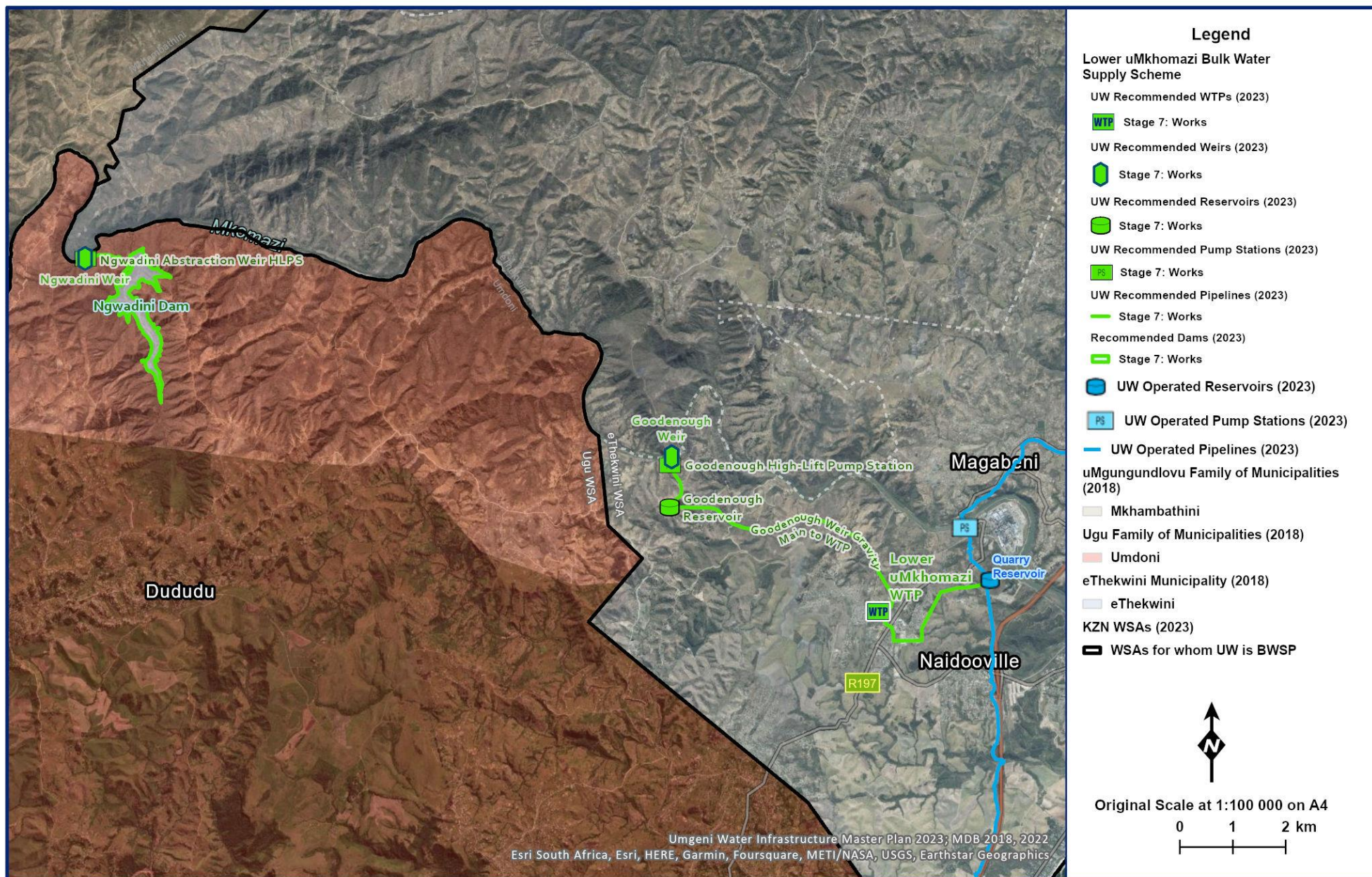
Figure 11.73 Layout of the proposed Lower uMkhomazi BWSS.
