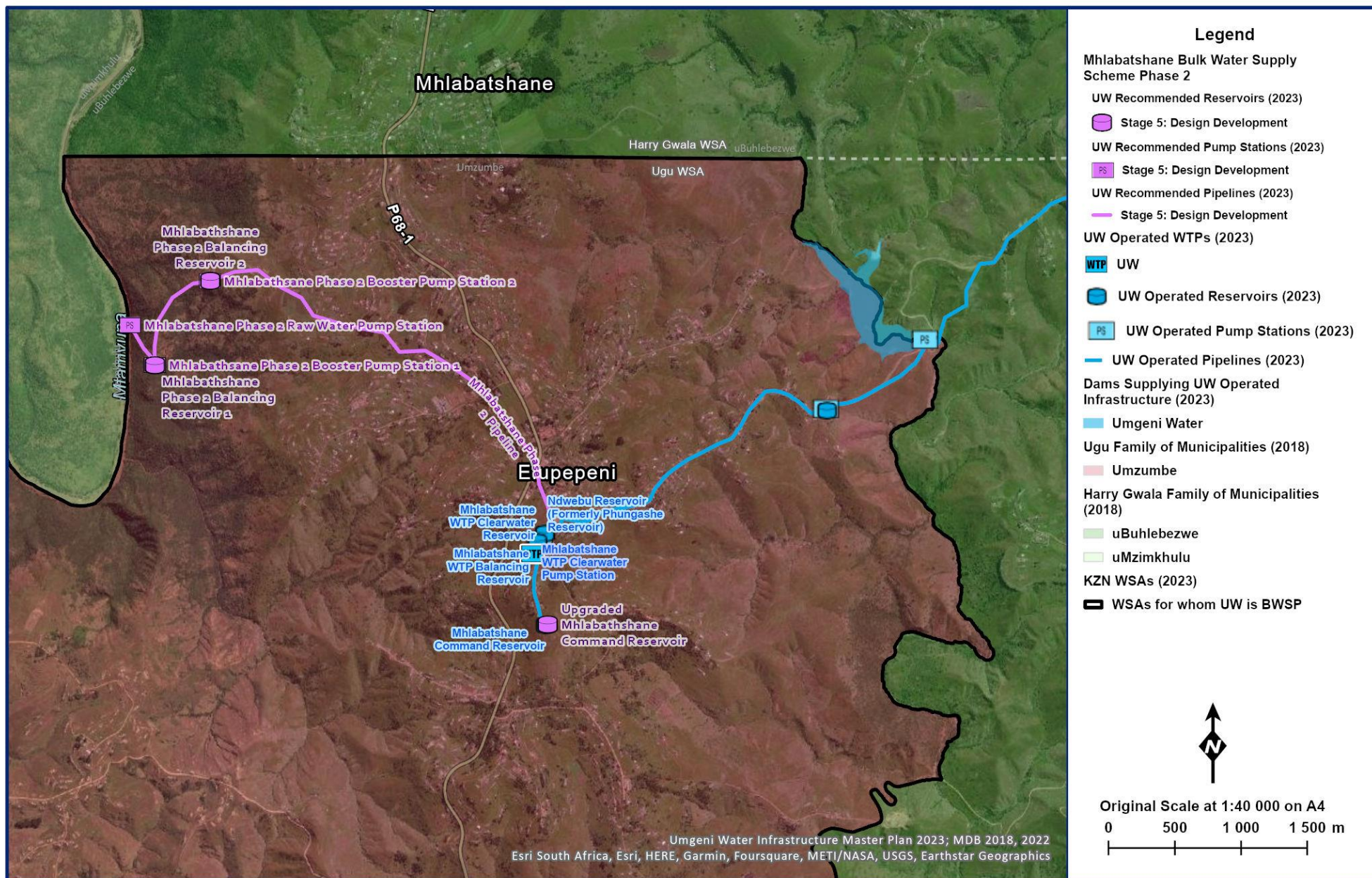
Figure 11.70 General layout of the Mhlabatshane BWSS Phase 2.
