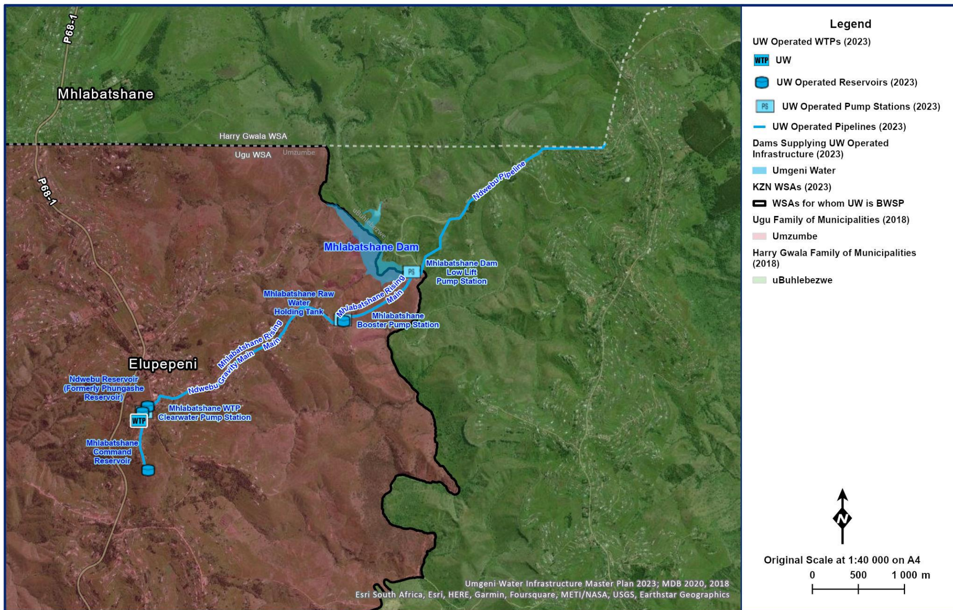
Figure 11.28 Mhlabatshane Supply System.
