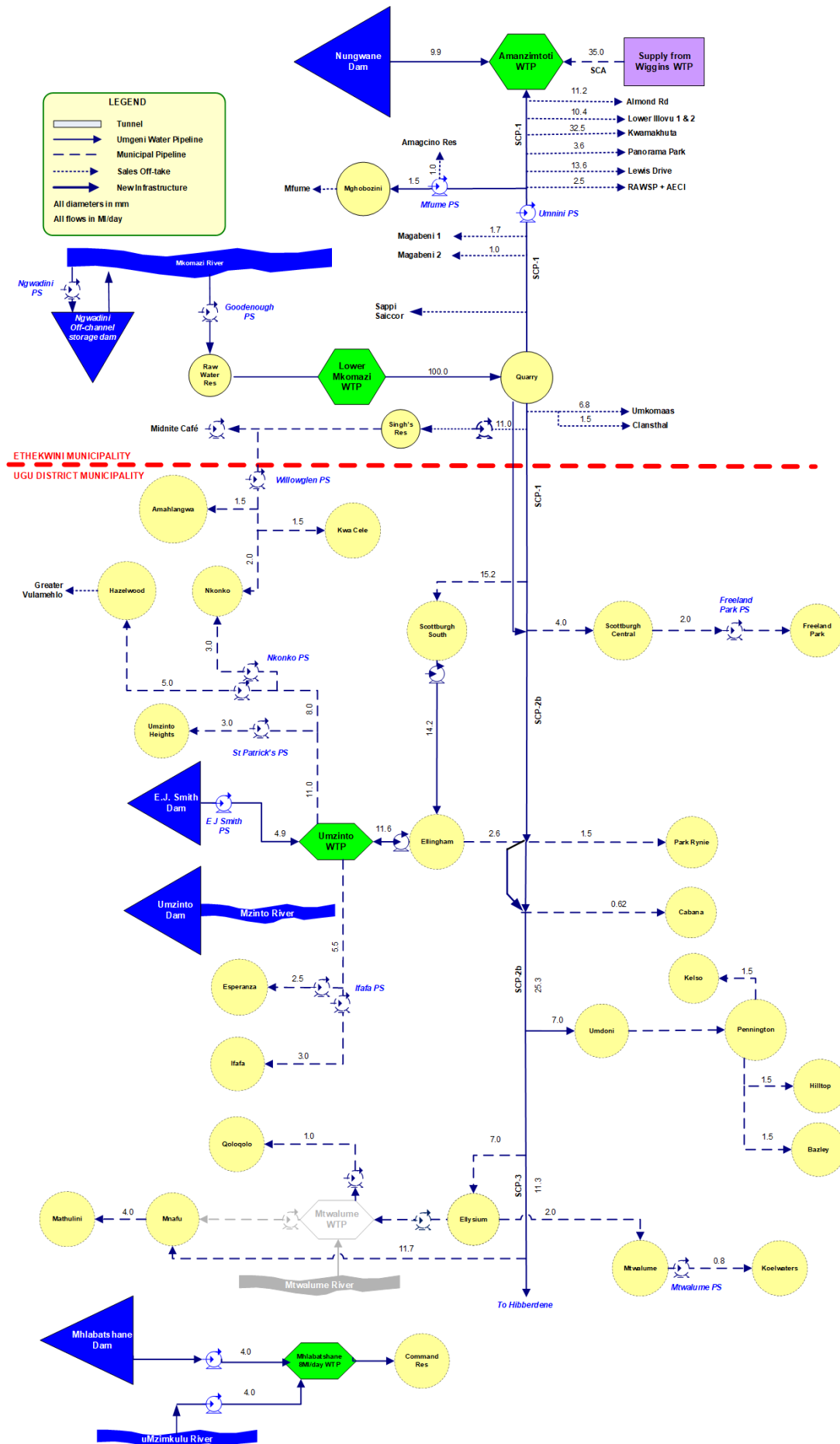
Figure 11.47 Thirty year demand projection for the South Coast System.
