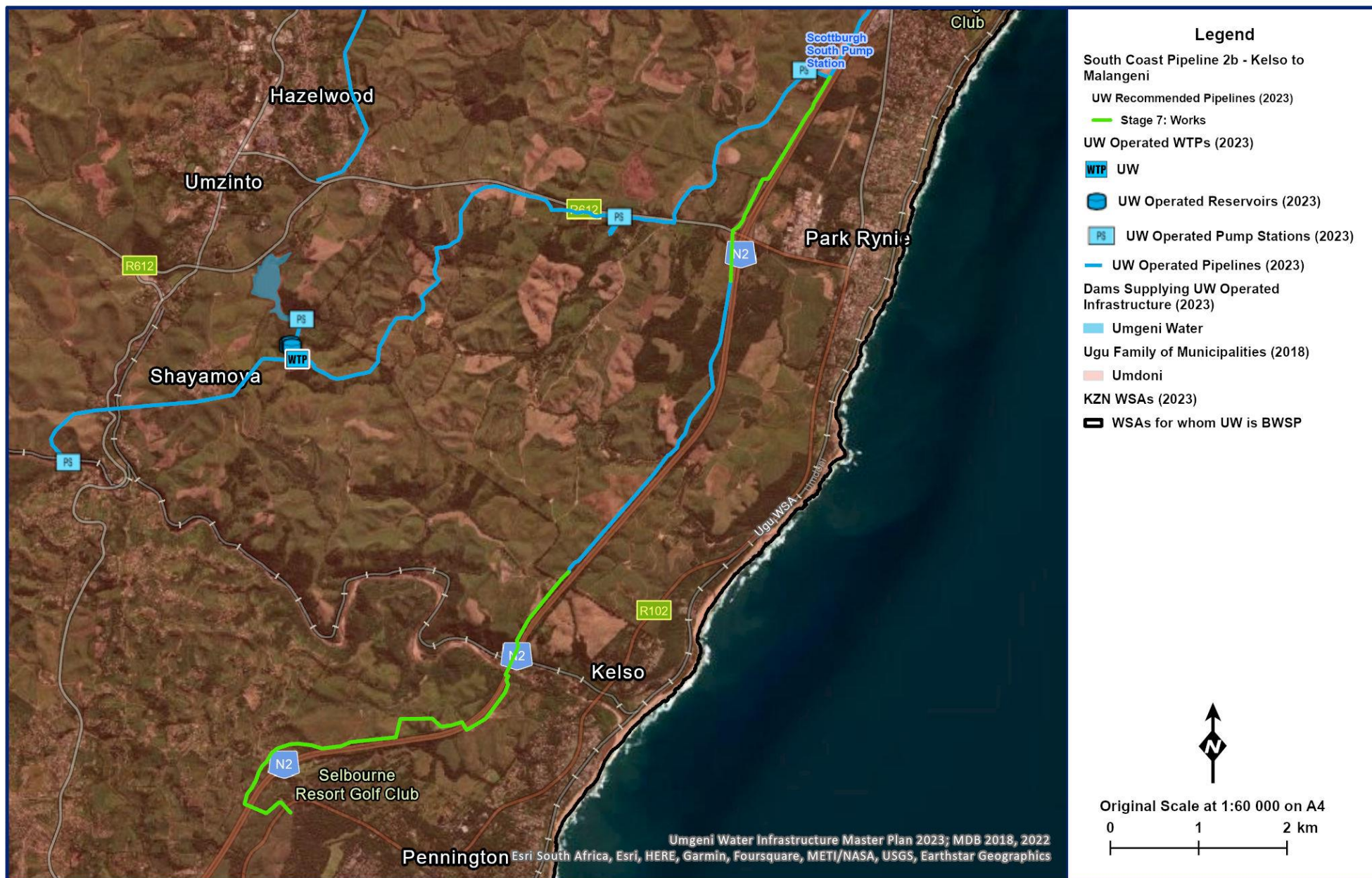
Figure 11.69 General layout of the proposed South Coast Pipeline Phase 2b.
