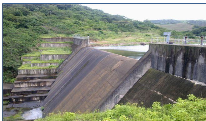
Figure 11.15 Umzinto Dam.
