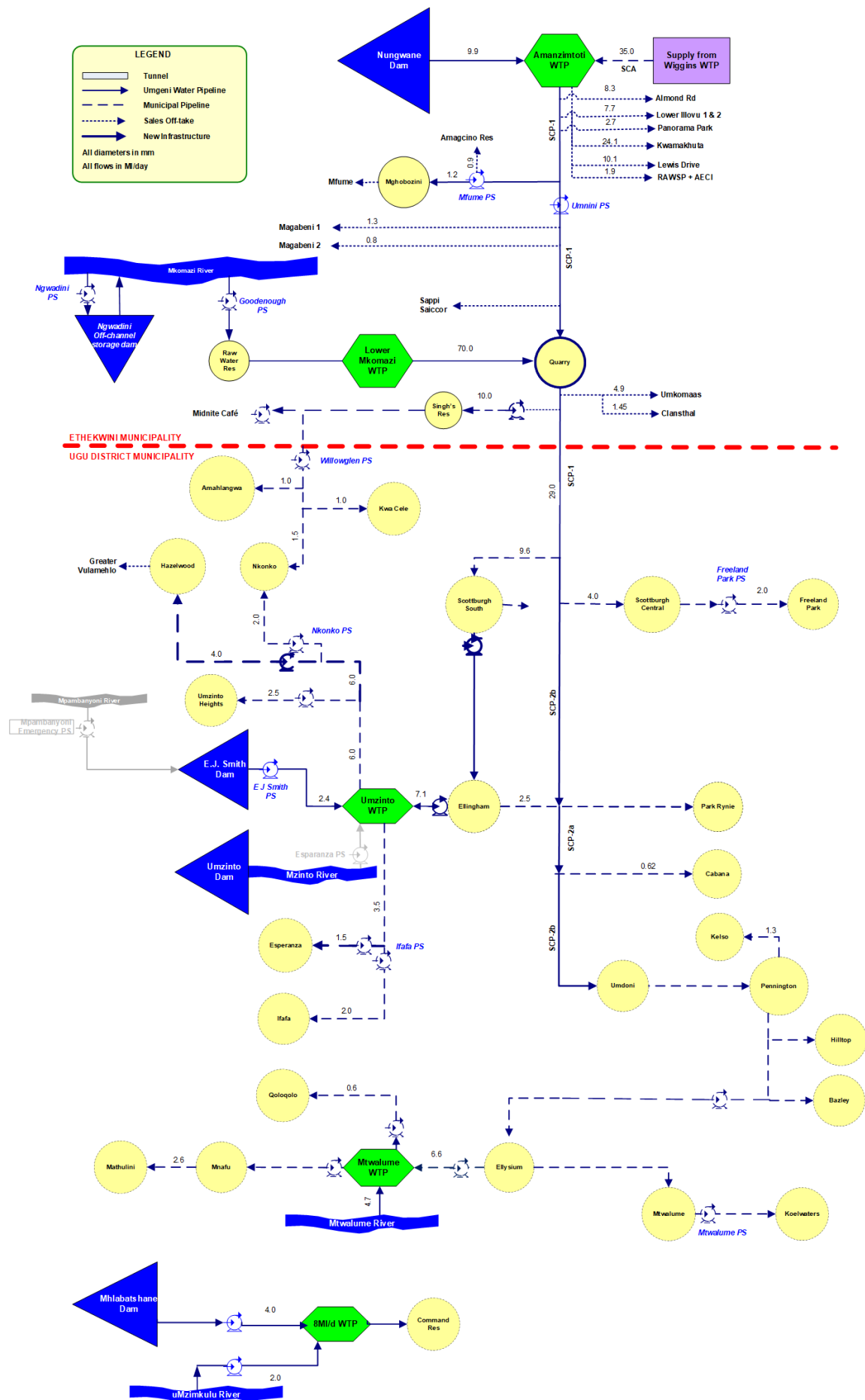
Figure 11.44 Ten year demand and projection for the South Coast System.
