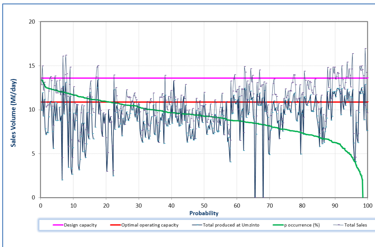
Figure 11.34 Analysis of historical production at Umzinto WTP (November 2022 to October 2023).
