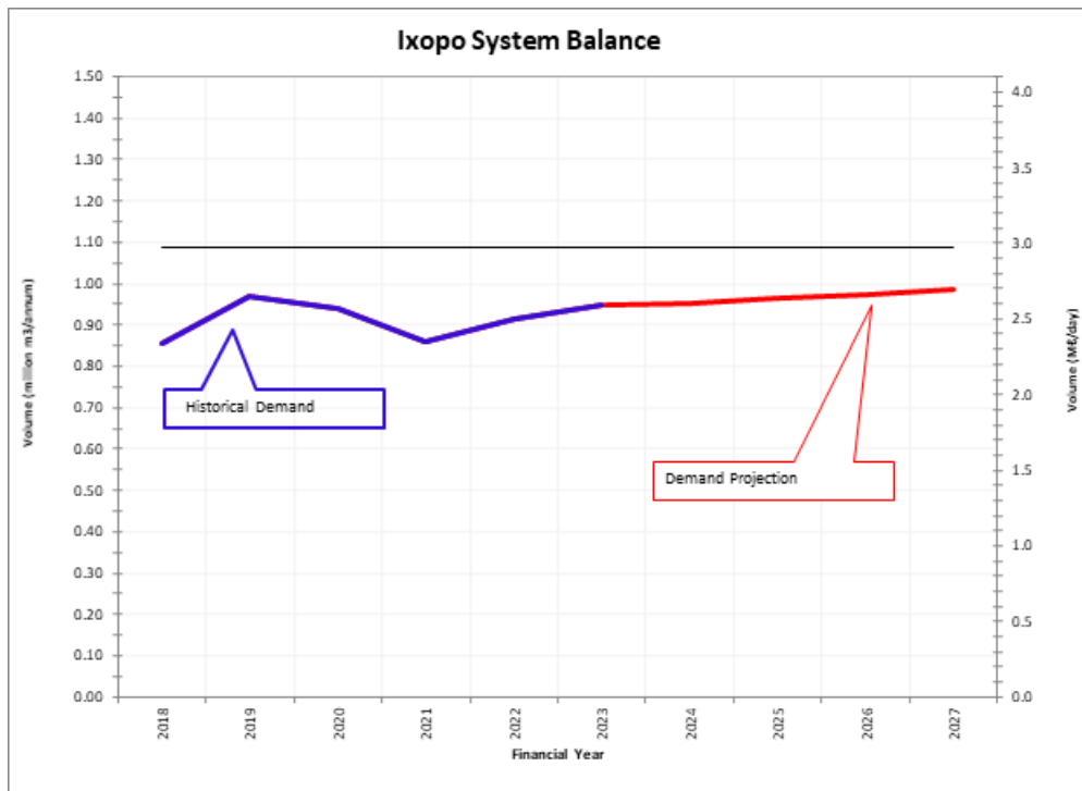
Figure 8.8 Ixopo System Water Balance.
