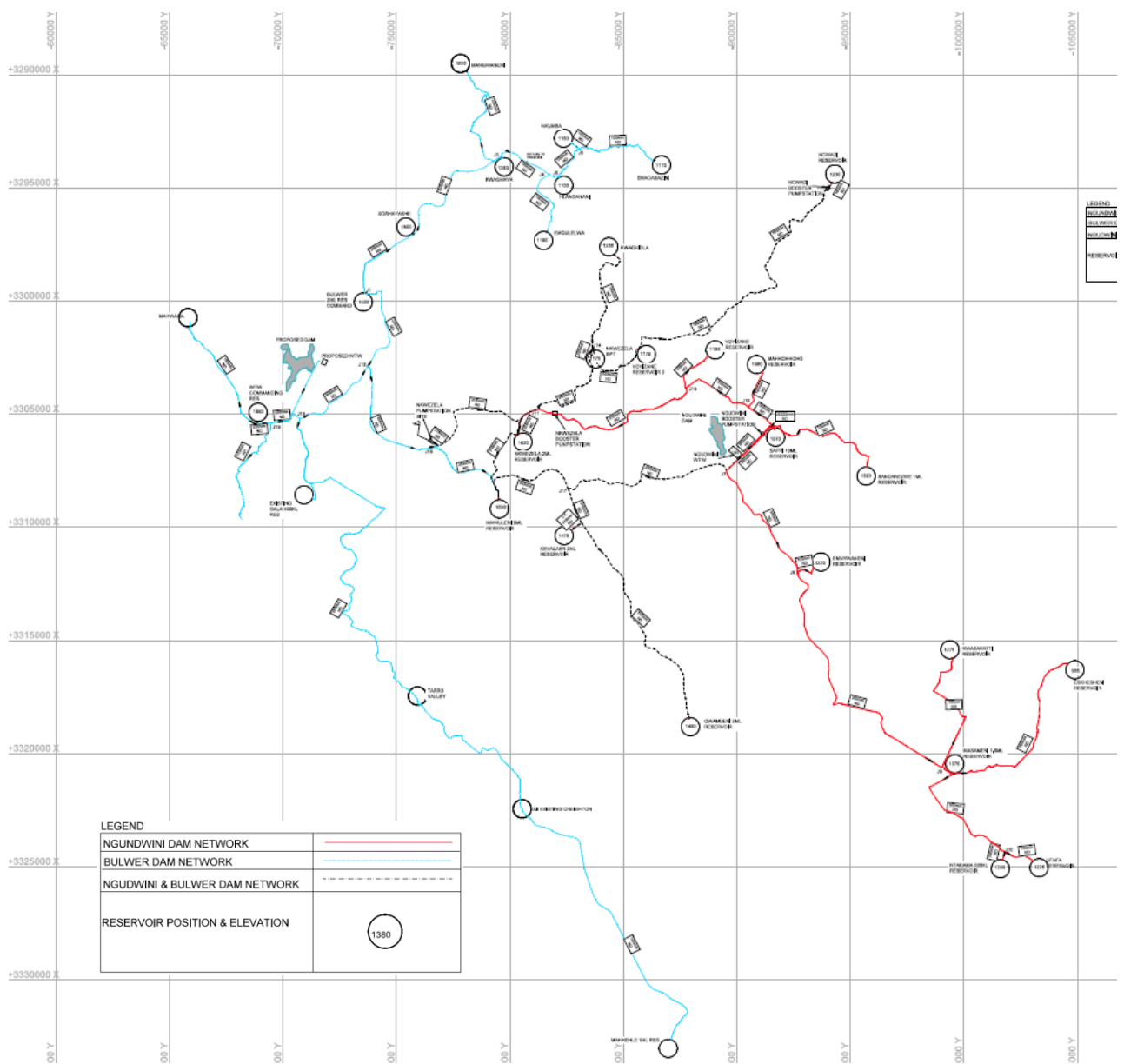
Figure 8.12 Overall Layout of the HGDM RBWSS
