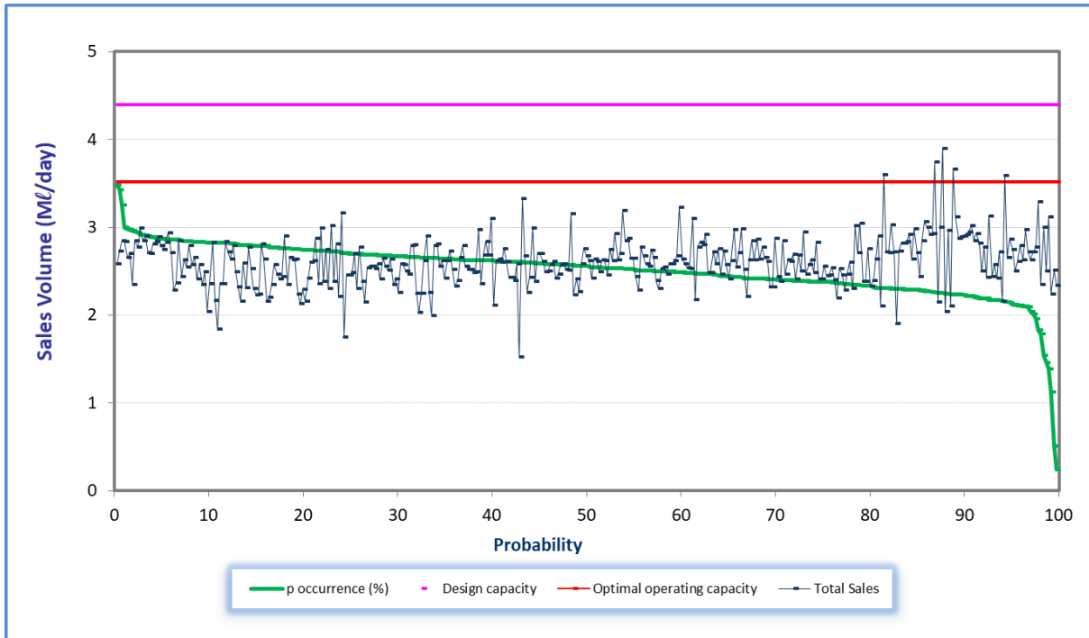
Figure 8.7 Analysis of historical production at Ixopo WTP (November 2022 to October 2023).
