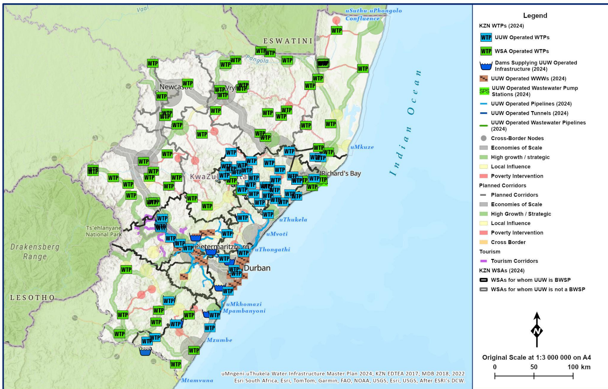
Figure 2.60 KZN WTPs in relation to the KZN PSEDs 2016 (KZN DoT 2021; KZN EDTEA 2017; MDB 2018; uMngeni-uThukela Water 2023).
