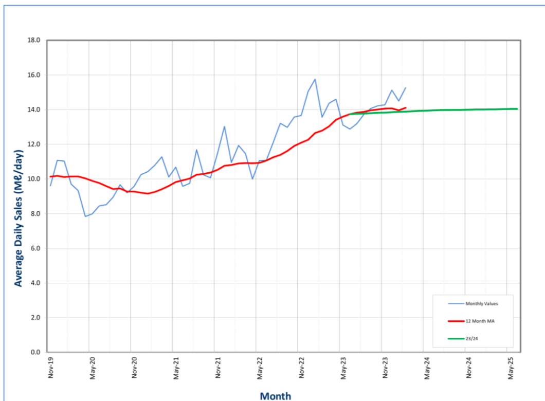
Figure 3.7 Siza Water Total Sales Volumes - Annual short-term forecast.
