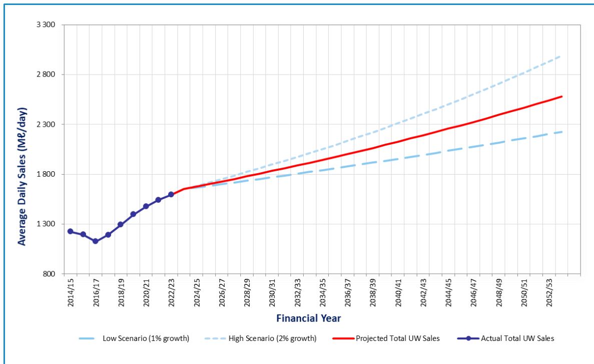
Figure 3.12 uMngeni-uThukela Water Long-Term Bulk Water Sales Forecast.
