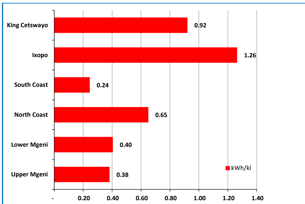
Figure 5.2 Energy requirement to supply water in uMngeni-uThukela Water Systems 2022/23 (kWh/kl).
