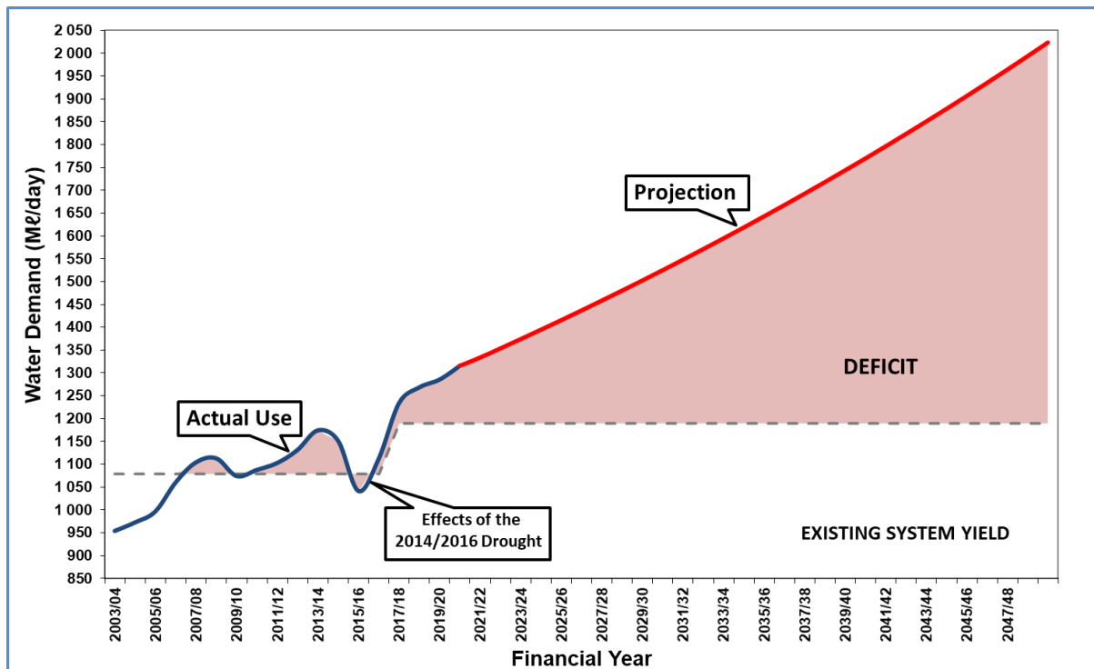
Figure 2.72 uMngeni System - Existing Water Balance
