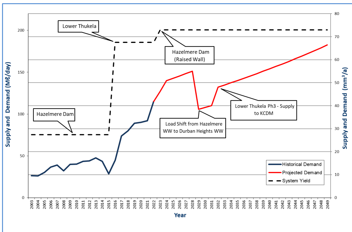
Figure 2.73 North Coast Supply System – Existing Water Balance
