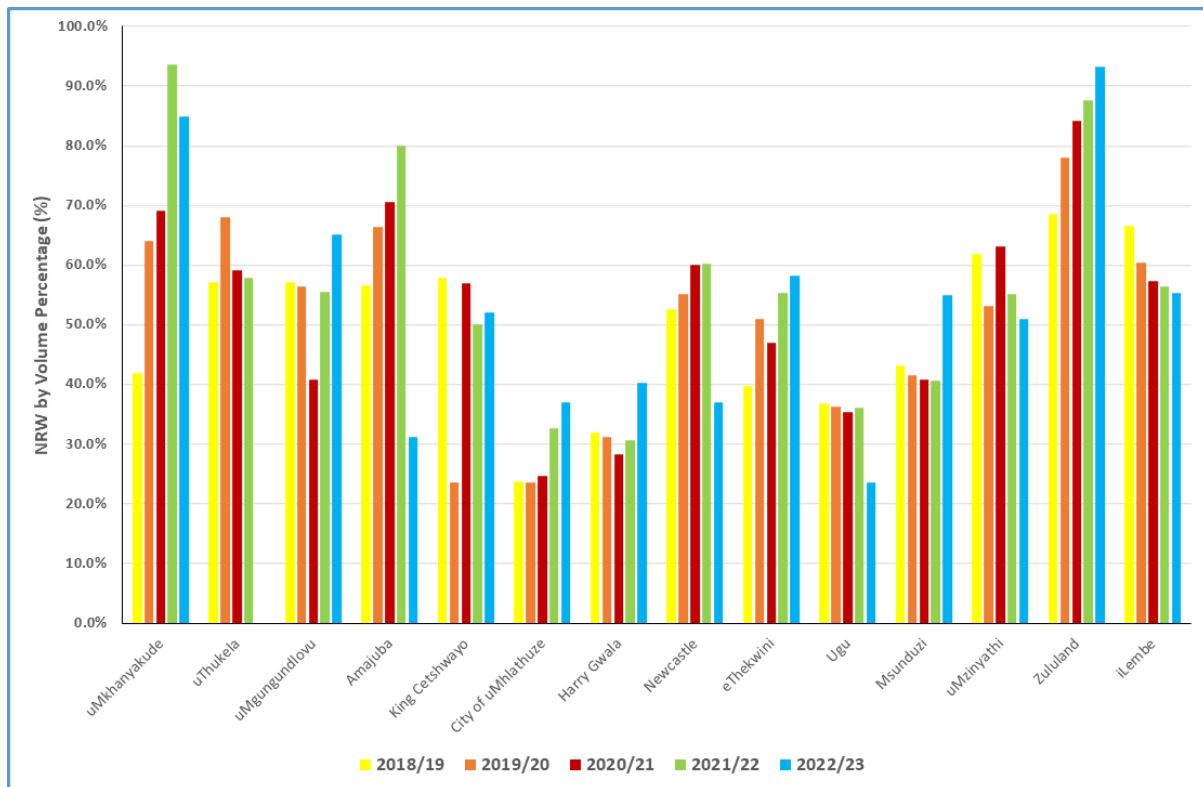
Figure 4.1 Historical Water Balance Analysis (2018/2019 to 2022/2023) (uMngeni-uThukela Water 2023).
