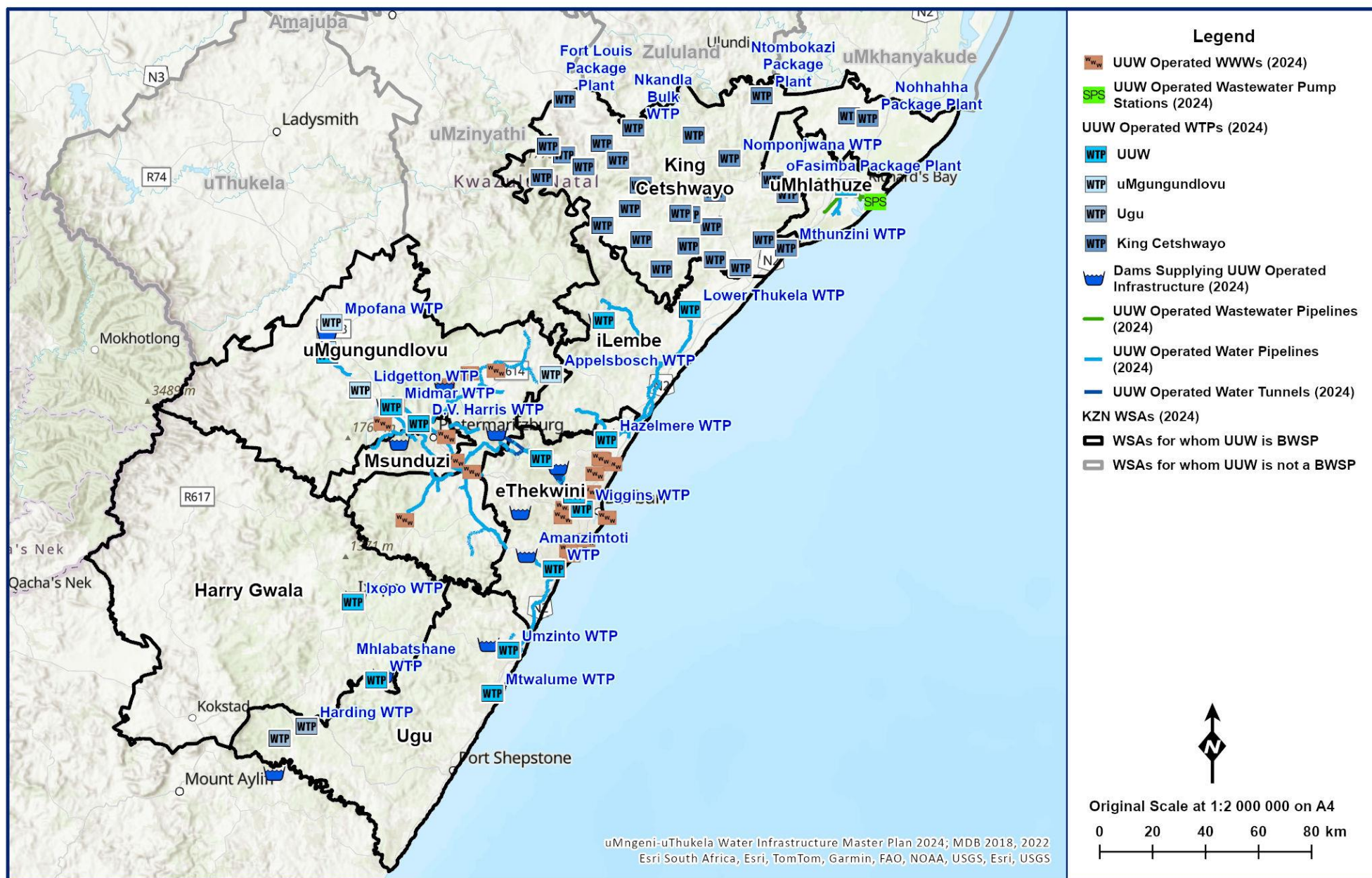
Figure 1.4 uMngeni-uThukela Water's infrastructure (January 2023 – present).
