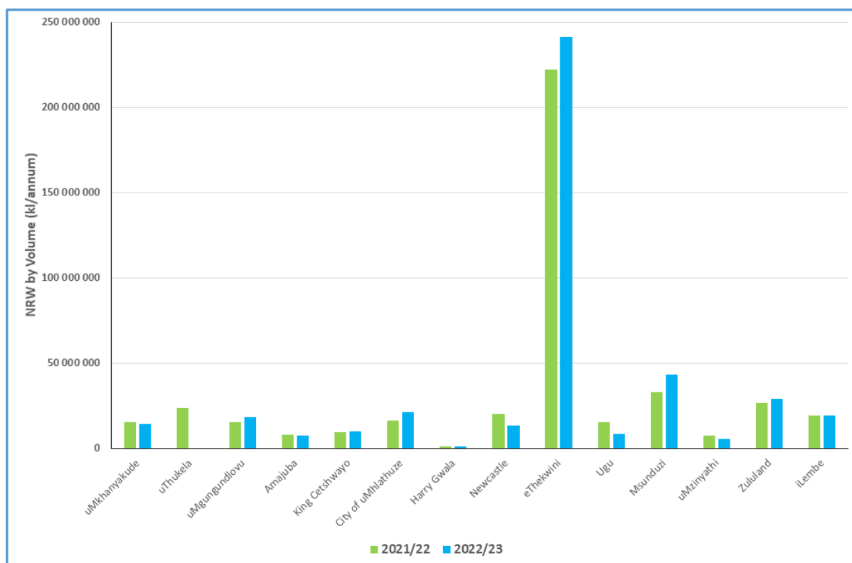
Figure 4.5 WSA Non-Revenue Water by Volume (2021/2022 vs 2022/2023) (uMngeni-uThukela Water 2023).
