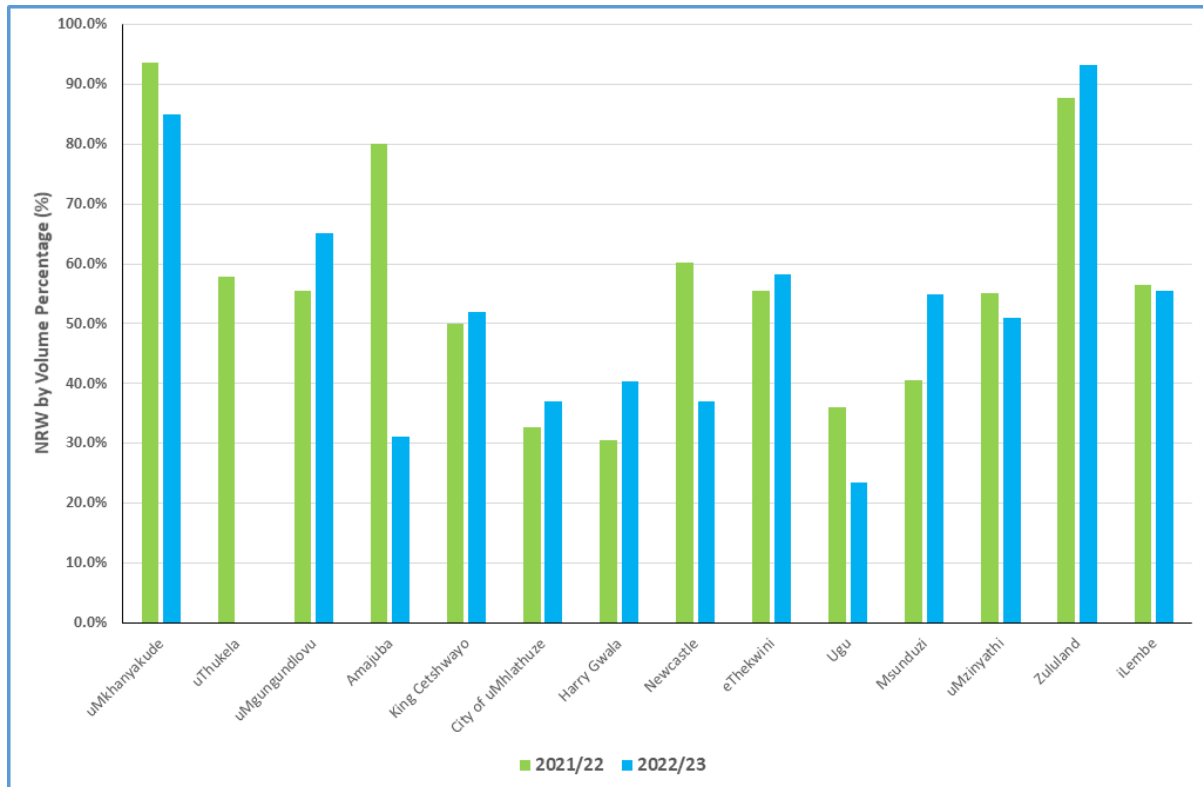
Figure 4.6 WSA Non-Revenue Water by Percentage (2021/2022 vs 2022/2023) (uMngeni-uThukela Water 2023).
