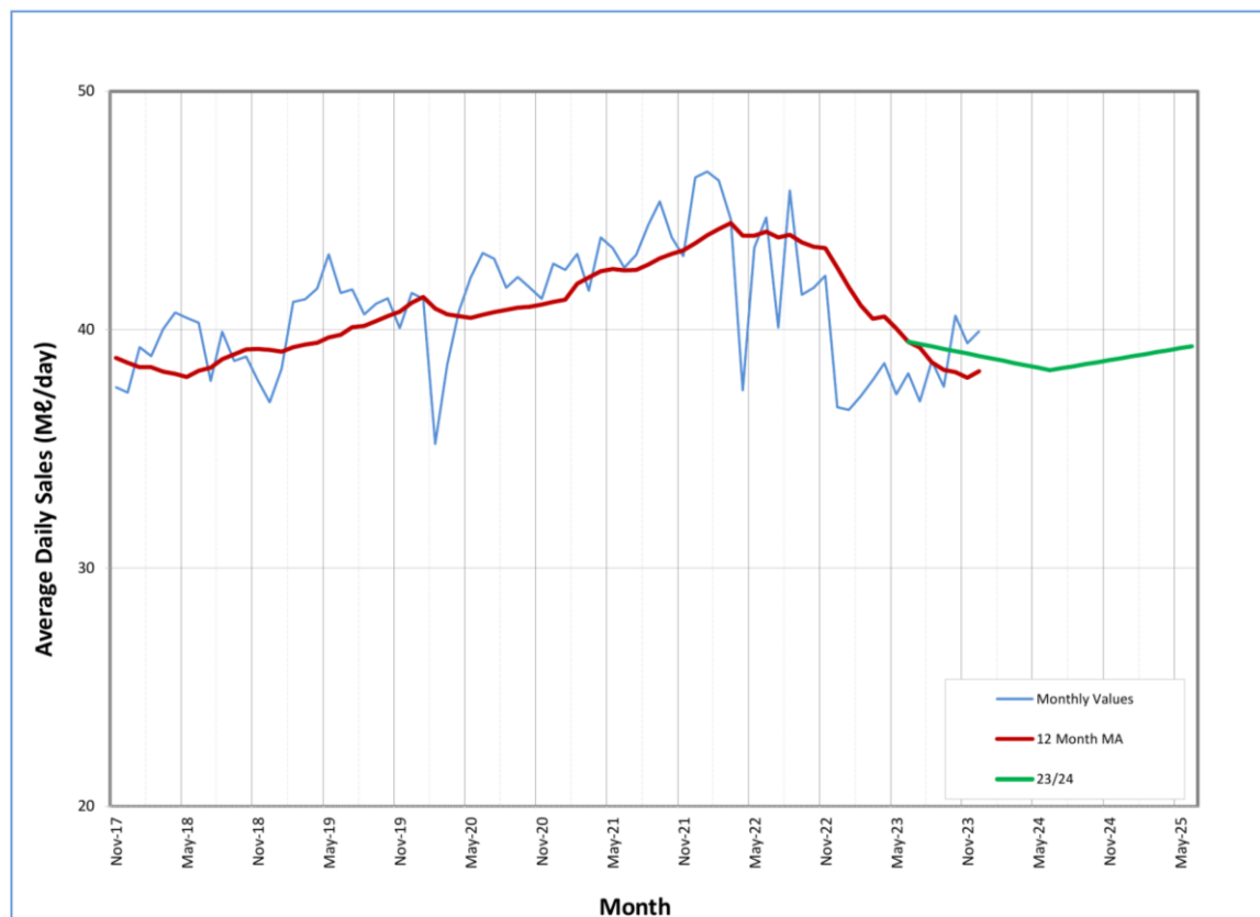
Figure 3.9 Ugu District Municipality Total Sales Volumes - Annual short-term forecast.
