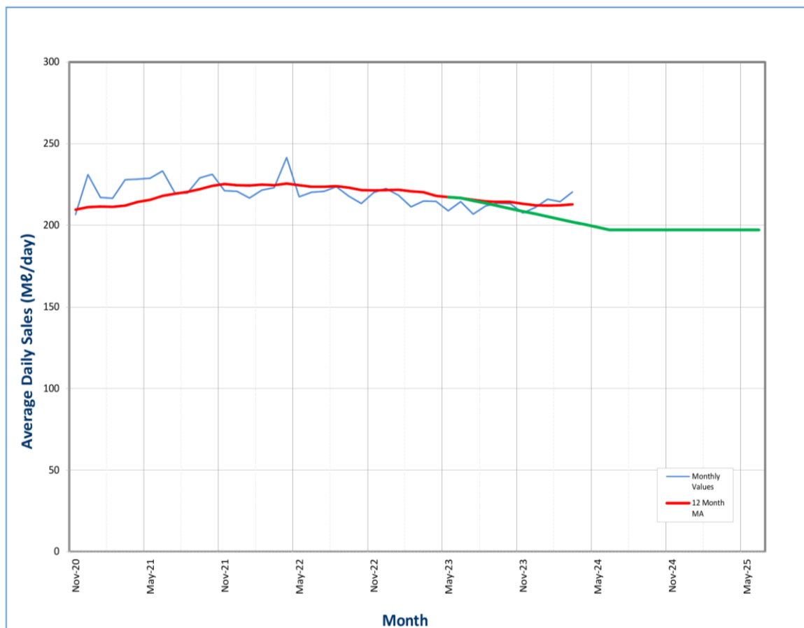
Figure 3.5 Msunduzi Municipality Total Sales Volumes - Annual short-term forecast.
