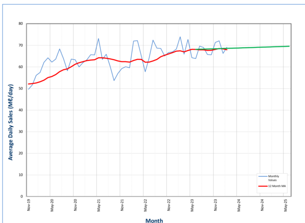
Figure 3.8 iLembe District Municipality Total Sales Volumes - Annual short-term forecast.
