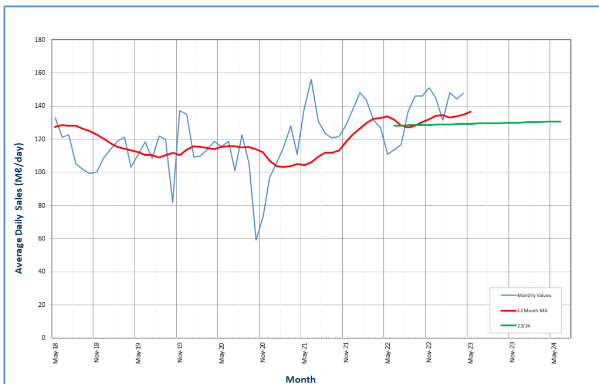
Figure 3.12 uMhlathuze Local Municipality and Industrial Volumes – Annual Short Term Forecast.
