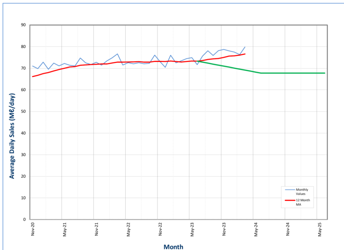
Figure 3.6 uMgungundlovu District Municipality Total Sales Volumes - Annual short-term forecast.
