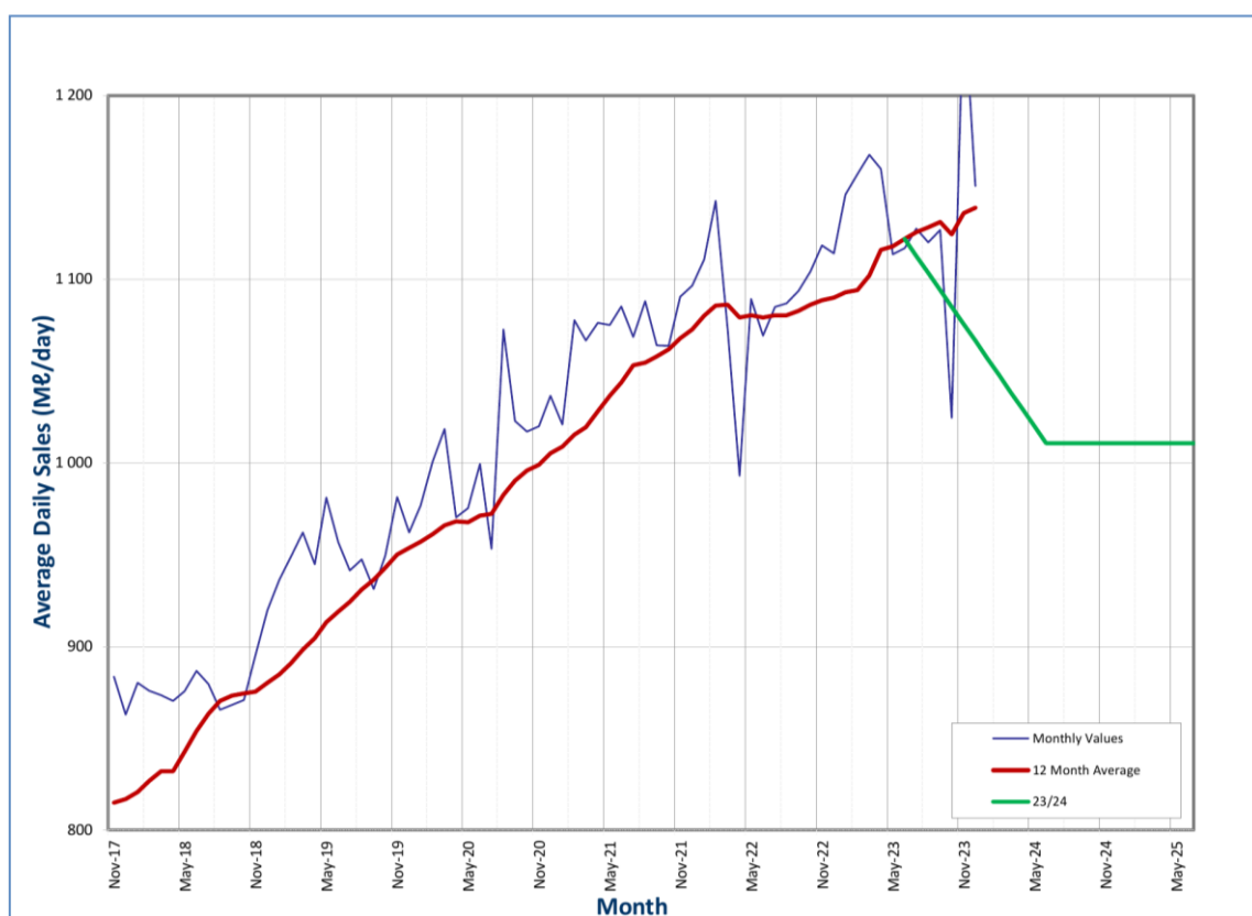
Figure 3.4 eThekweni Municipality Total Volumes - Annual short-term forecast.
