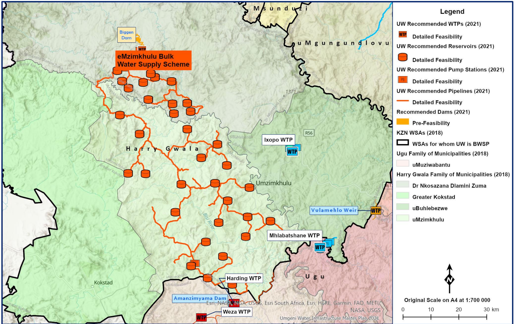
Figure 8.9 Proposed uMzimkhulu Bulk Water Supply Scheme.
