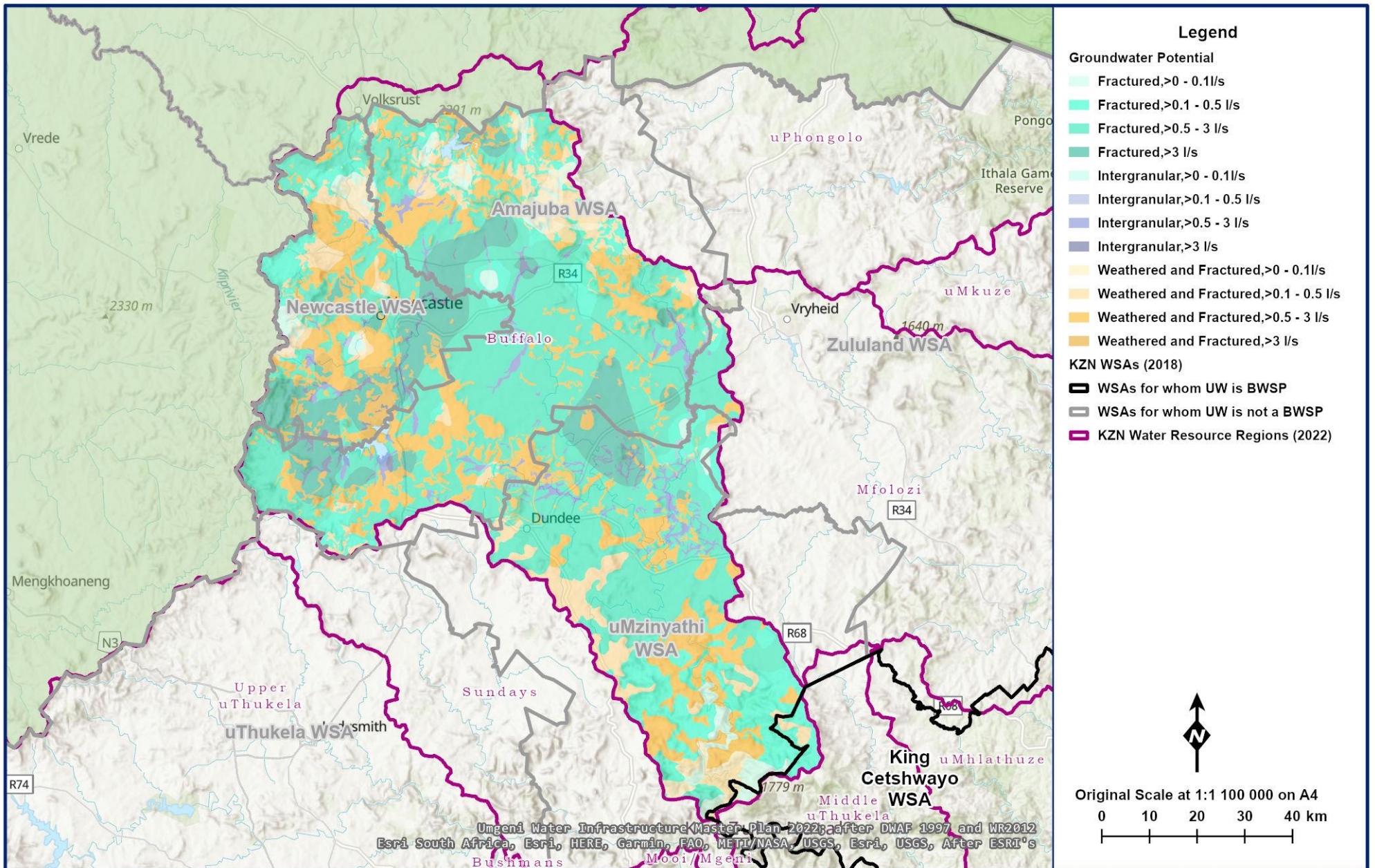
Figure 14.6 Groundwater potential in the Buffalo Region (MDB 2020; Umgeni Water 2022; after DWAF 1997 and WR2012).
