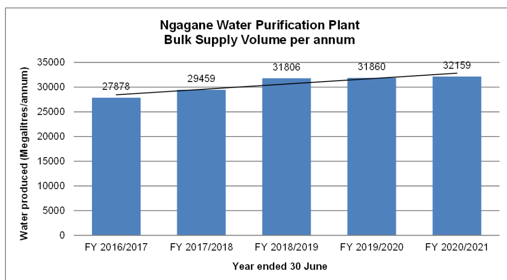
Figure 14.47 Water Demand of Ngagane WTP till 2021 (uThukela Water 2022)
