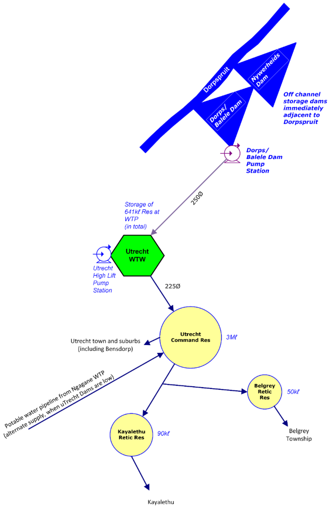
Figure 14.39 Utrecht WTP Supply Schematic (not to scale; Amajuba DM Water bulk infrastructure)
