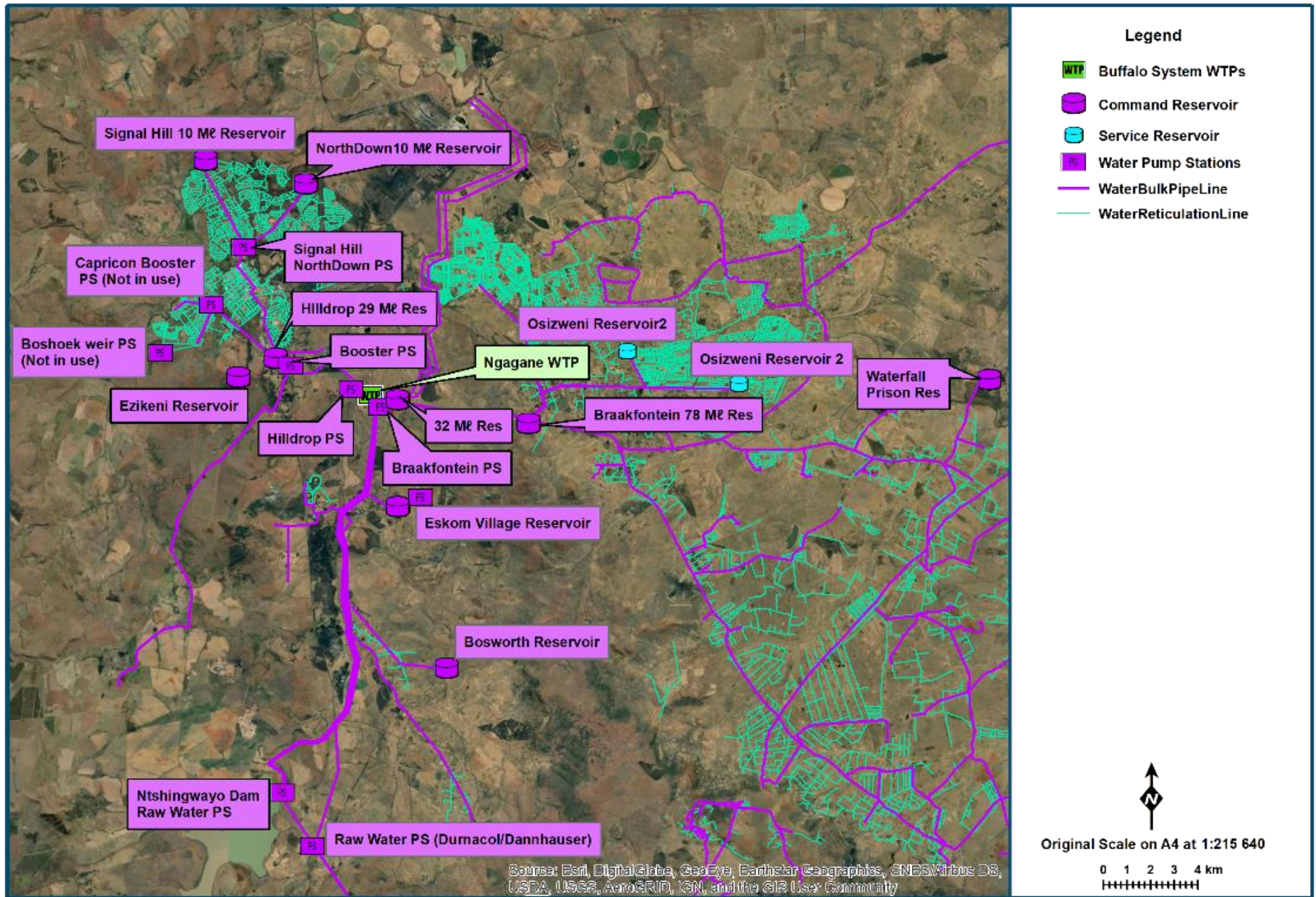
Figure 14.22 Newcastle Supply System Layout (Ngagane WTP System) (NGI 2014; Umgeni Water 2020)
