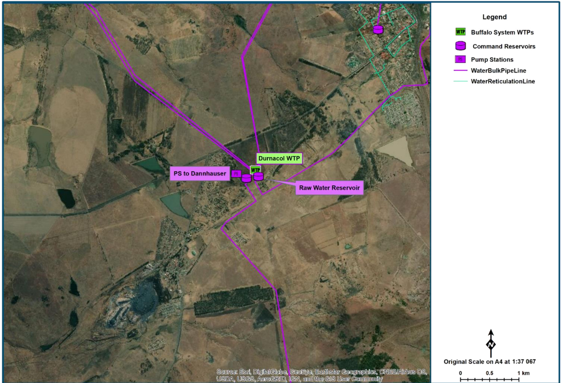
Figure 14.36 Durnacol Supply System Layout (Durnacol WTP System) (NGI 2014; Umgeni Water 2020)
