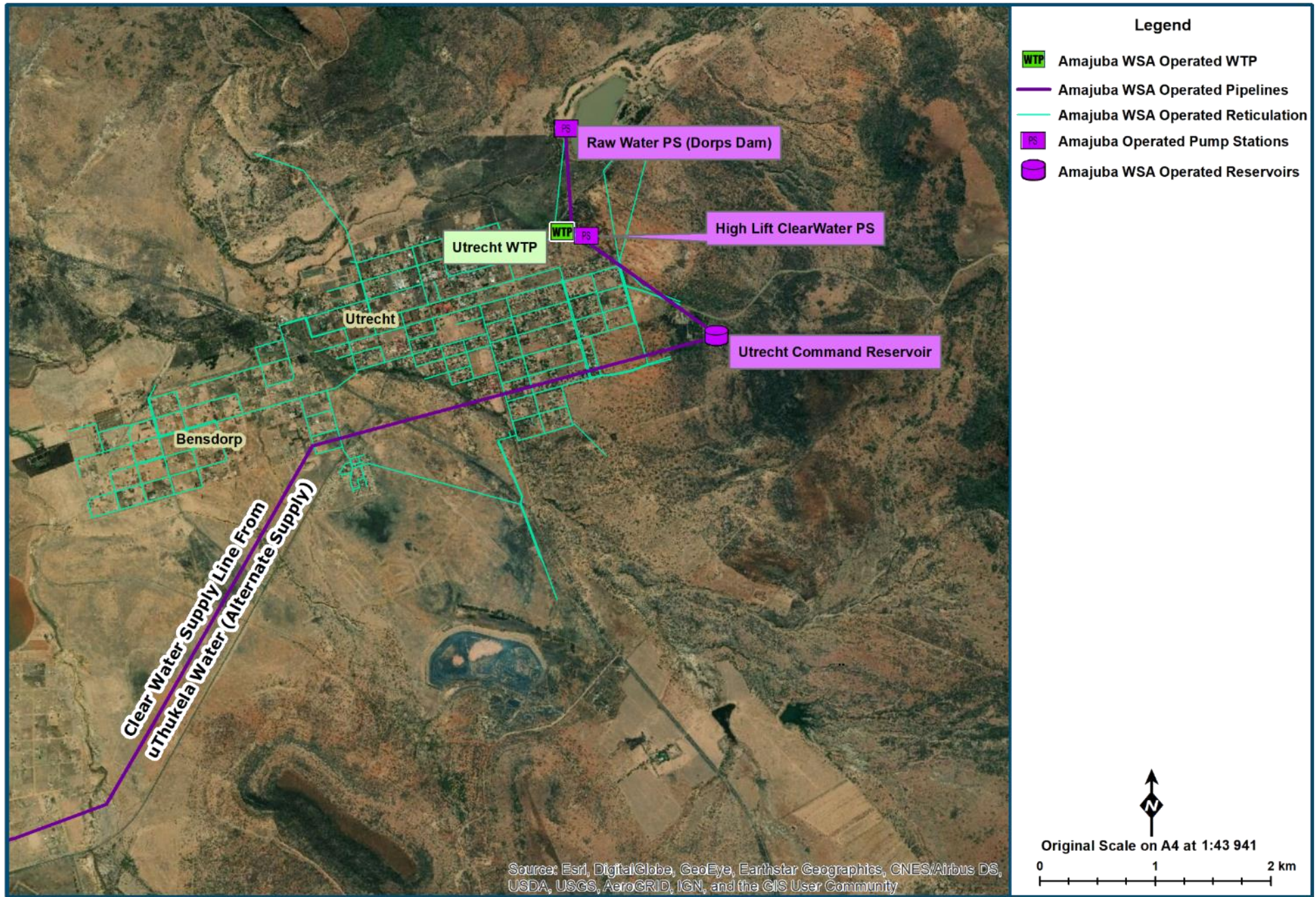
Figure 14.40 Utrecht Supply System Layout (Utrecht WTP System) (NGI 2014; Umgeni Water 2020)
