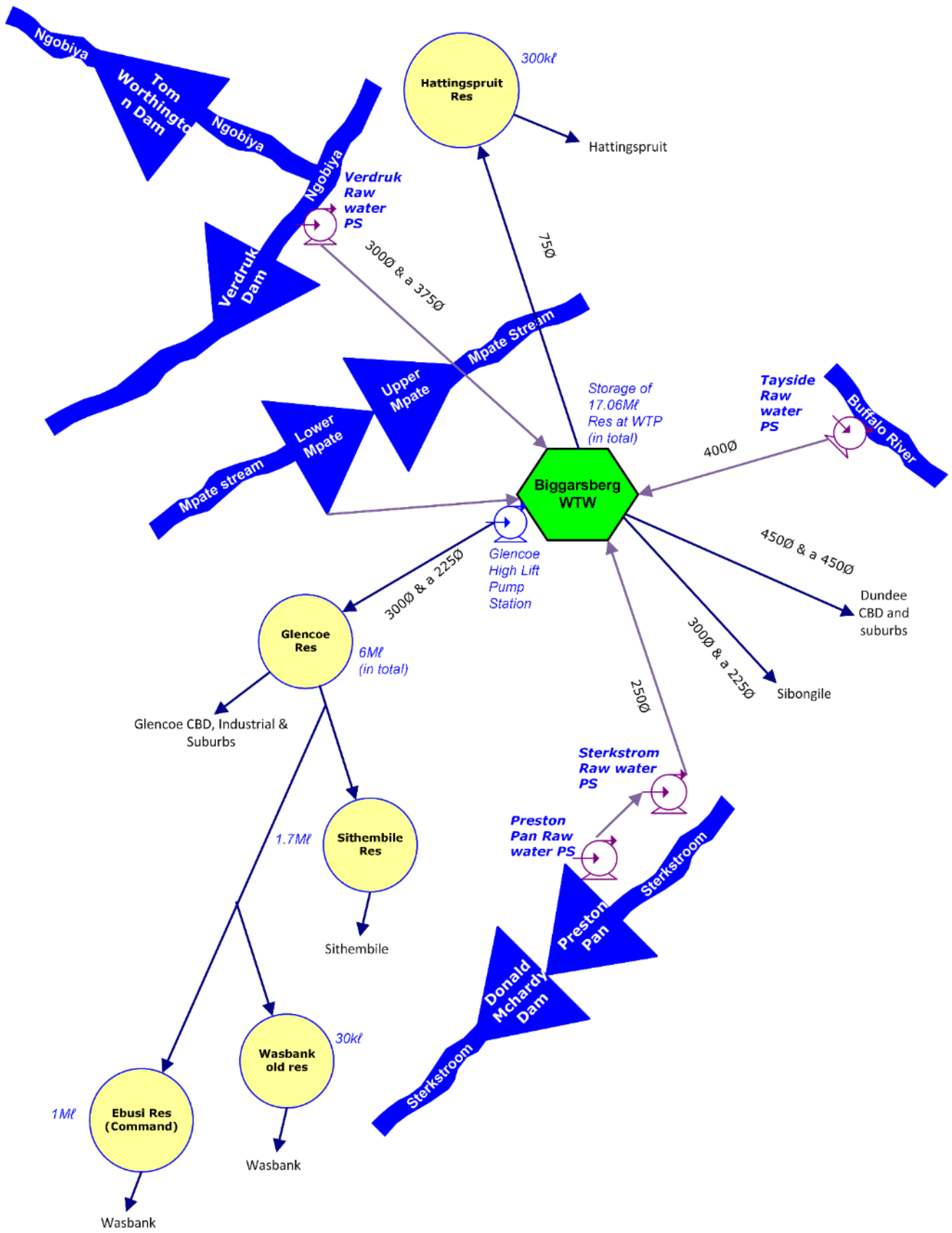
Figure 14.26 Biggarsberg WTP Supply Schematic (not to scale; uMzinyathi bulk infrastructure)
