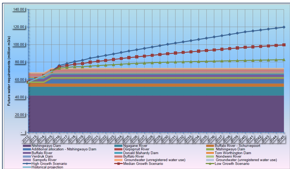
Figure 14.53 Comparison of the future water requirements and the available water supplies in the Buffalo catchment (DWS 2016).
