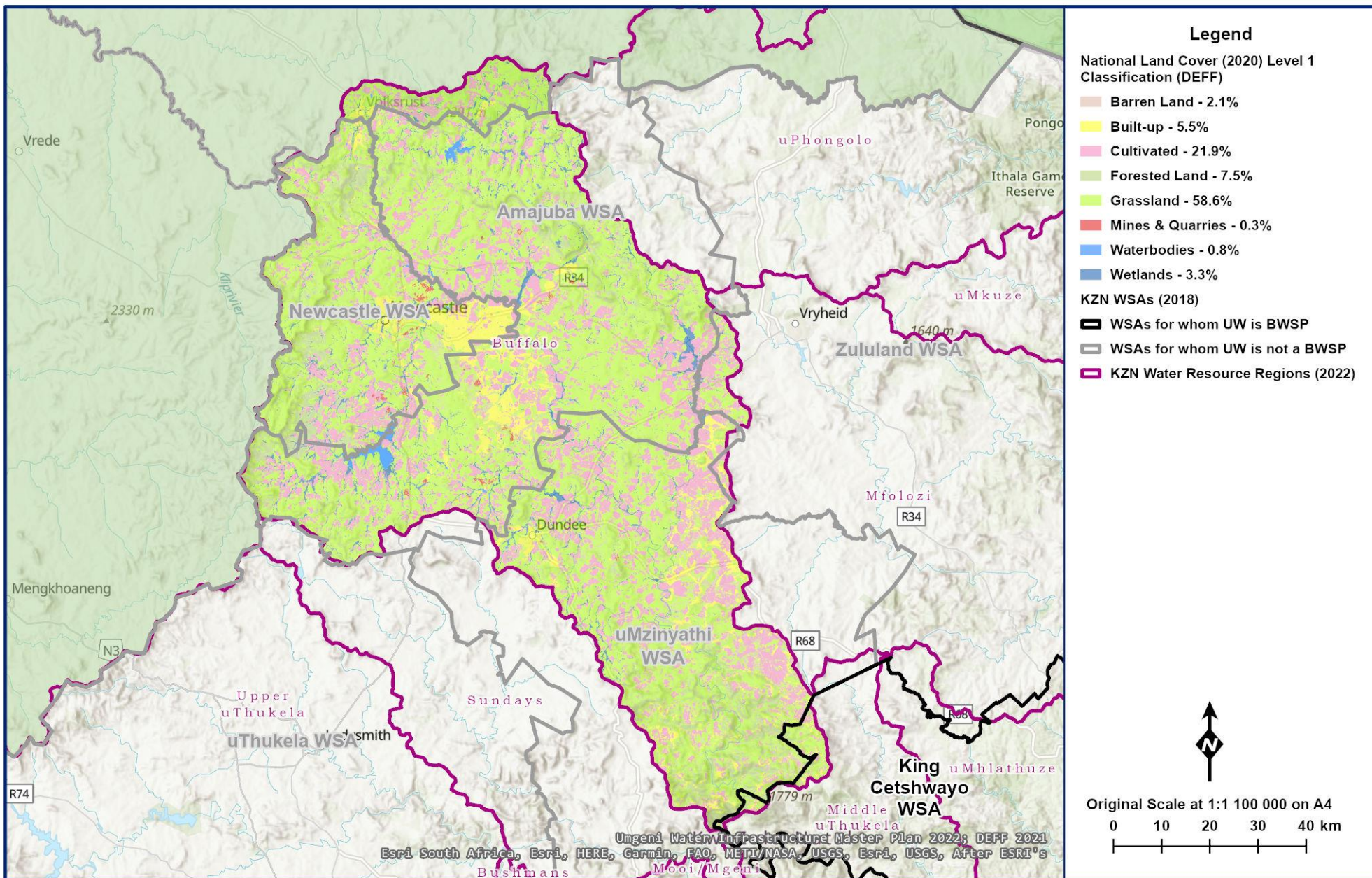
Figure 14.5 Buffalo System Land Cover Map (DEFF 2020; MDB 2020; Umgeni Water 2022; WR2012).
