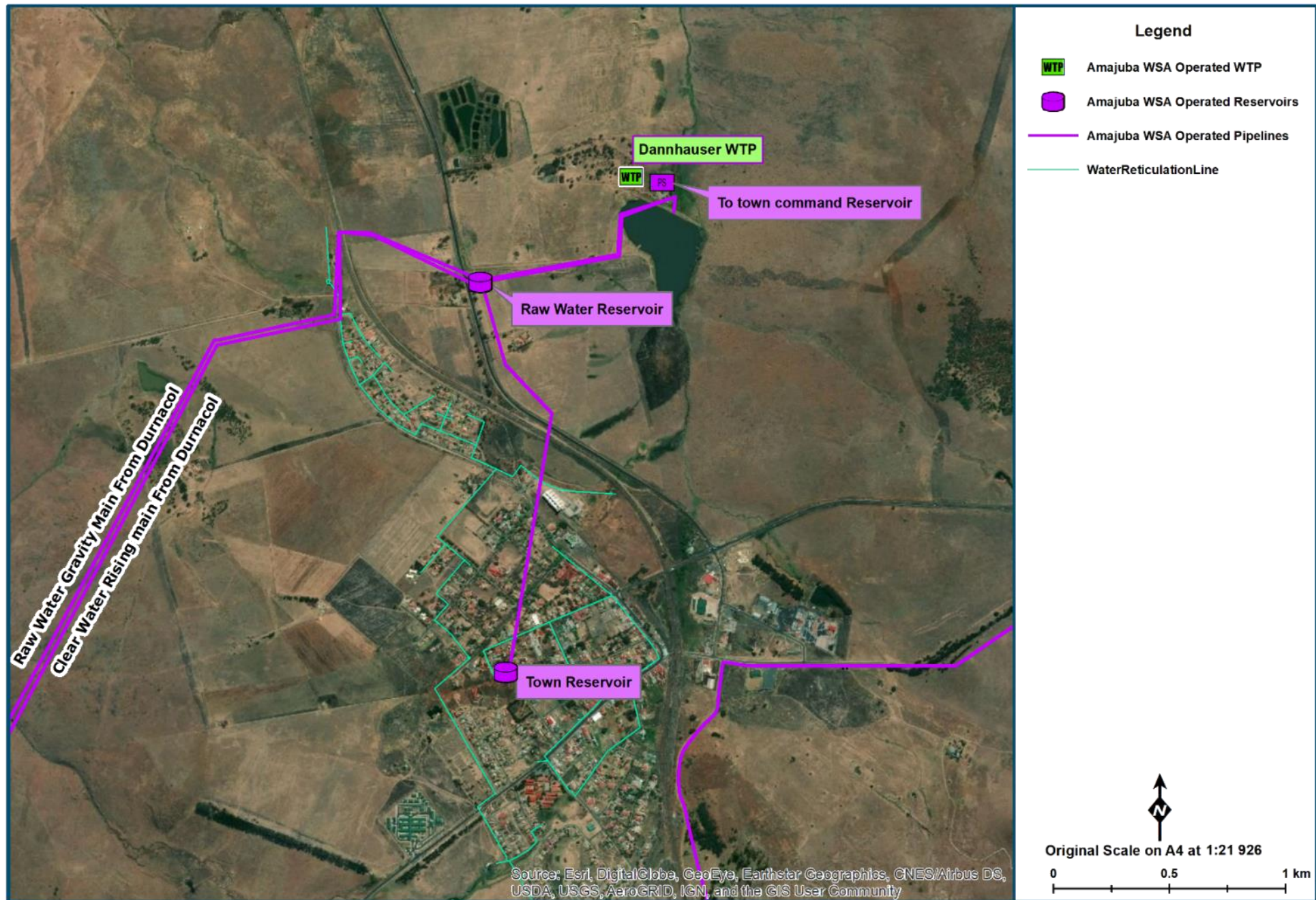
Figure 14.33 Dannhauser Supply System Layout (Dannhauser WTP System) (NGI 2014; Umgeni Water 2020)
