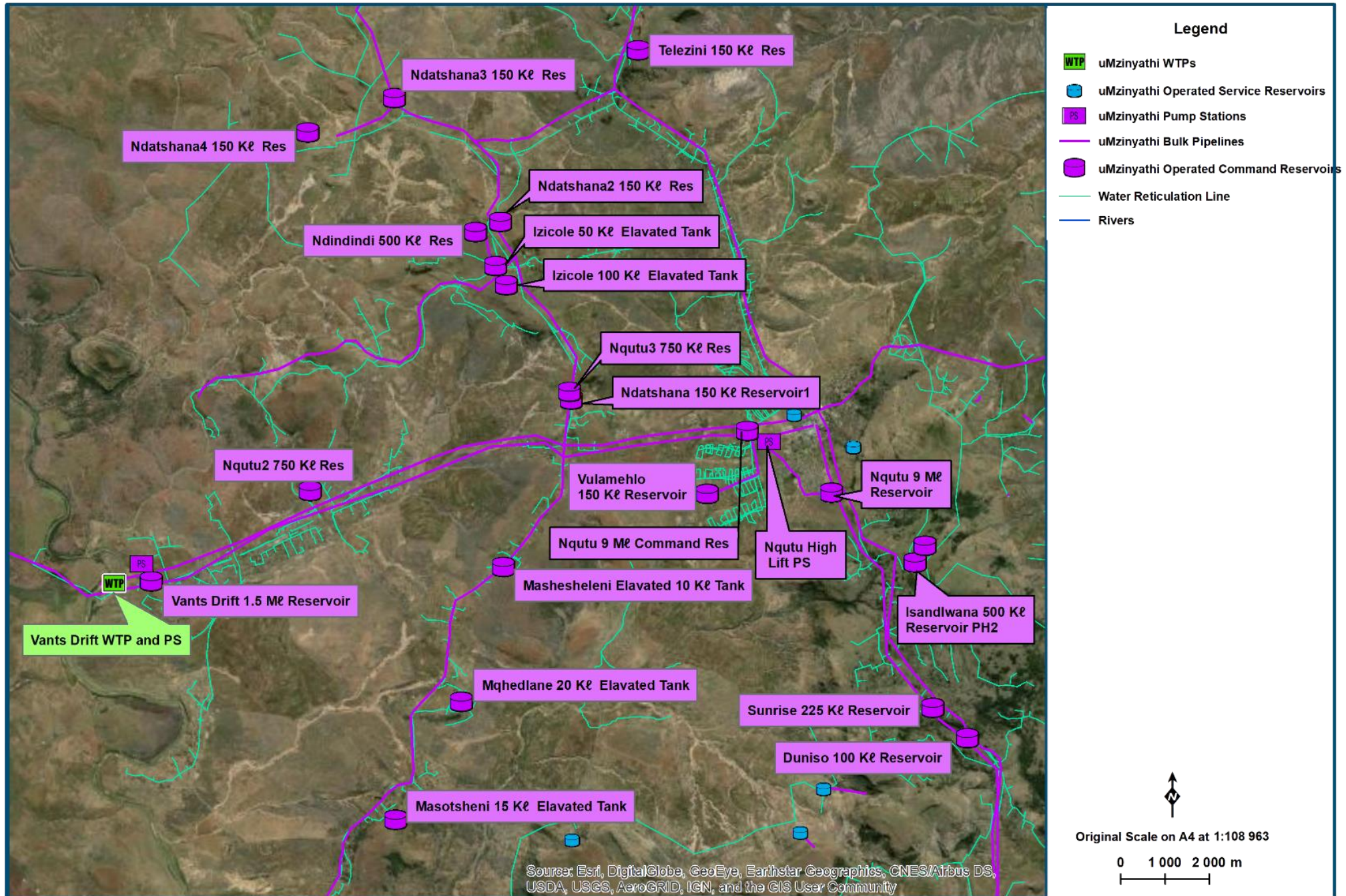
Figure 14.29 Nqutu Supply System Layout (Vants Drift WTP System) (NGI 2014; Umgeni Water 2020)
