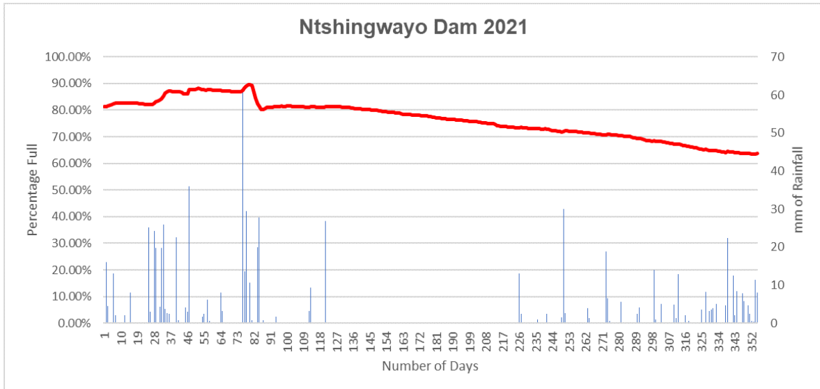
Figure 14.49 Ntshingwayo Dam Level and rainfall figures from Jan 2021 to Dec 2021 (DWS 2022)
