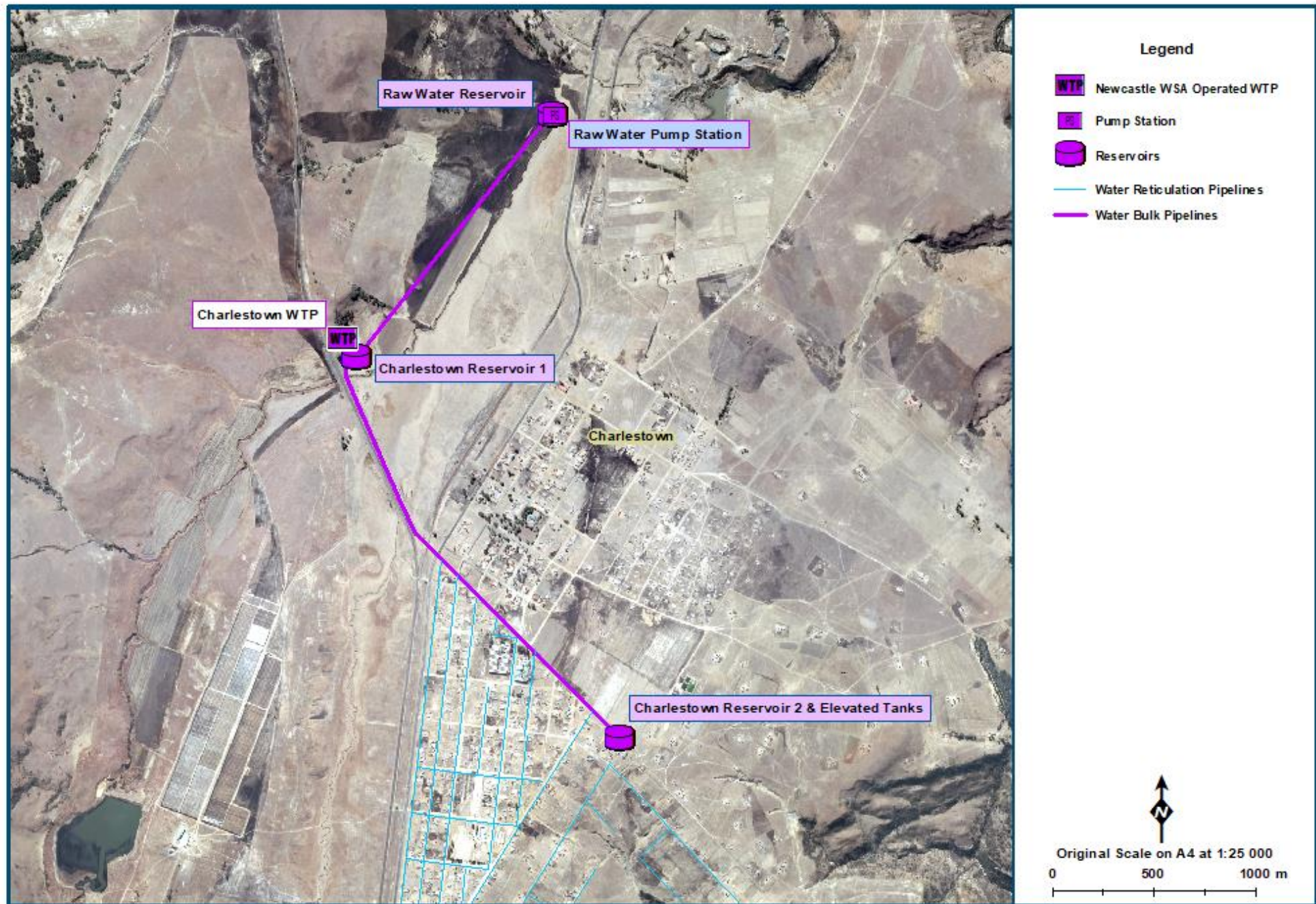
Figure 14.45 Charlestown Supply System Layout (Charlestown WTP System) (NGI 2014; Umgeni Water 2020)
