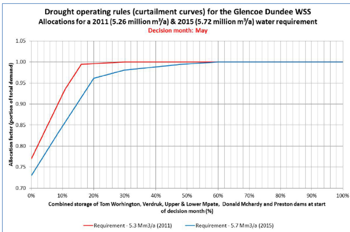
Figure 14.19 Drought operating rules for the Glencoe and Dundee WSS (May decision month).
