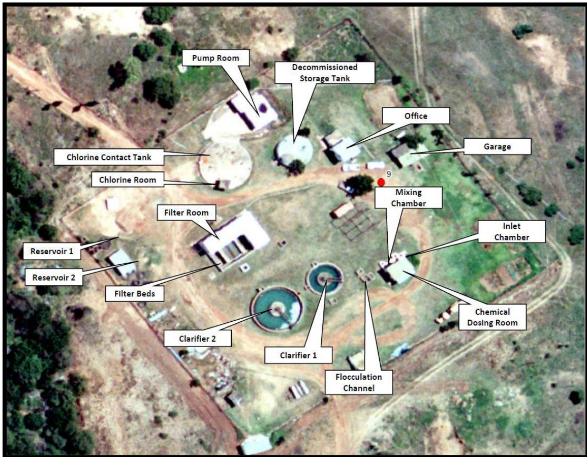
Figure 14.38 Aerial Image of Utrecht Water Treatment Plant (ADM O&M Manual May 2016)
